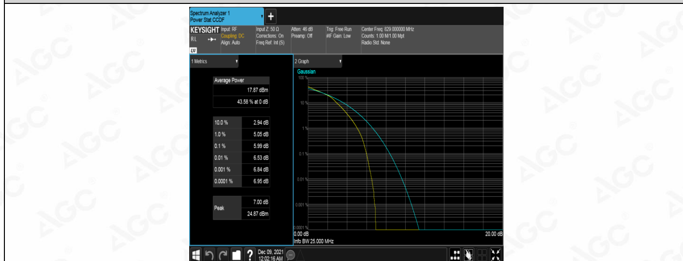
Band5-10MHz-16QAM-20525-1RB#0
