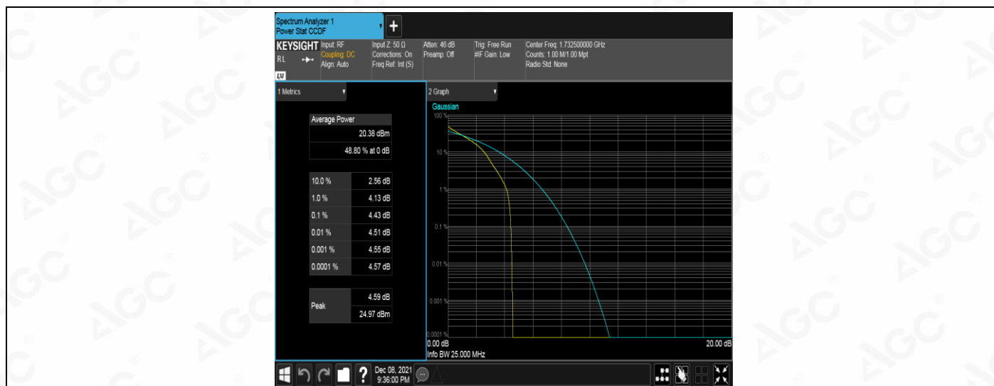
Band4-1.4MHz-QPSK-20175-6RB#0
