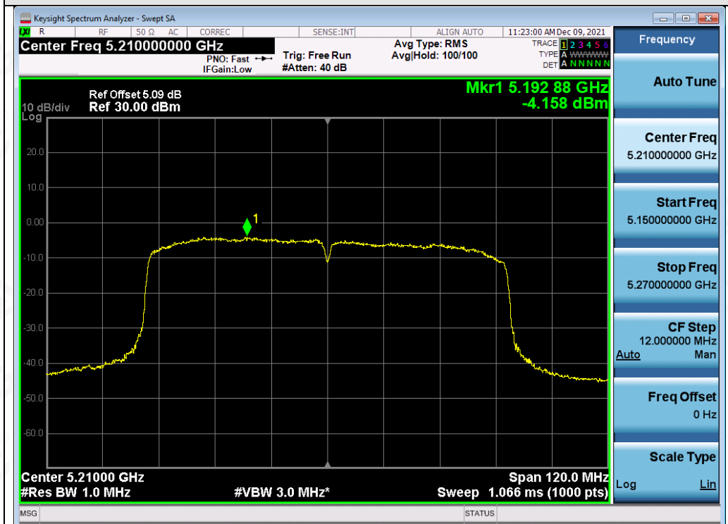
Test_Graph_802.11ac80_ANT1_5210_MCS9_PSD
