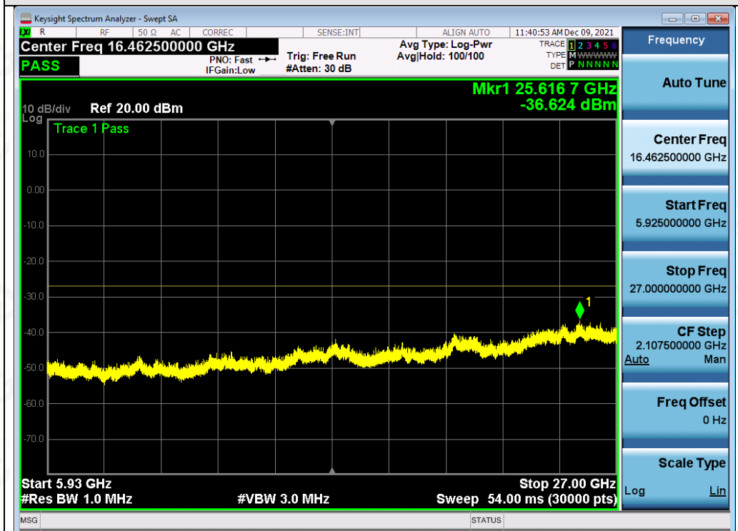
Test_Graph_802.11n40_ANT1_5755_MCS0_Frequency Band4
