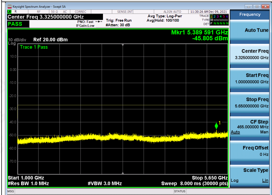
Test_Graph_802.11a_ANT1_5745_6Mbps_Frequency Band2
