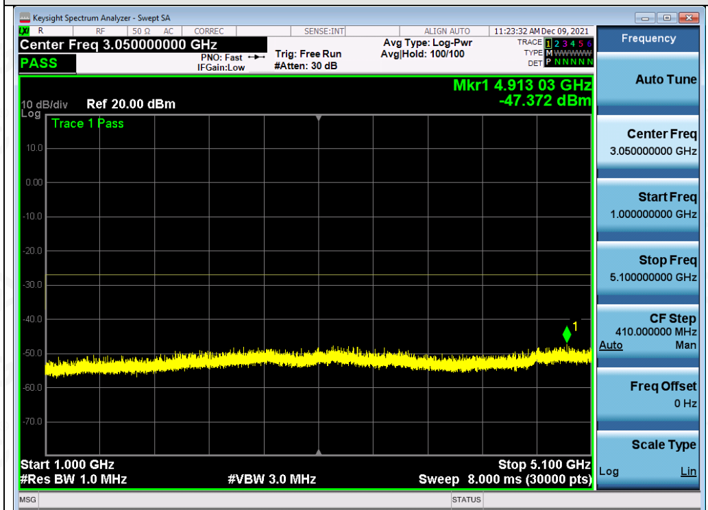
Test_Graph_802.11ac80_ANT1_5210_MCS9_Frequency Band 2
