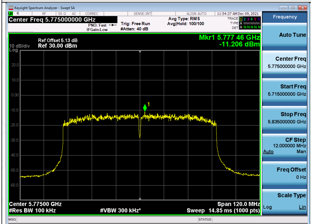
Test_Graph_802.11ac80_ANT1_5775_MCS9_PSD
