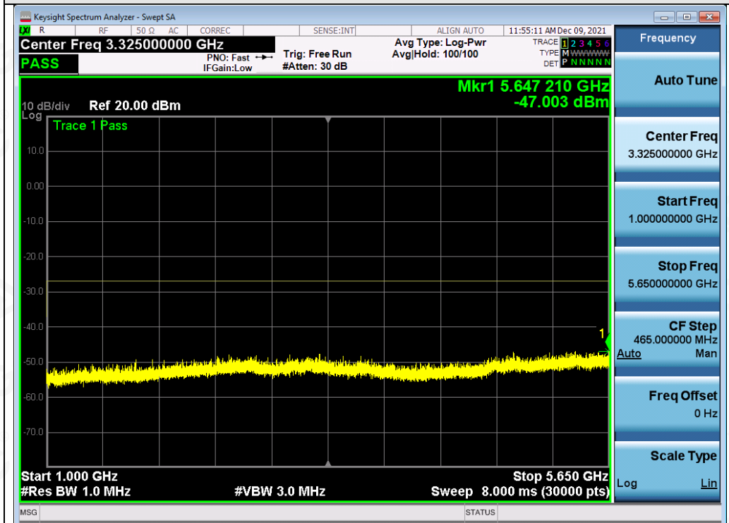
Test_Graph_802.11ac80_ANT1_5775_MCS9_Frequency Band2
