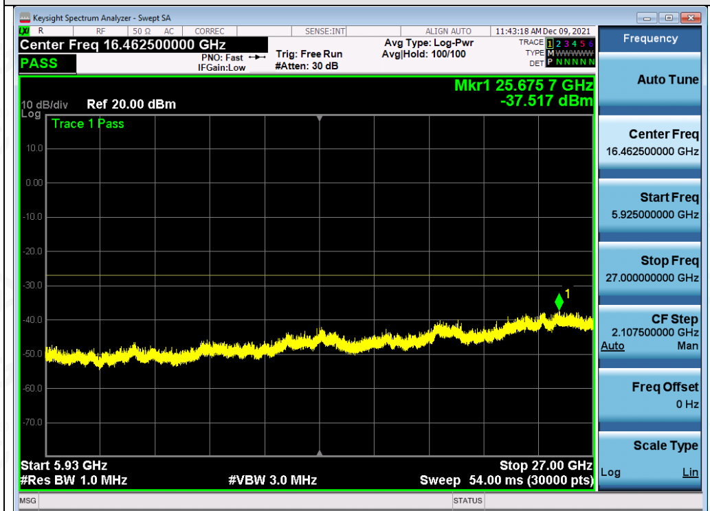
Test_Graph_802.11n40_ANT1_5795_MCS0_Frequency Band4
