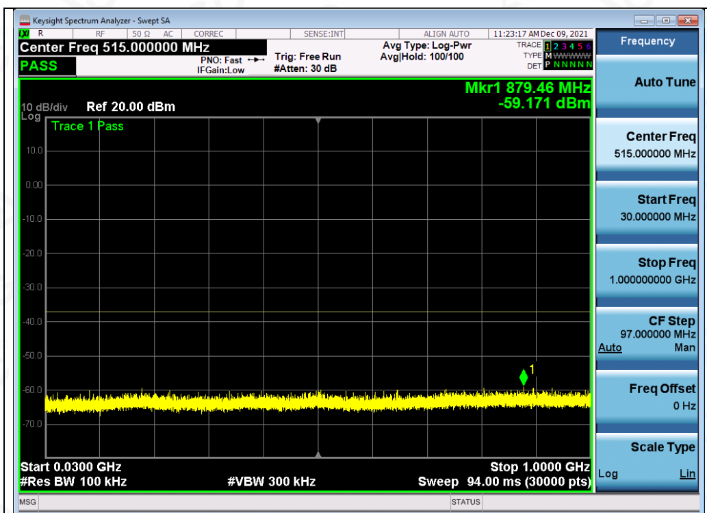
Test_Graph_802.11ac80_ANT1_5210_MCS9_Frequency Band 1
