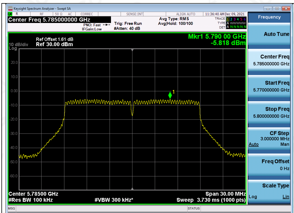
Test_Graph_802.11n20_ANT1_5785_MCS0_PSD
