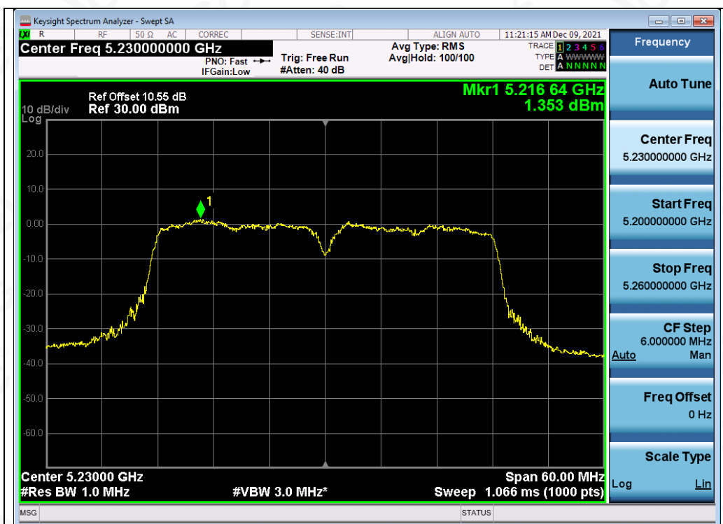
Test_Graph_802.11ac40_ANT1_5230_MCS9_PSD
