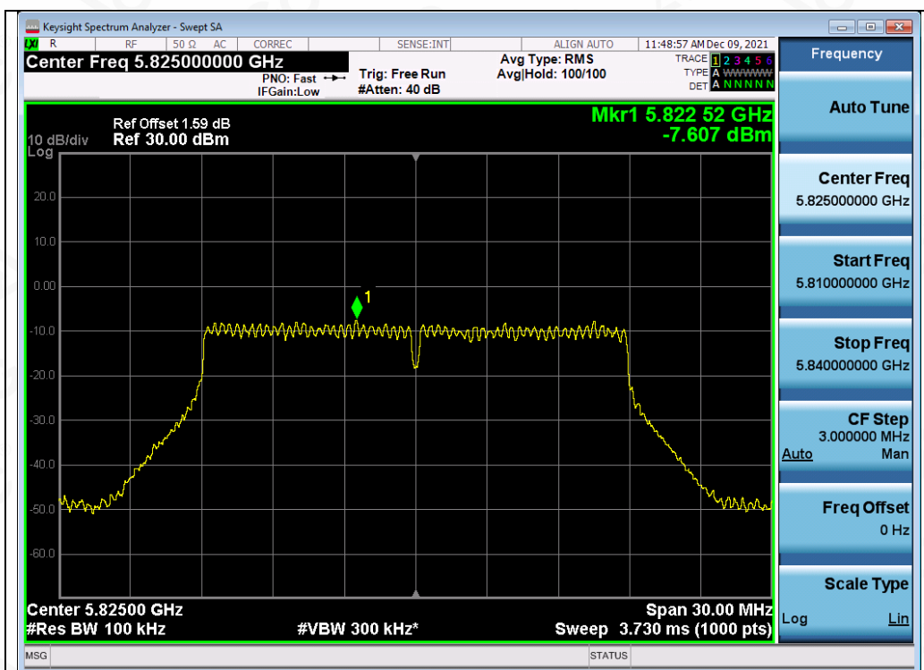
Test_Graph_802.11ac20_ANT1_5825_MCS9_PSD
