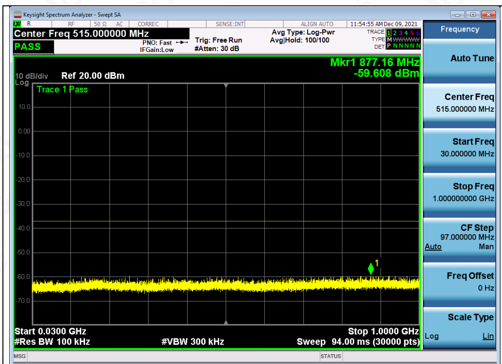
Test_Graph_802.11ac80_ANT1_5775_MCS9_Frequency Band1
