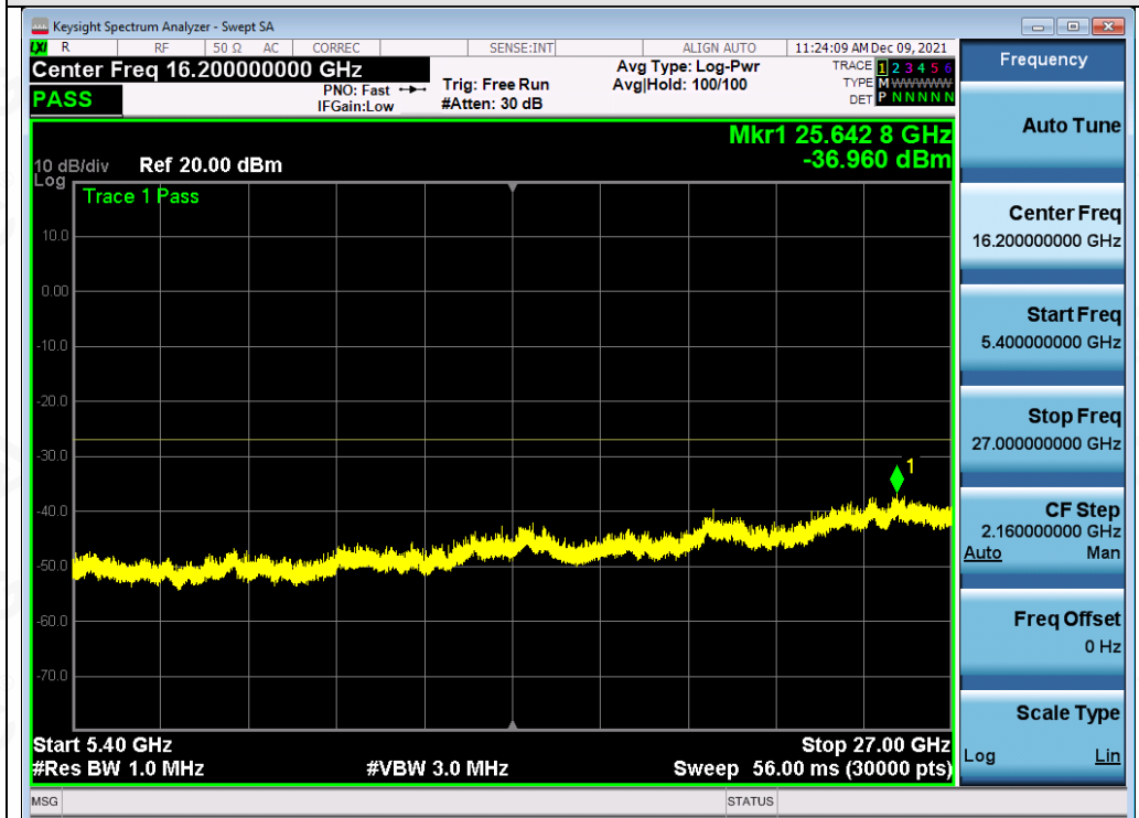
Test_Graph_802.11ac80_ANT1_5210_MCS9_Frequency Band 4
