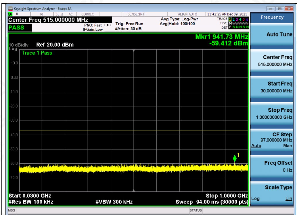
Test_Graph_802.11n40_ANT1_5795_MCS0_Frequency Band1
