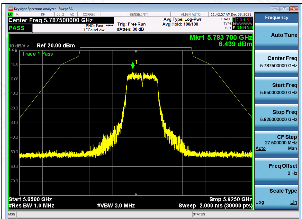
Test_Graph_802.11n40_ANT1_5795_MCS0_Frequency Band3
