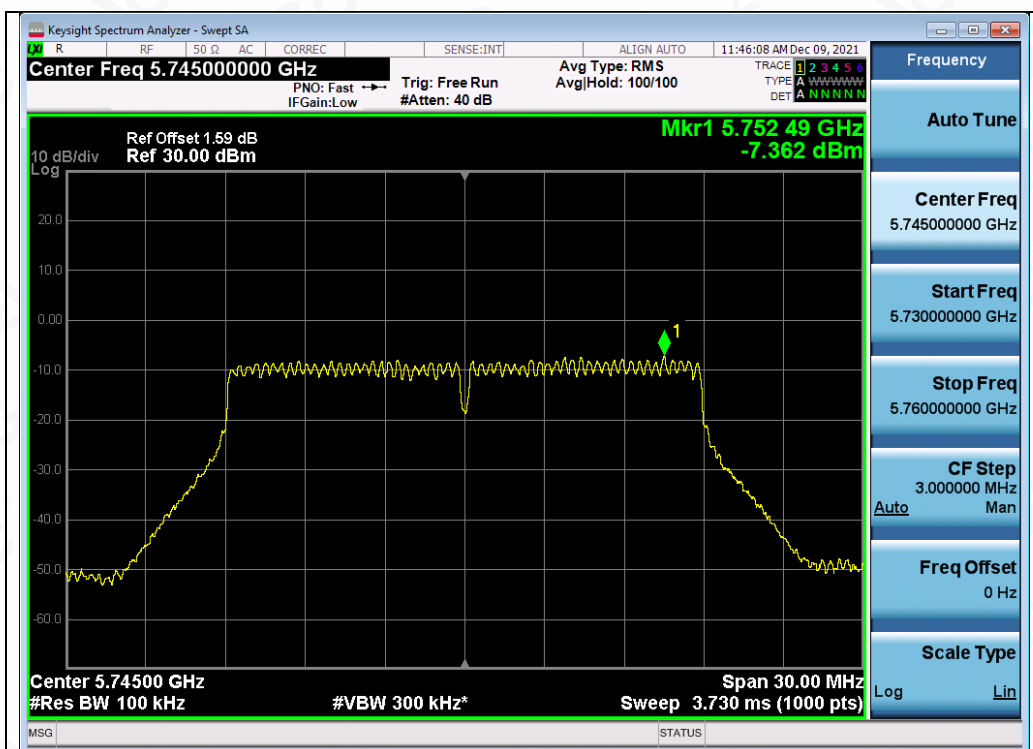
Test_Graph_802.11ac20_ANT1_5745_MCS0_PSD
