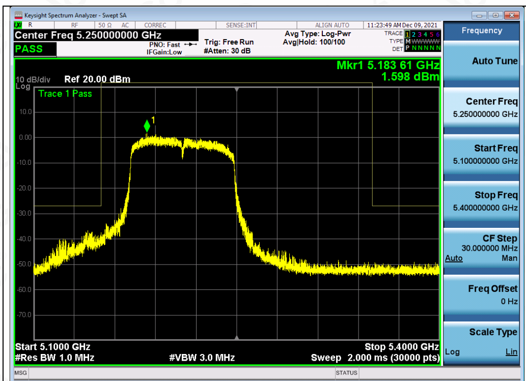
Test_Graph_802.11ac80_ANT1_5210_MCS9_Frequency Band 3
