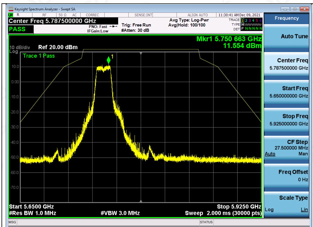
Test_Graph_802.11a_ANT1_5745_6Mbps_Frequency Band3
