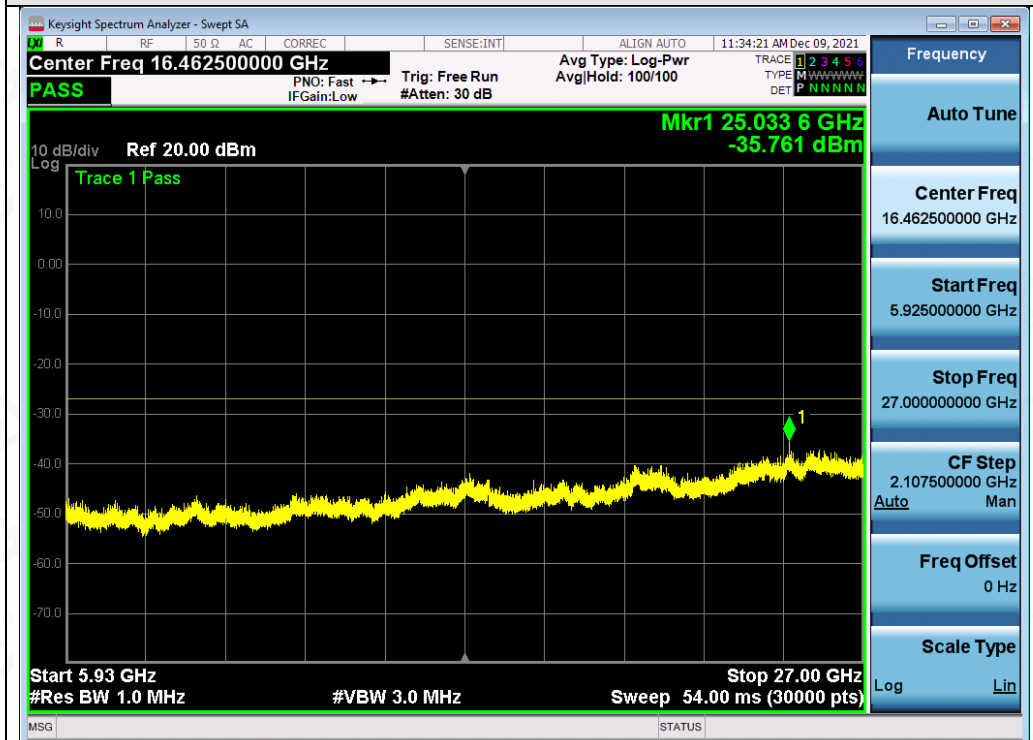
Test_Graph_802.11a_ANT1_5825_6Mbps_Frequency Band4
