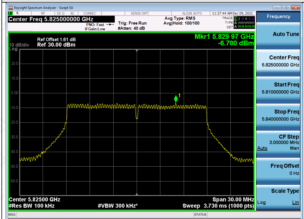
Test_Graph_802.11n20_ANT1_5825_MCS0_PSD
