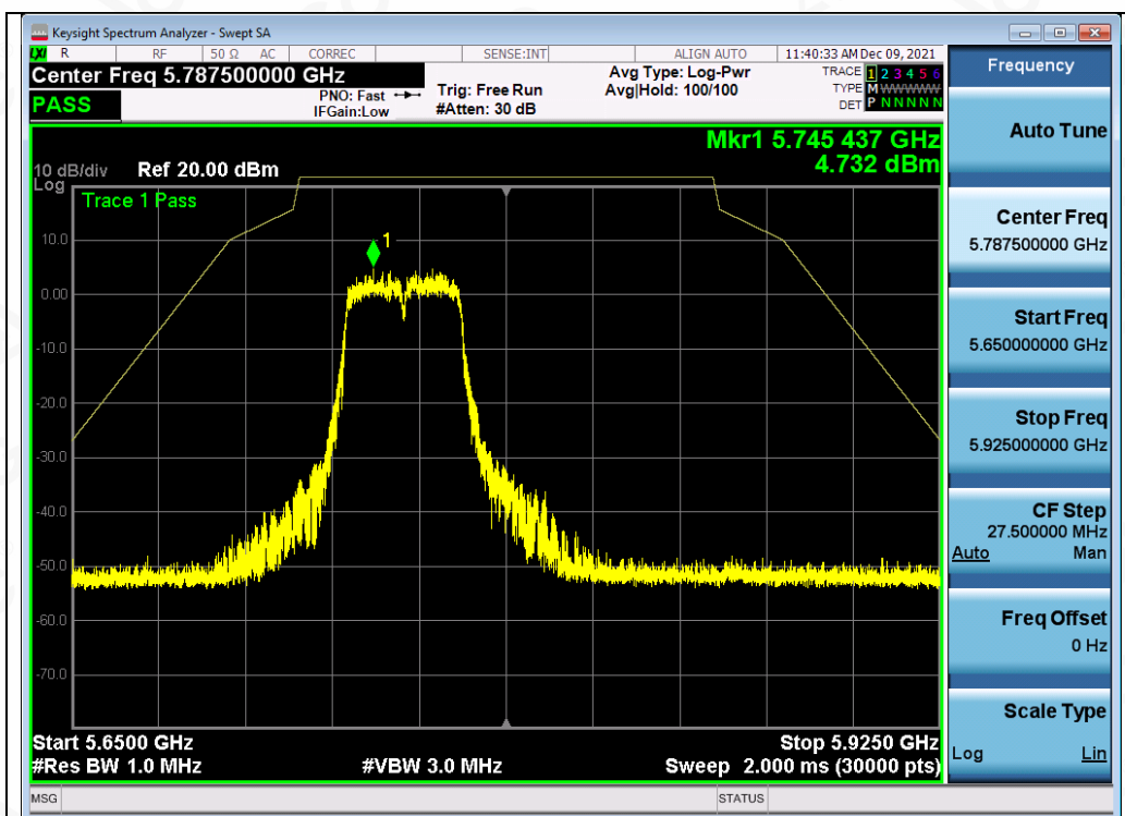
Test_Graph_802.11n40_ANT1_5755_MCS0_Frequency Band3
