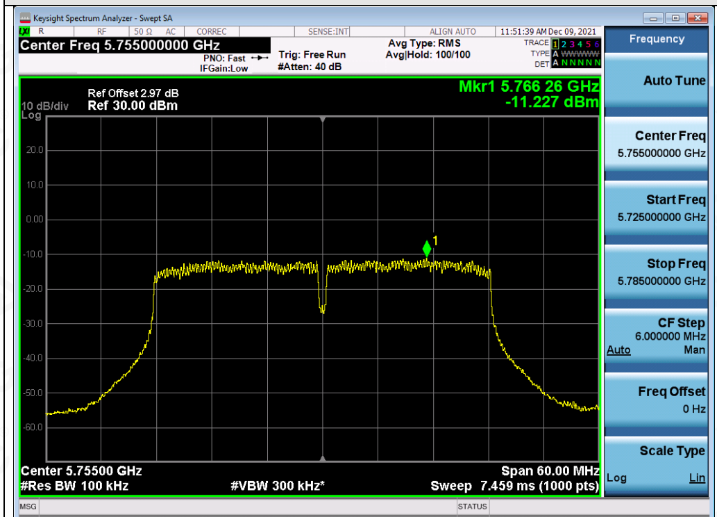
Test_Graph_802.11ac40_ANT1_5755_MCS9_PSD
