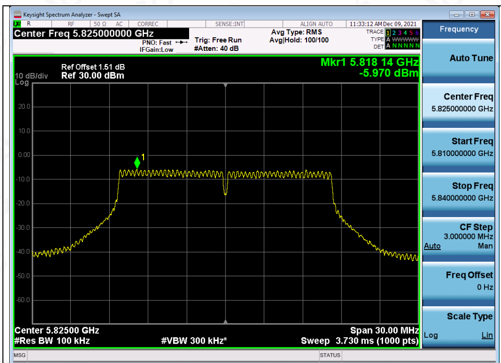
Test_Graph_802.11a_ANT1_5825_6Mbps_PSD
