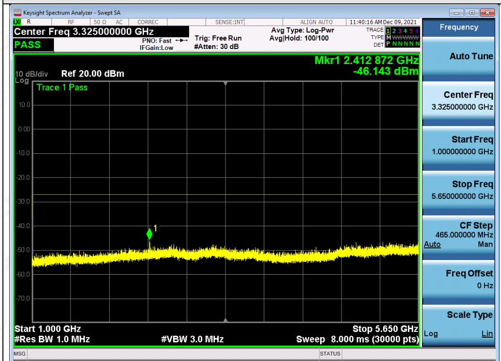
Test_Graph_802.11n40_ANT1_5755_MCS0_Frequency Band2
