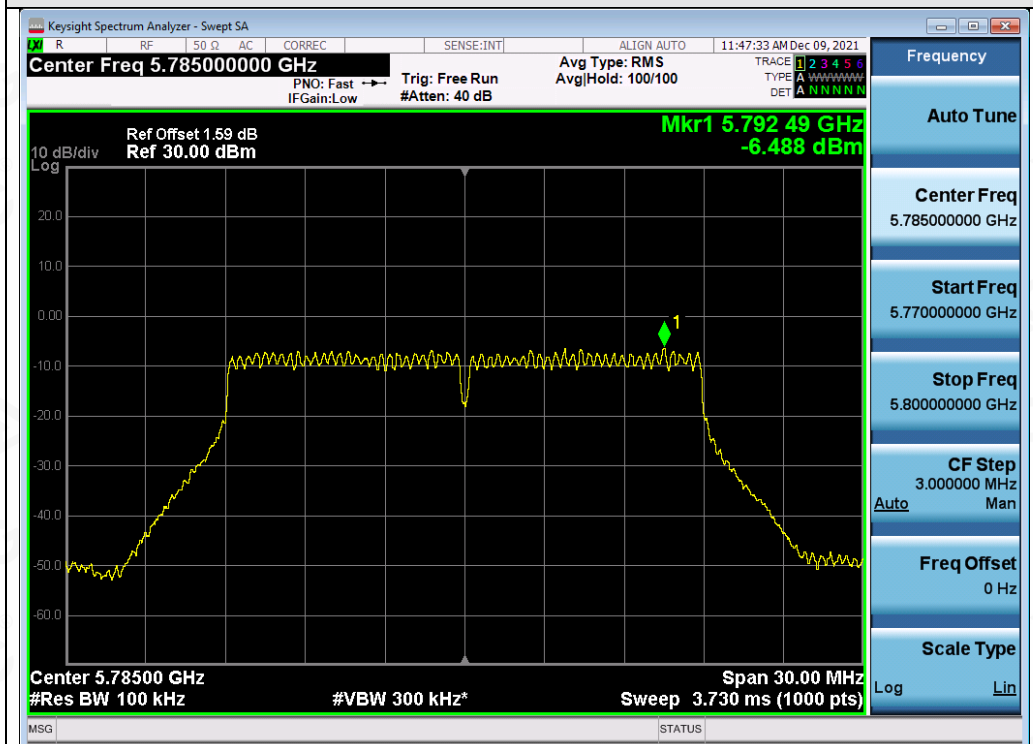
Test_Graph_802.11ac20_ANT1_5785_MCS0_PSD
