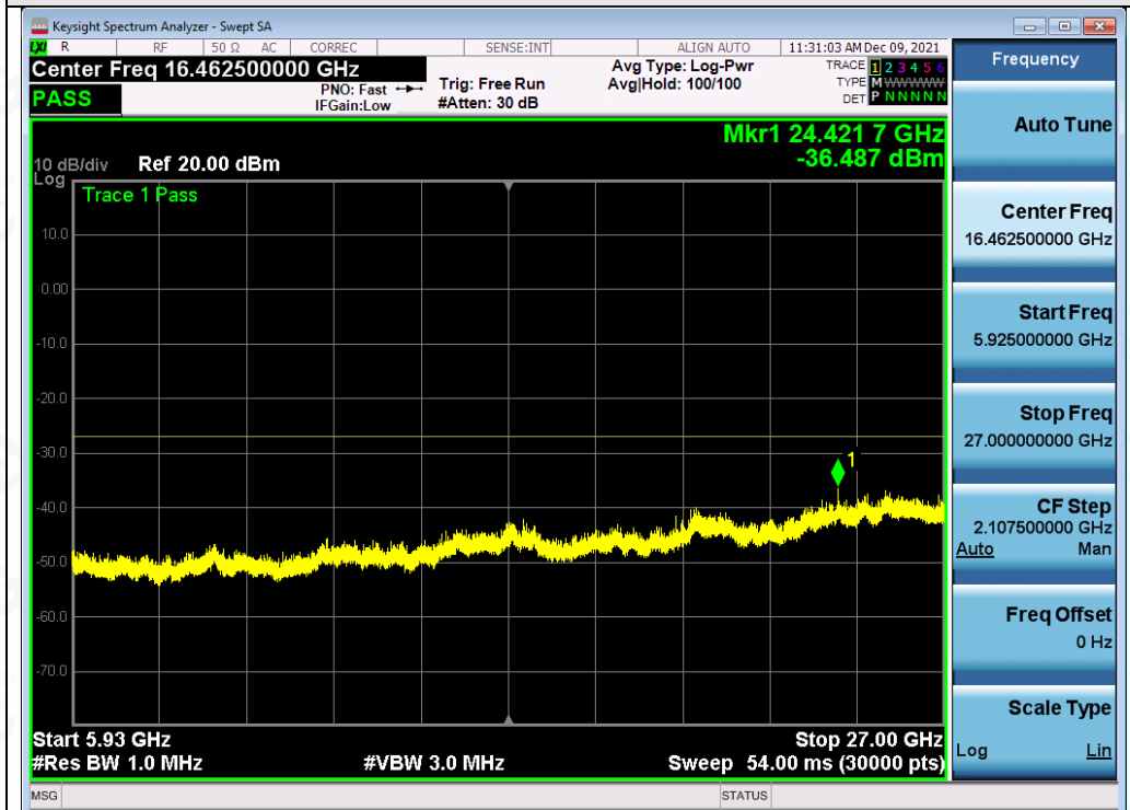
Test_Graph_802.11a_ANT1_5745_6Mbps_Frequency Band4
