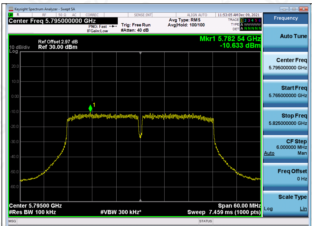
Test_Graph_802.11ac40_ANT1_5795_MCS9_PSD
