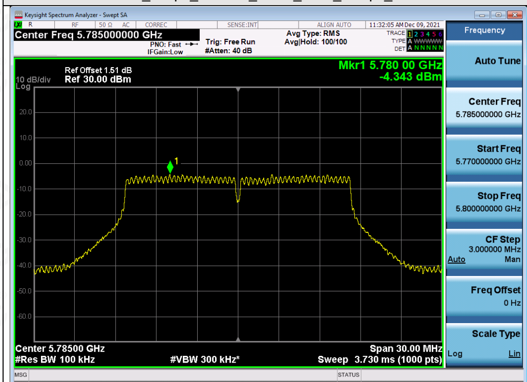
Test_Graph_802.11a_ANT1_5785_6Mbps_PSD
