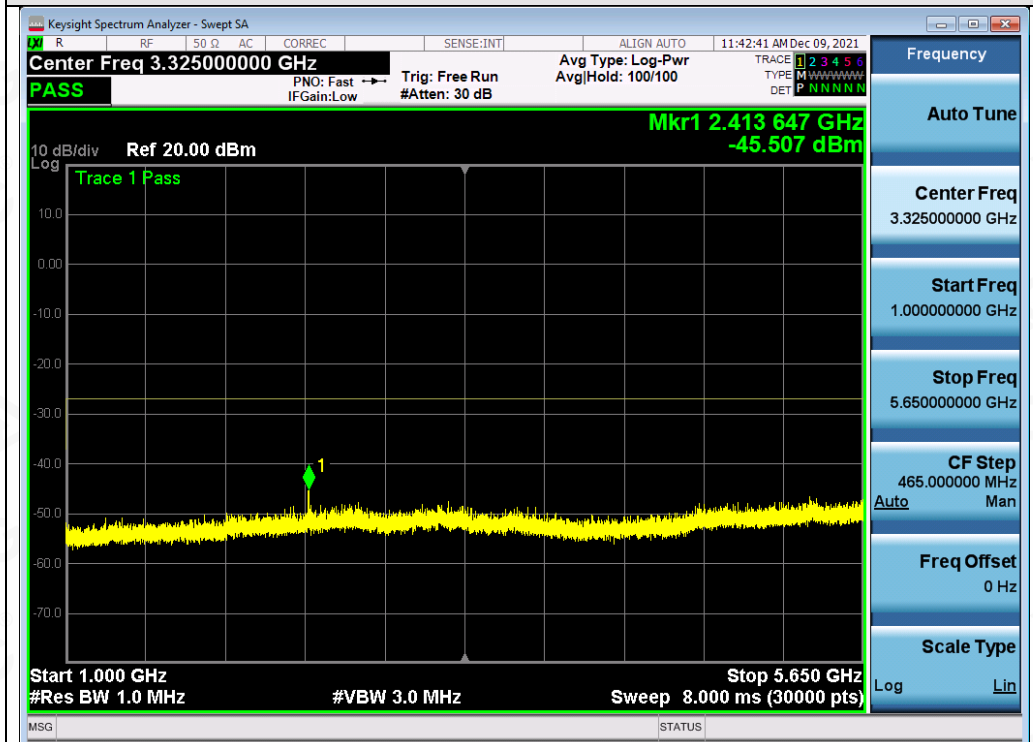
Test_Graph_802.11n40_ANT1_5795_MCS0_Frequency Band2
