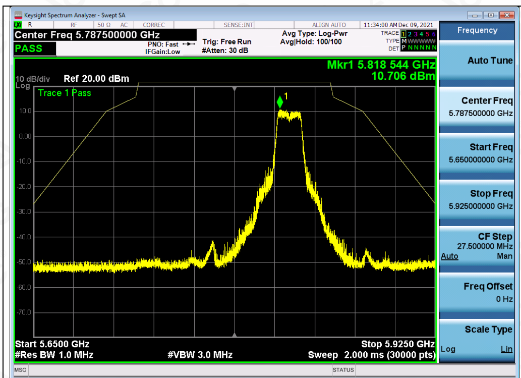
Test_Graph_802.11a_ANT1_5825_6Mbps_Frequency Band3
