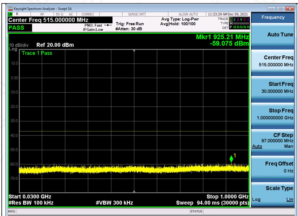
Test_Graph_802.11a_ANT1_5825_6Mbps_Frequency Band1
