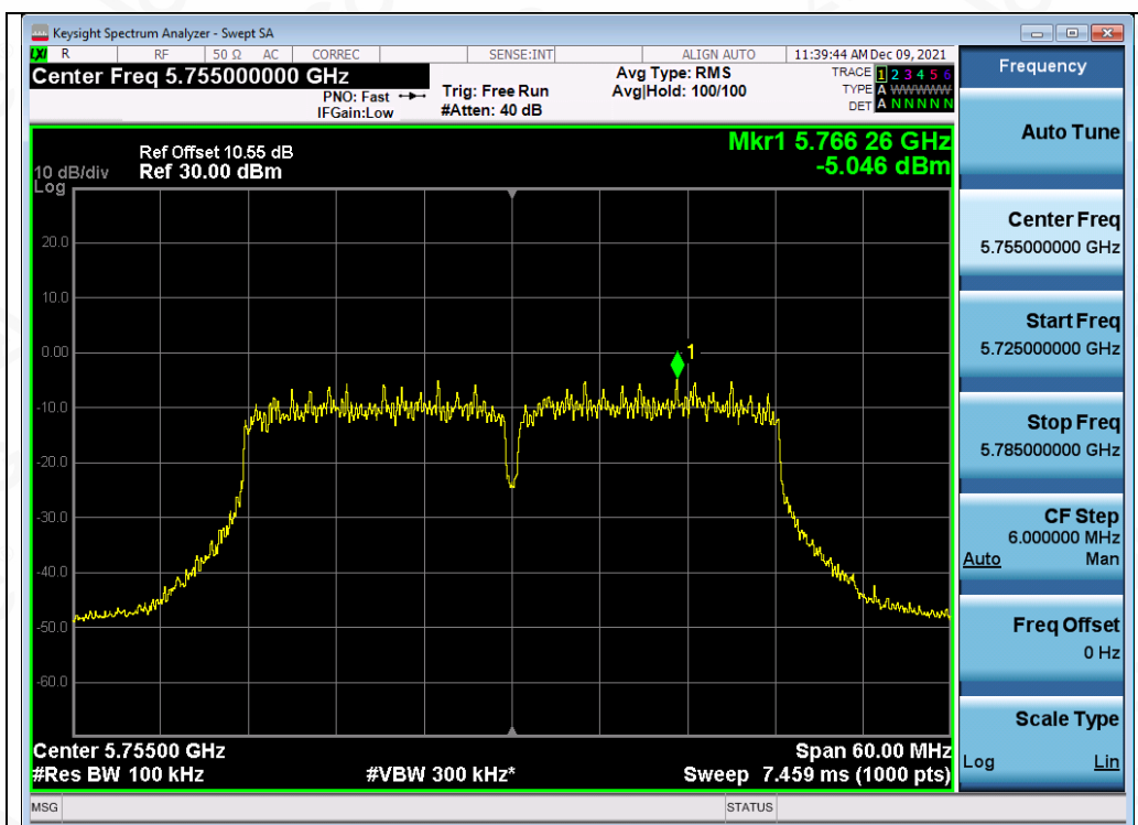
Test_Graph_802.11n40_ANT1_5755_MCS0_PSD
