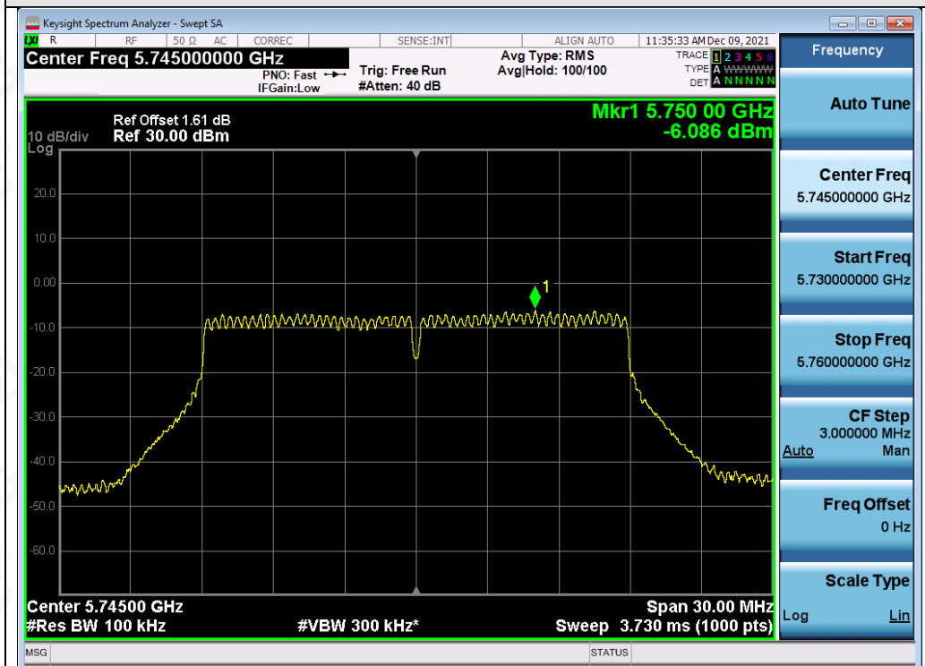
Test_Graph_802.11n20_ANT1_5745_MCS0_PSD
