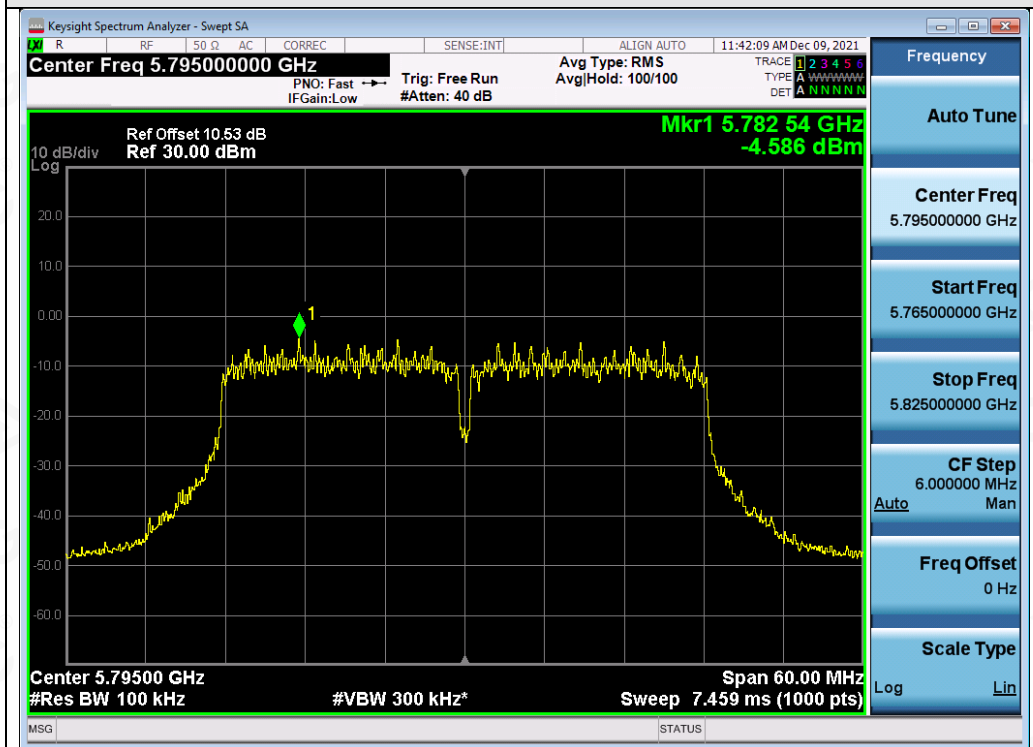
Test_Graph_802.11n40_ANT1_5795_MCS0_PSD
