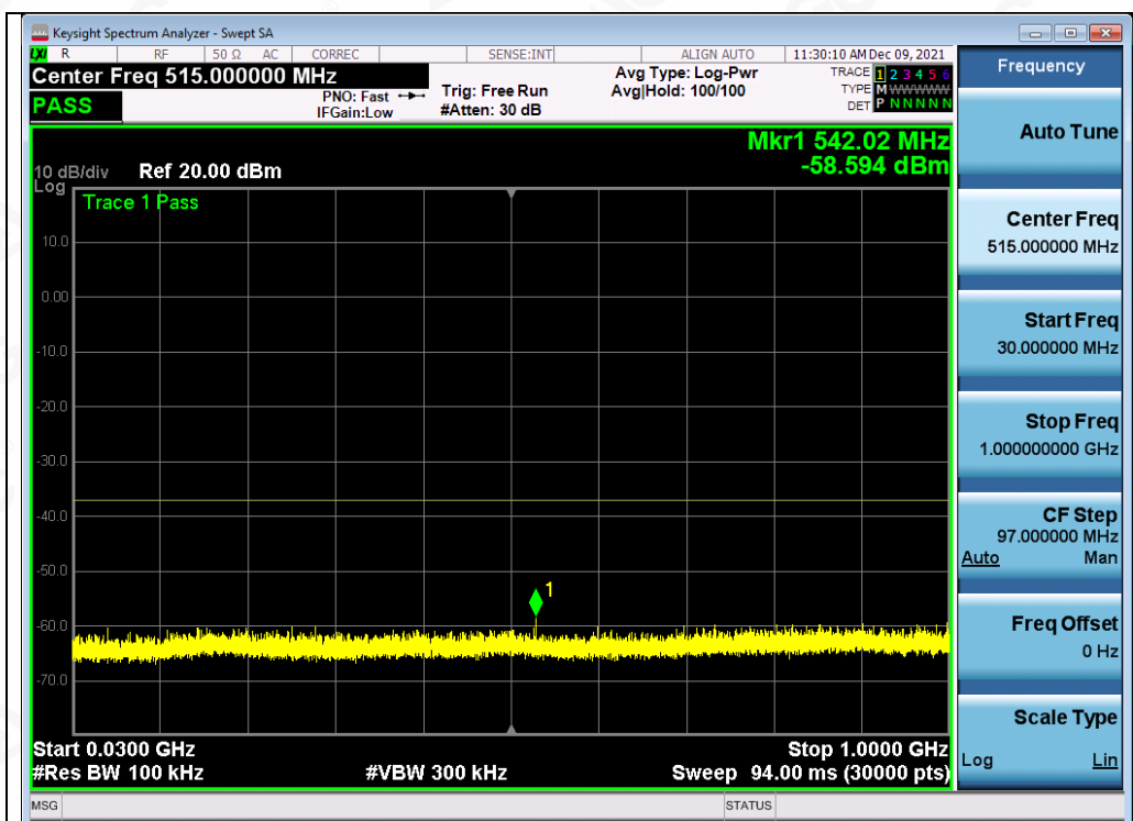
Test_Graph_802.11a_ANT1_5745_6Mbps_Frequency Band1
