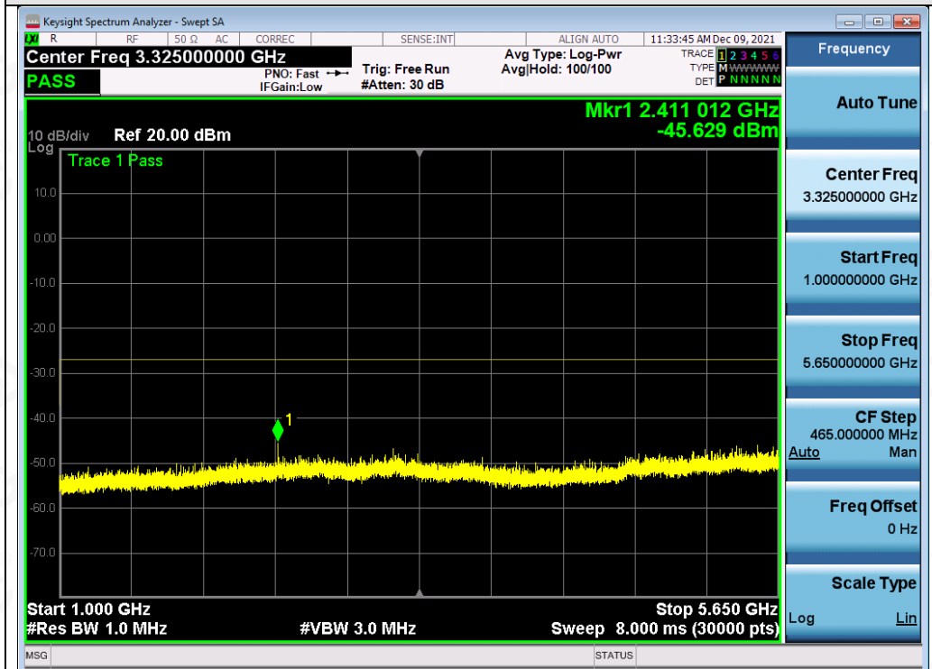
Test_Graph_802.11a_ANT1_5825_6Mbps_Frequency Band2
