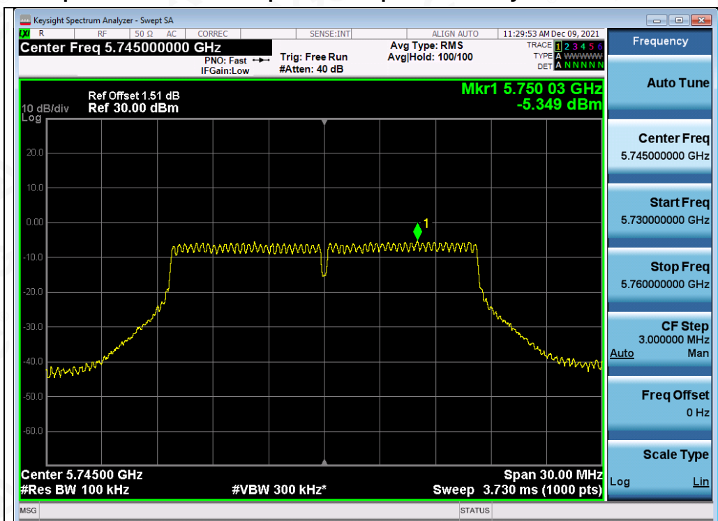
Test_Graph_802.11a_ANT1_5745_6Mbps_PSD
