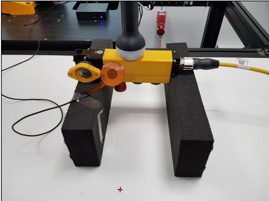
Photo 8: Test pictures - Setting distance to EUT (worst case side)
