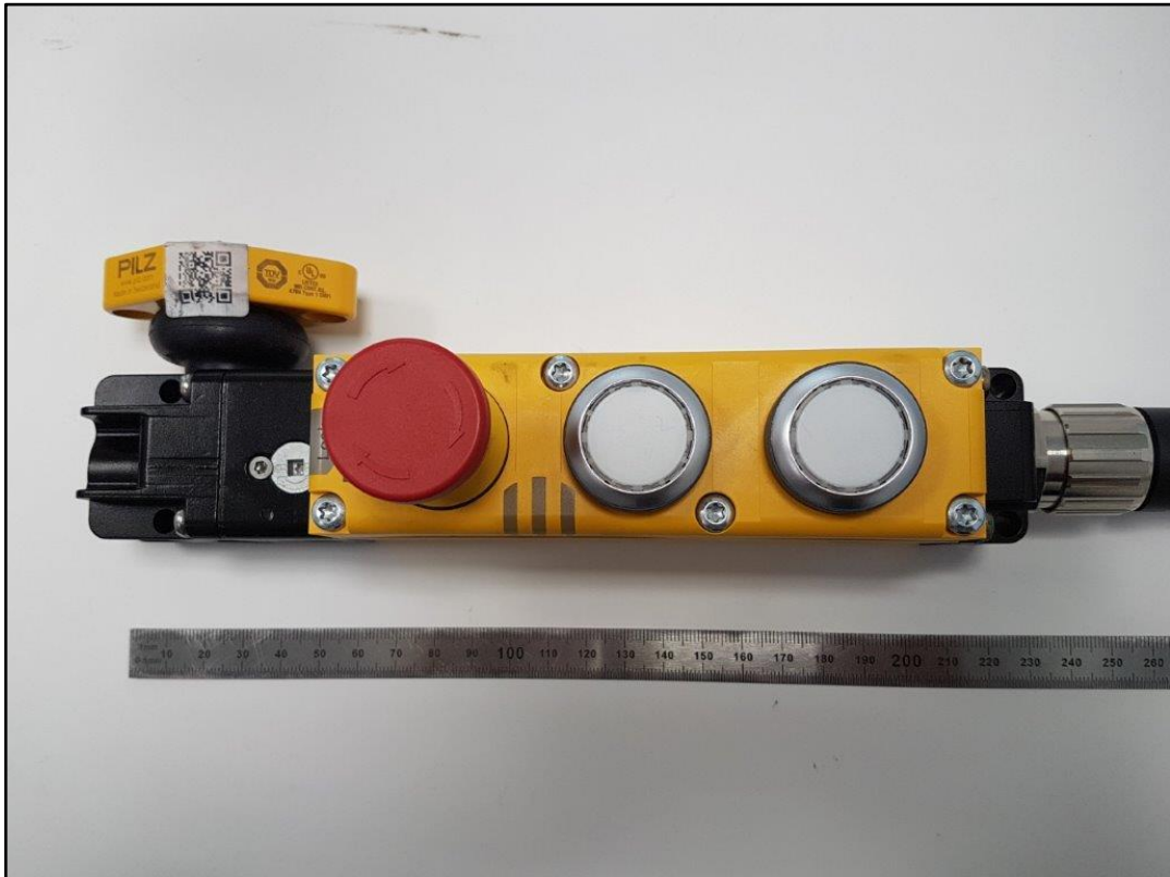
Photo 3: EUT - Front
