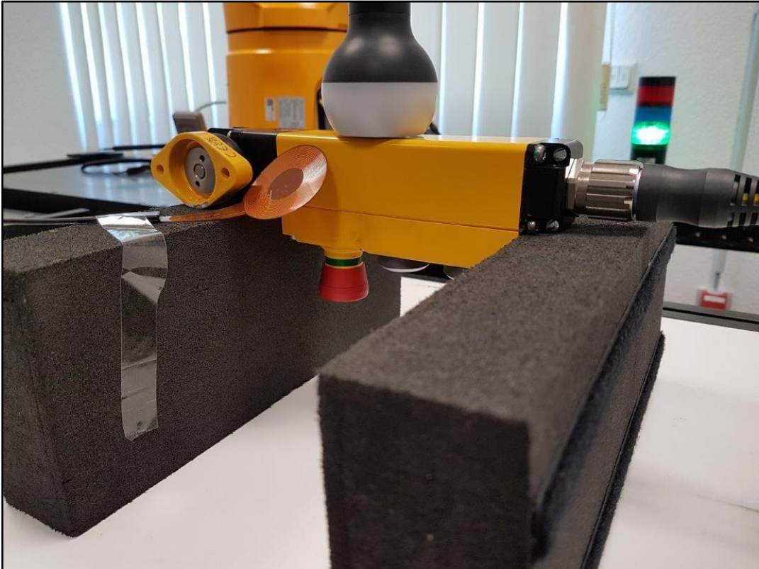
Photo 7: Test pictures - Setting distance to EUT (worst case side)
