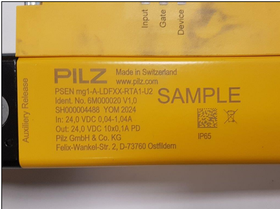
Photo 5: EUT – Serial Number
