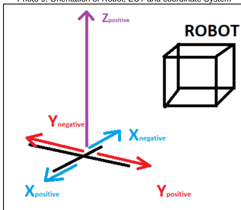
Photo 9: Orientation of Robot, EUT and coordinate System
