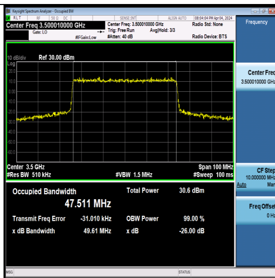
NTNV-N78-3450-3550-PC2-30-50-M-CP-16QAM-Outer_Full-Ant7-PASS
