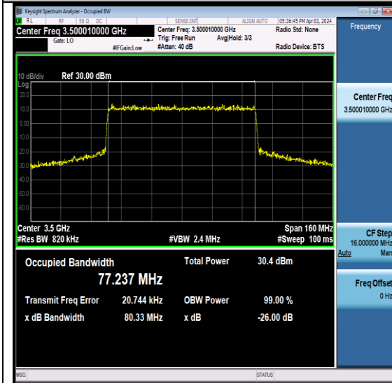
NTNV- N78-3450-3550-PC2-30-80-M-CP-64QAM-Outer_Full-Ant7-PASS
