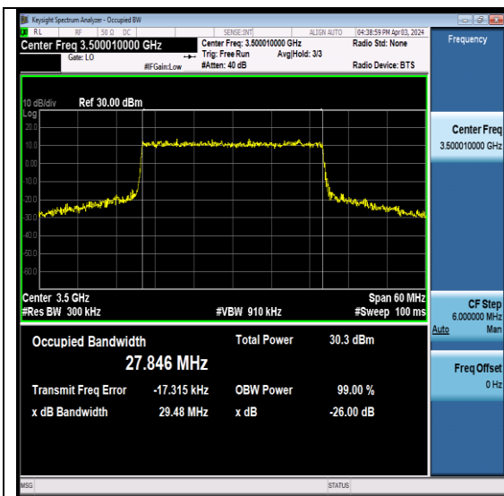
NTNV- N78-3450-3550-PC2-30-30-M-CP-QPSK-Outer_Full-Ant7-PASS
