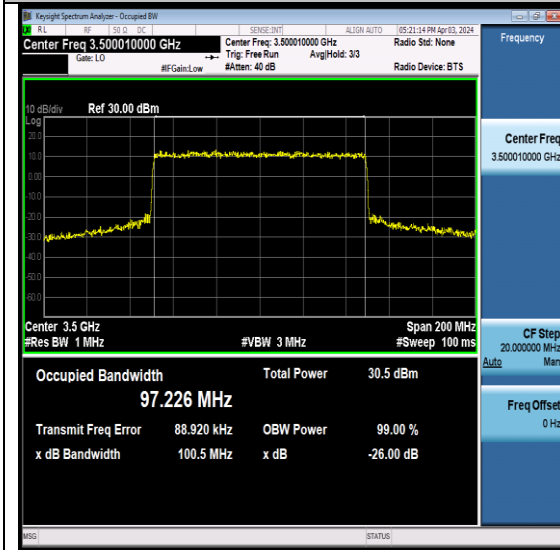
NTVN- N78-3450-3550-PC2-30-100-M-CP-64QAM-Outer_Full-Ant7-PASS
