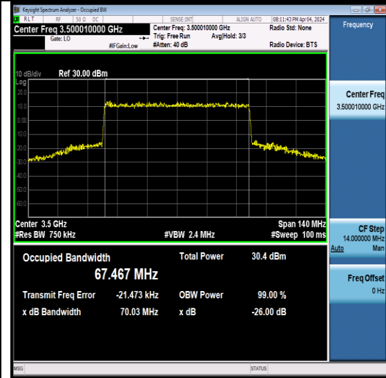
NTNV-N78-3450-3550-PC2-30-70-M-CP-256QAM-Outer_Full-Ant7-PASS
