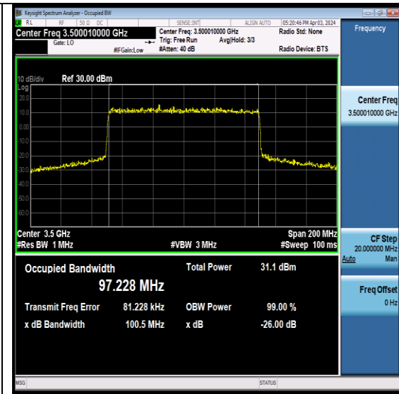
NTVN- N78-3450-3550-PC2-30-100-M-CP-16QAM-Outer_Full-Ant7-PASS
