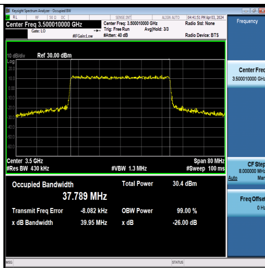
NTNV- N78-3450-3550-PC2-30-40-M-CP-16QAM-Outer_Full-Ant7-PASS
