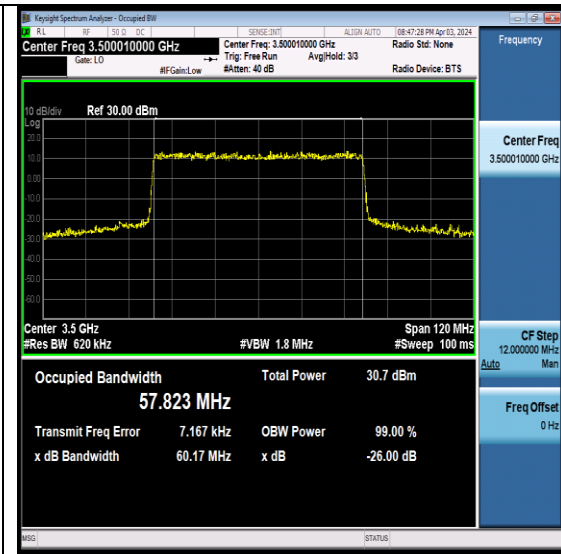
NTNV- N78-3450-3550-PC2-30-60-M-CP-16QAM-Outer_Full-Ant7-PASS
