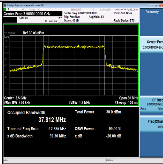
NTNV- N78-3450-3550-PC2-30-40-M-CP-256QAM-Outer_Full-Ant7-PASS
