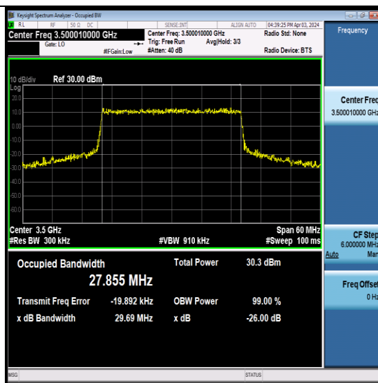
NTNV- N78-3450-3550-PC2-30-30-M-CP-16QAM-Outer_Full-Ant7-PASS
