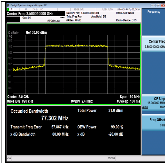
NTNV- N78-3450-3550-PC2-30-80-M-CP-QPSK-Outer_Full-Ant7-PASS
