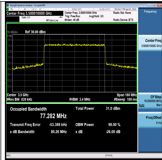
NTNV- N78-3450-3550-PC2-30-80-M-CP-16QAM-Outer_Full-Ant7-PASS
