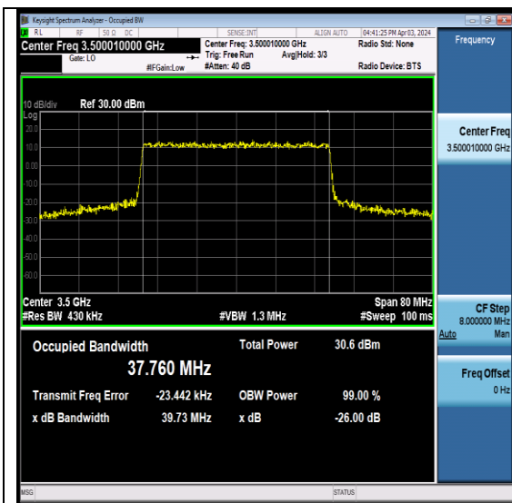
NTNV- N78-3450-3550-PC2-30-40-M-CP-QPSK-Outer_Full-Ant7-PASS
