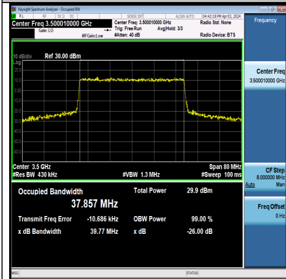
NTNV- N78-3450-3550-PC2-30-40-M-CP-64QAM-Outer_Full-Ant7-PASS
