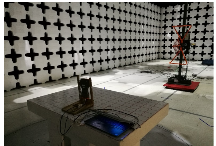
Radiated Emissions (>1GHz) - Rear View
