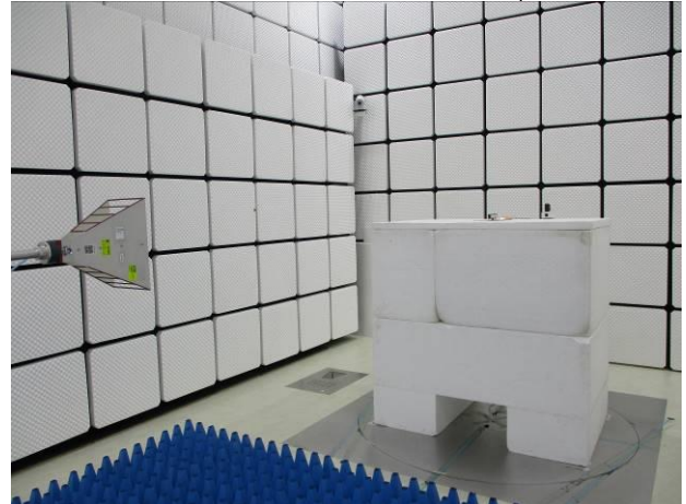
FCC_15_407_WLAN_Radiated_Setup
