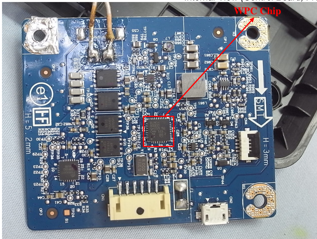
Figure 30 Internal View (Control Board, Front View)
