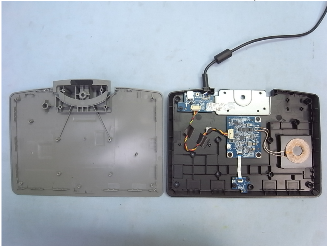
Figure 24 Internal View (Removed Cover of Base)
