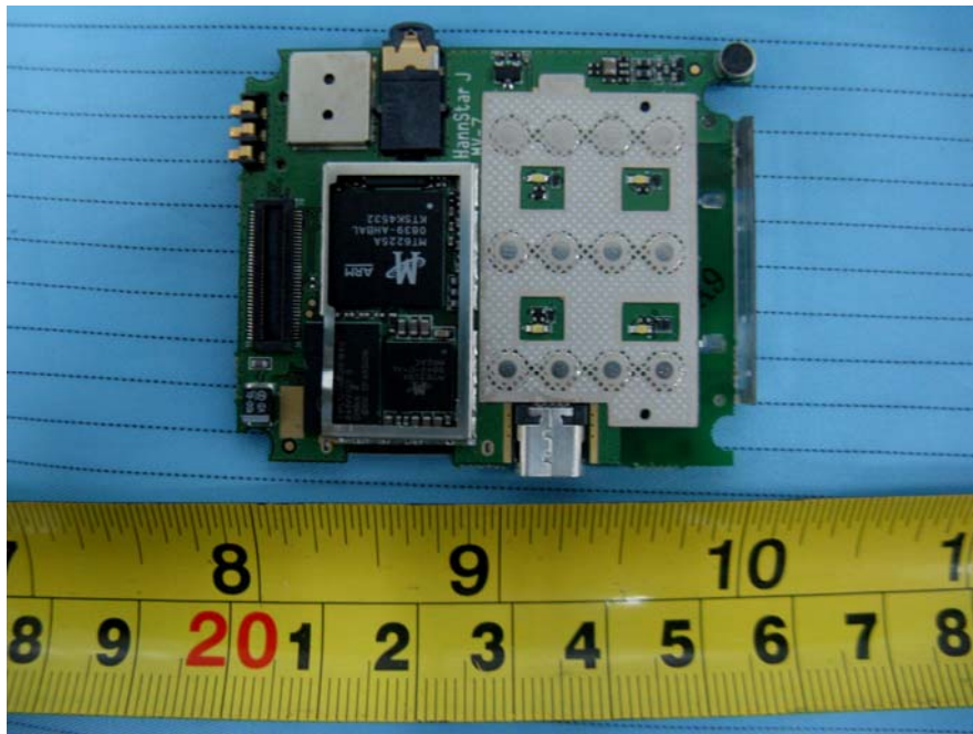
EUT – Main Board Bottom Uncovered View
