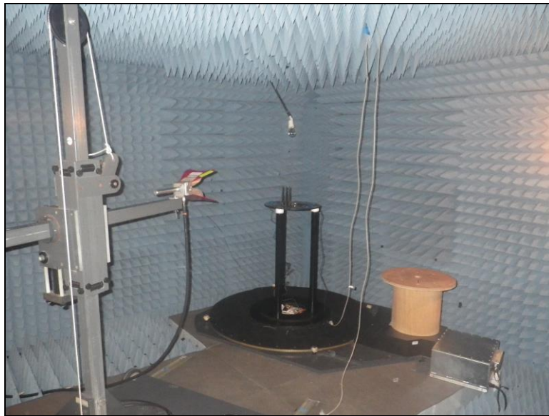
Photograph 2. Radiated Test Setup, Above 1GHz
