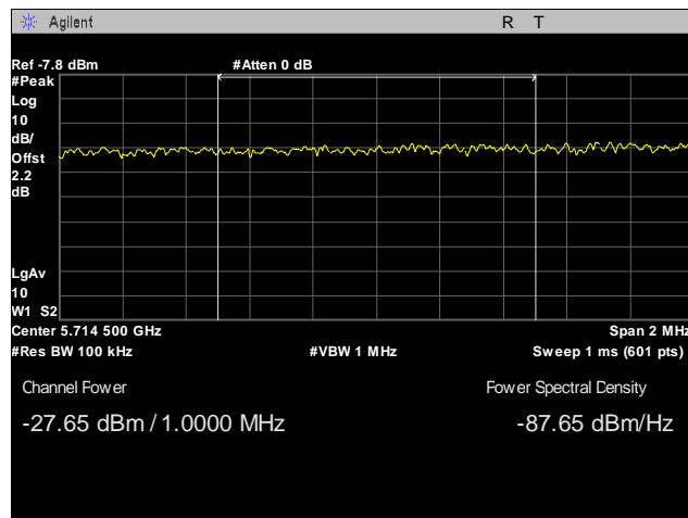
Plot 46. Radiated Band Edge, Low Channel, 40 MHz, -27 Peak Integration
