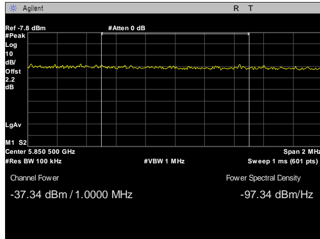
Plot 42. Radiated Band Edge, High Channel, 20 MHz, -17 Peak Integration
