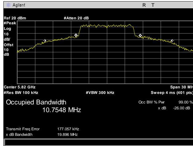
Plot 4. Occupied Bandwidth, 5820 MHz, 10 MHz
