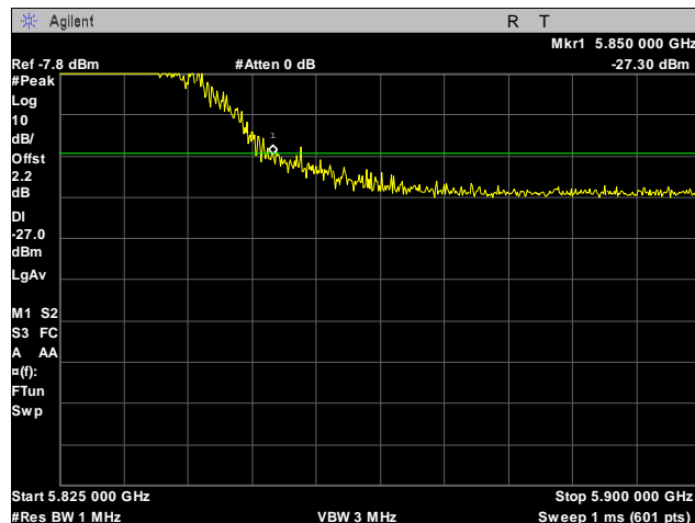
Plot 44. Radiated Band Edge, High Channel, 20 MHz, -27 Peak
