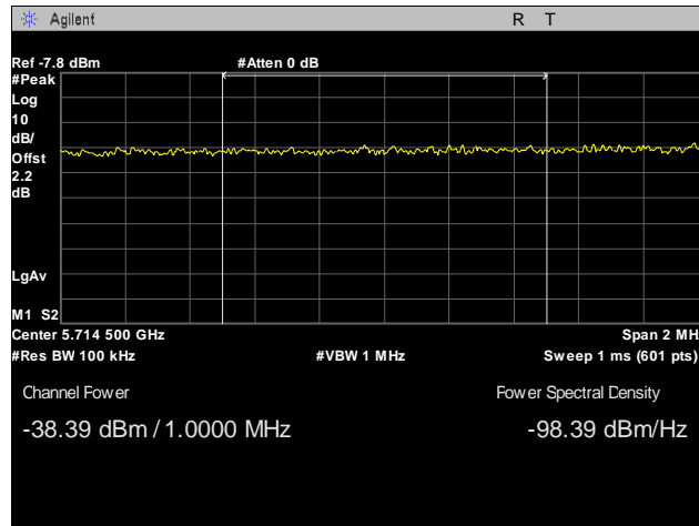
Plot 36. Radiated Band Edge, Low Channel, 10 MHz, -27 Peak Integration
