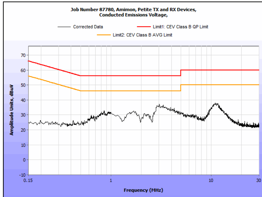
Plot 49. Conducted Emissions, Neutral Line
