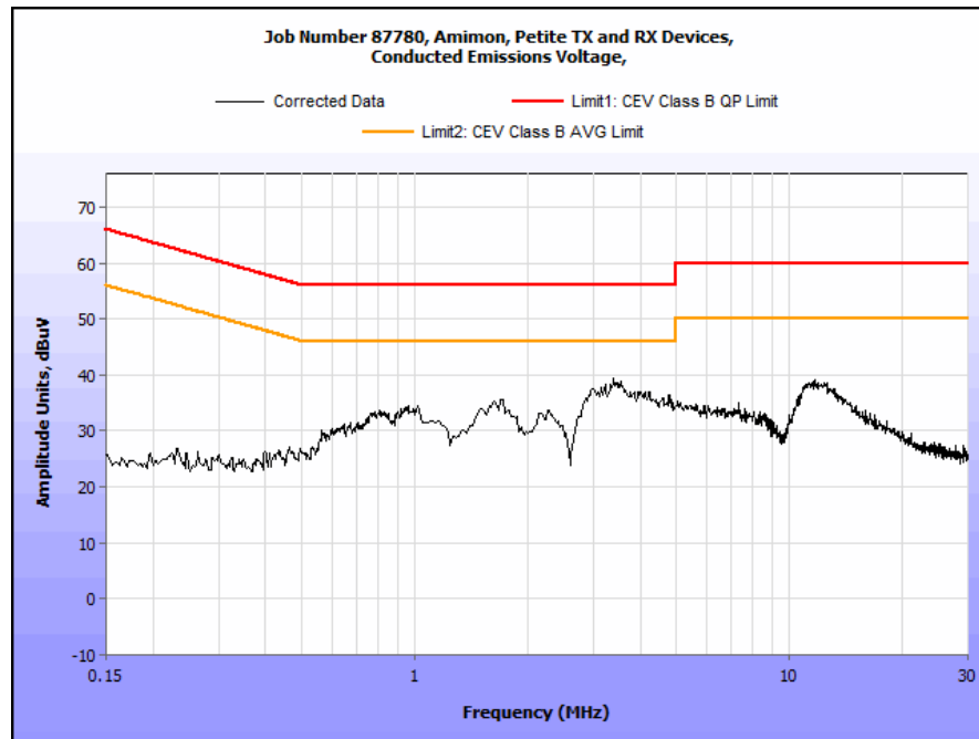
Plot 48. Conducted Emissions, Phase Line
