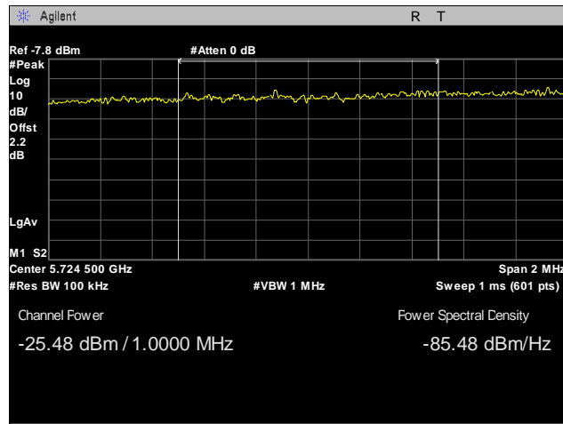
Plot 39. Radiated Band Edge, Low Channel, 20 MHz, -17 Peak Integration
