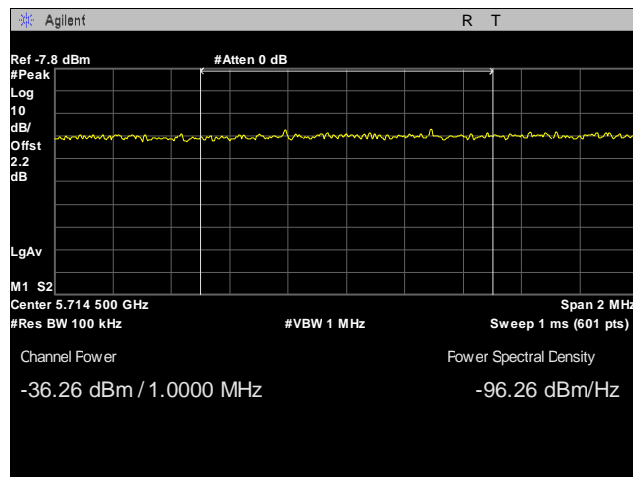
Plot 40. Radiated Band Edge, Low Channel, 20 MHz, -27 Peak Integration
