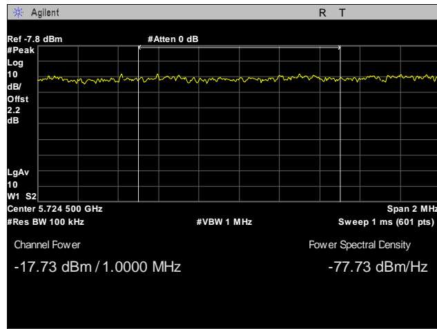
Plot 45. Radiated Band Edge, Low Channel, 40 MHz, -17 Peak Integration
