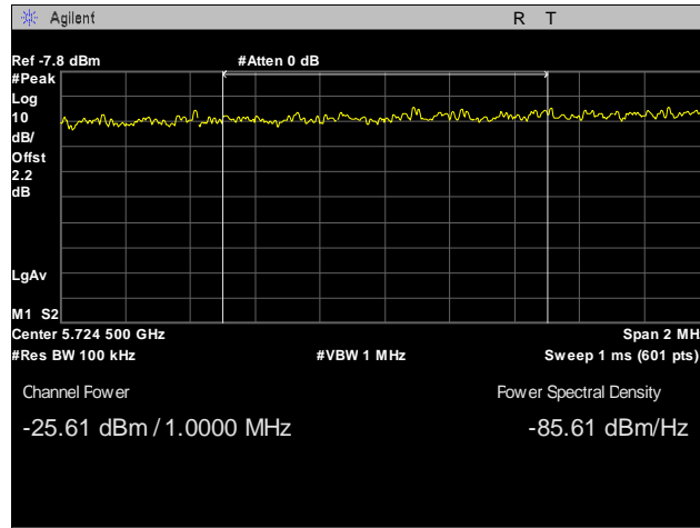
Plot 35. Radiated Band Edge, Low Channel, 10 MHz, -17 Peak Integration
