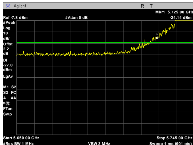
Plot 41. Radiated Band Edge, Low Channel, 20 MHz, -27 Peak
