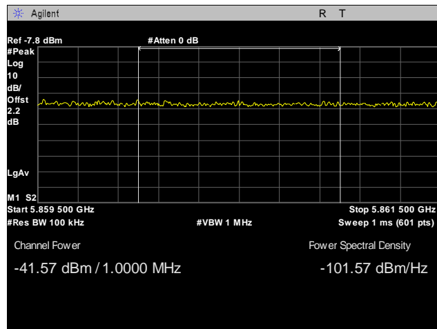
Plot 43. Radiated Band Edge, High Channel, 20 MHz, -27 Peak Integration
