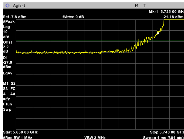
Plot 37. Radiated Band Edge, Low Channel, 10 MHz, Peak
