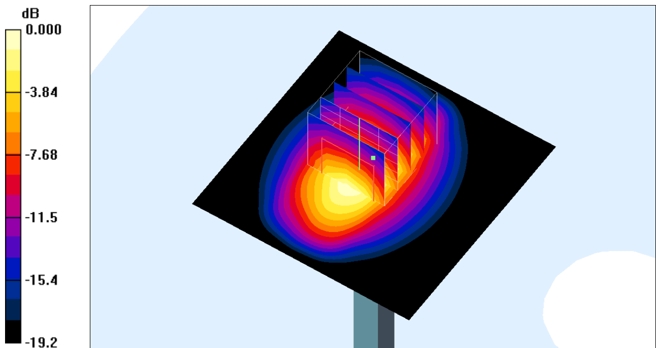
0 dB = 14.8mW/g
