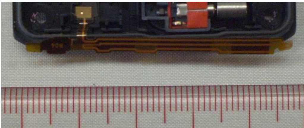
BT/WLAN Antenna
