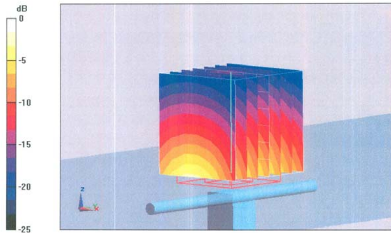
0 dB = 16.9mW/g
