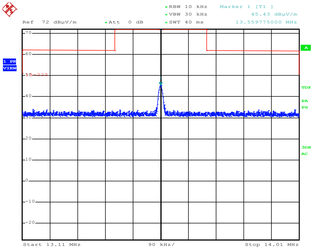
Figure 7: Spektrum mask of 13.56 MHz @ 3m distance
