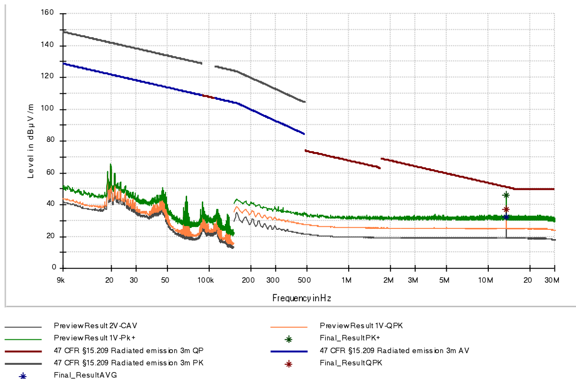
Figure 8: Chart of emissions test below 30 MHz without tag in position 2, antenna parallel @ 3 m
