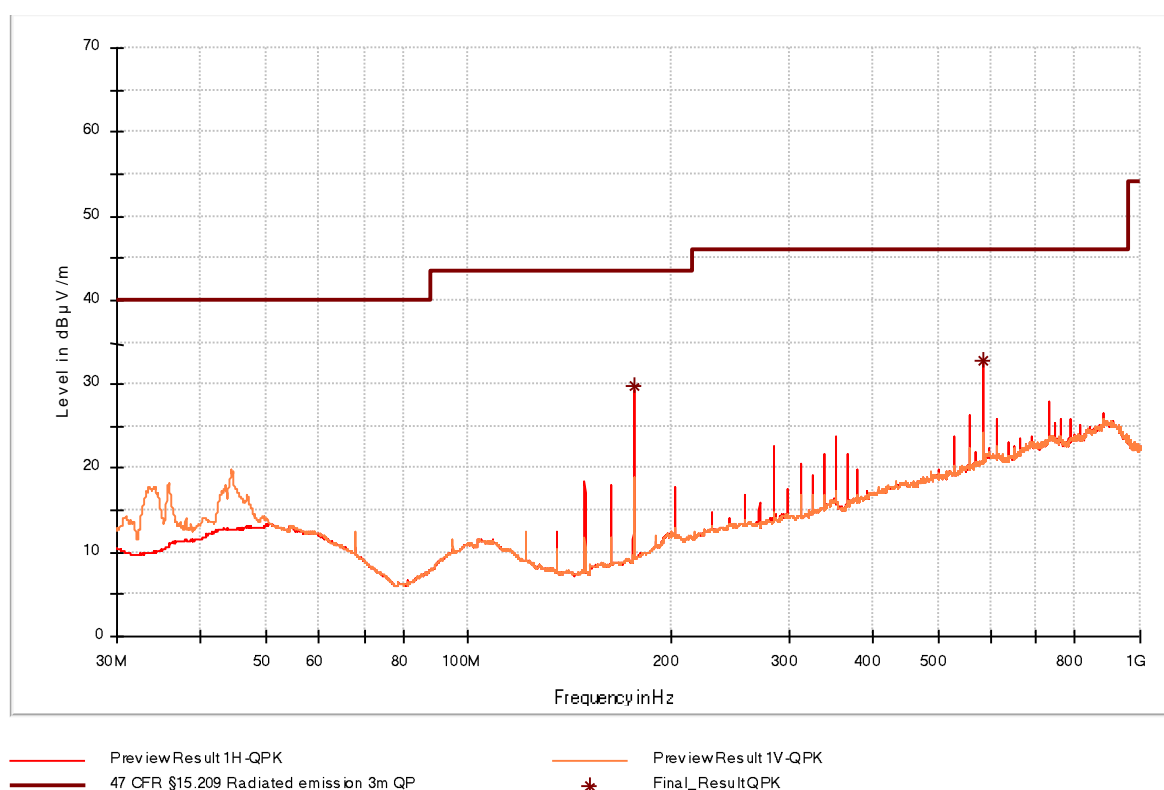
Figure 9: Chart of emissions test from 30 MHz to 1 GHz with tag in position 1
