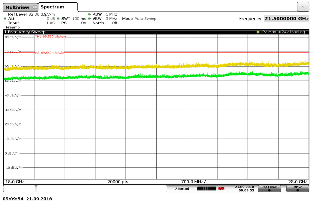
Figure 12: Chart of radiated disturbance test 18 GHz – 25 GHz – exploratory measurement- polarization vertical + horizontal
