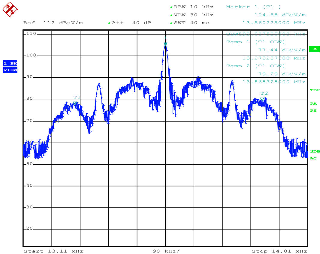
Figure 6: Chart of occupied bandwidth test
