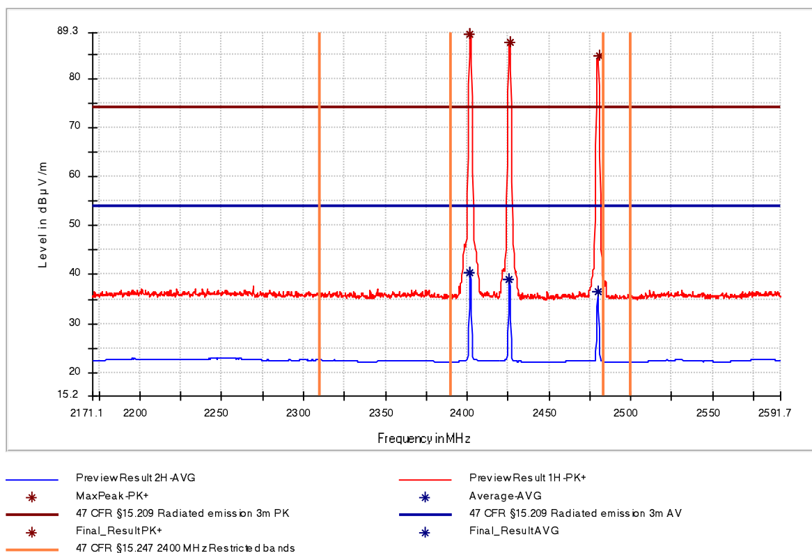
Figure 13: Chart of radiated emission – Band edge compliance
