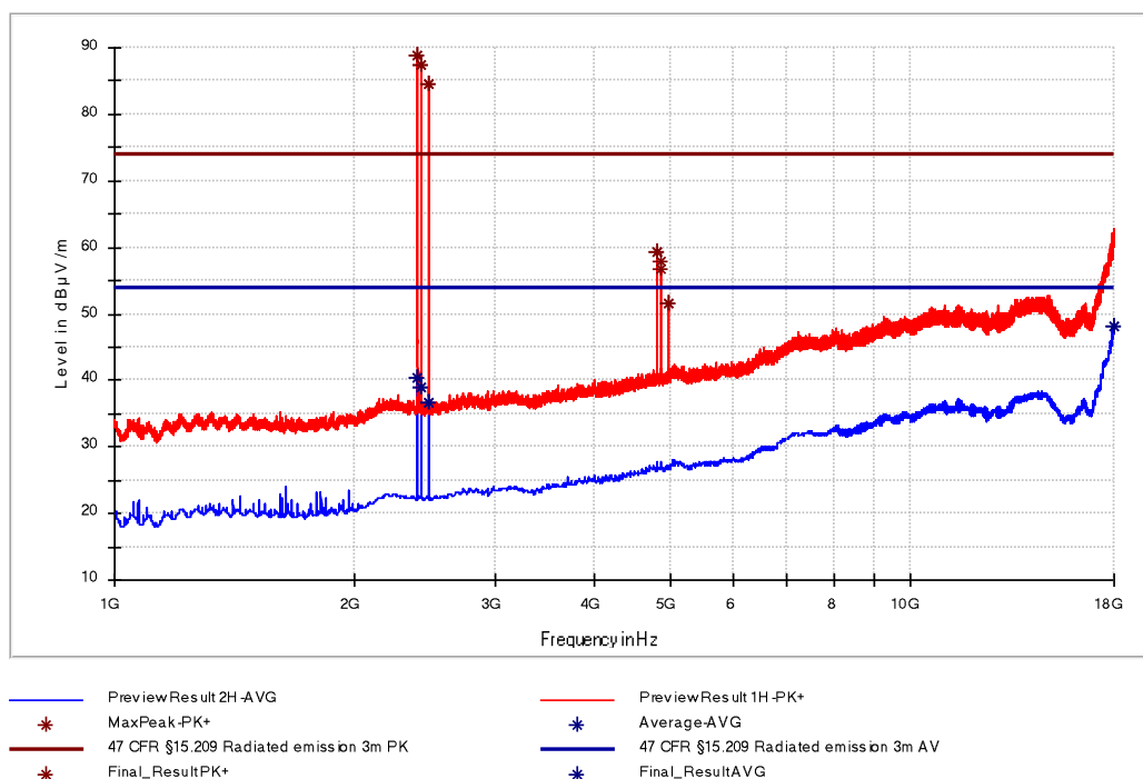
Figure 10: Chart of radiated disturbance test 1 GHz – 18 GHz, with tag, EUT position 1, horizontal polarization of antenna
