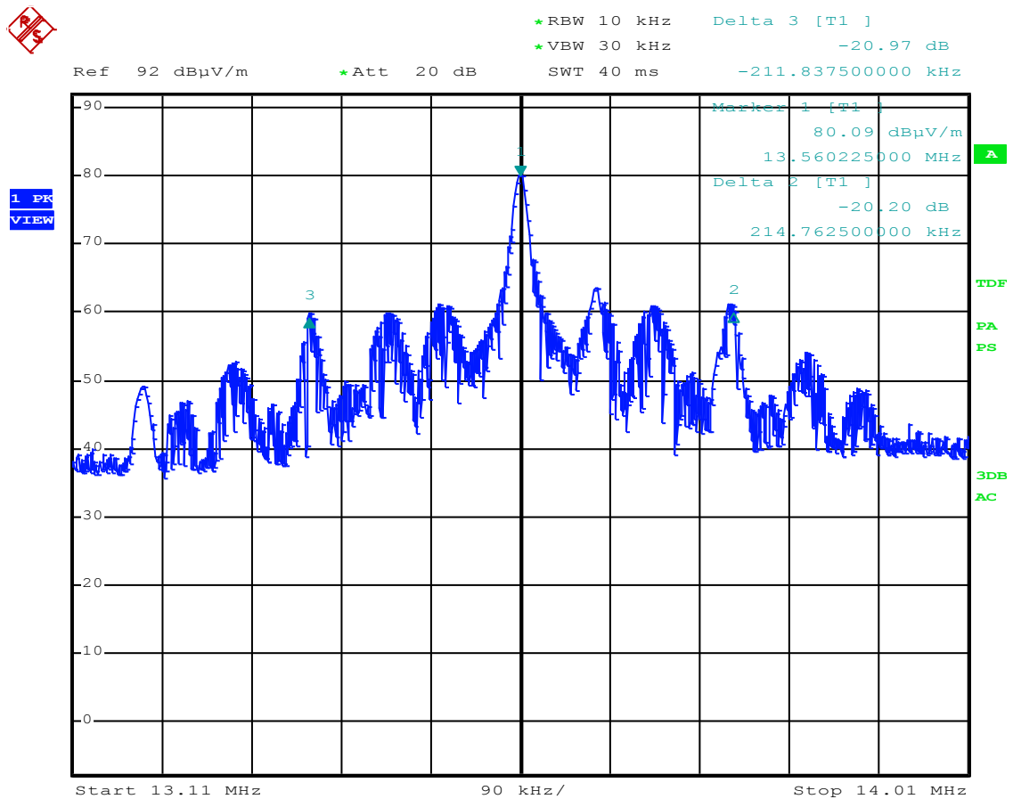
Figure 5: Chart of 20 dB bandwidth on channel 01
