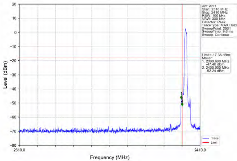
8DPSK_3DH5_LCH_2402MHz_Ant1_NTNV
