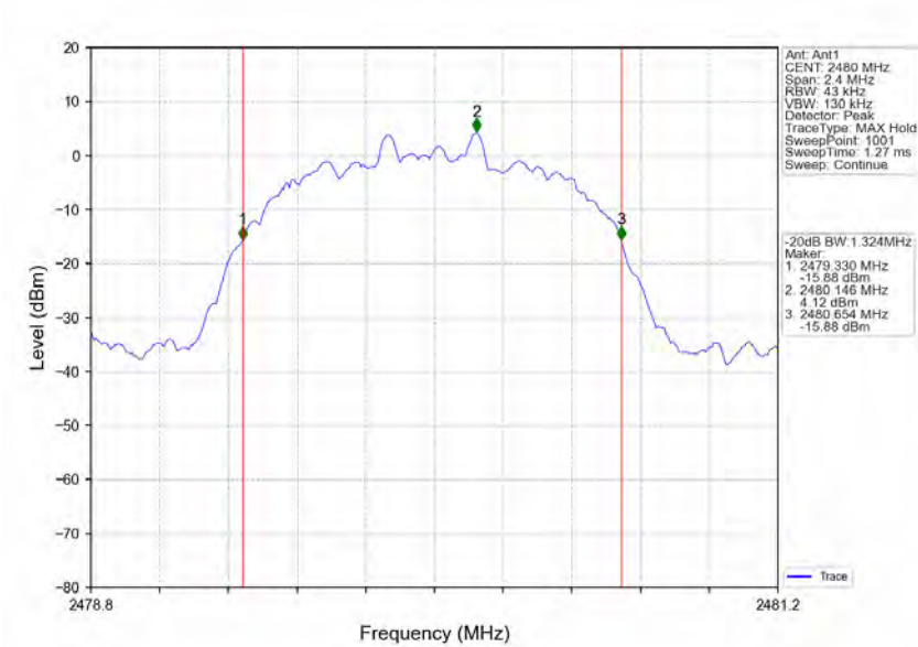
8DPSK_3DH5_HCH_2480MHz_Ant1_NTNV
