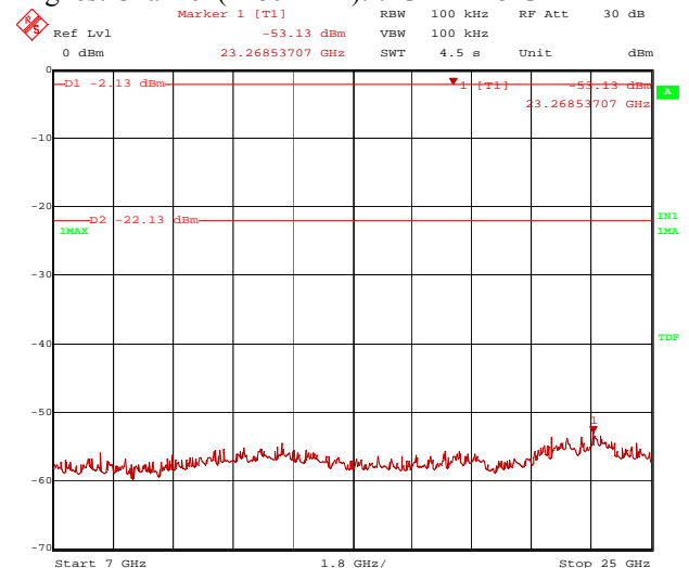
Highest Channel (2480 MHz): 7 GHz ~ 25 GHz
