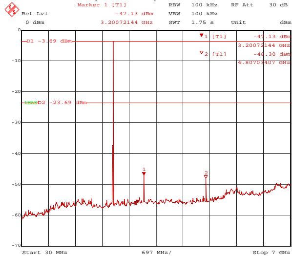
Lowest Channel (2402 MHz): 30 MHz ~ 7 GHz
