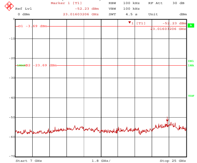
Lowest Channel (2402 MHz): 7 GHz ~ 25 GHz
