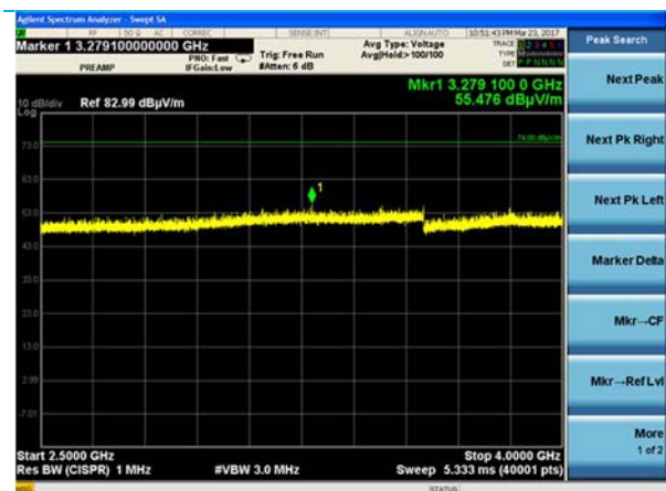
2.5-4 GHz – H+V Antenna
