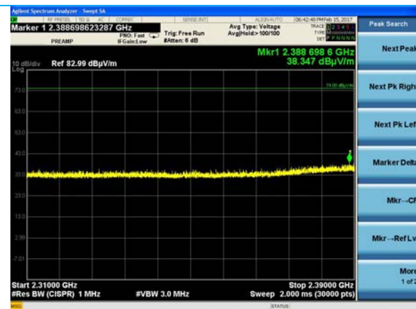
MCS0 – HT40 - Peak
