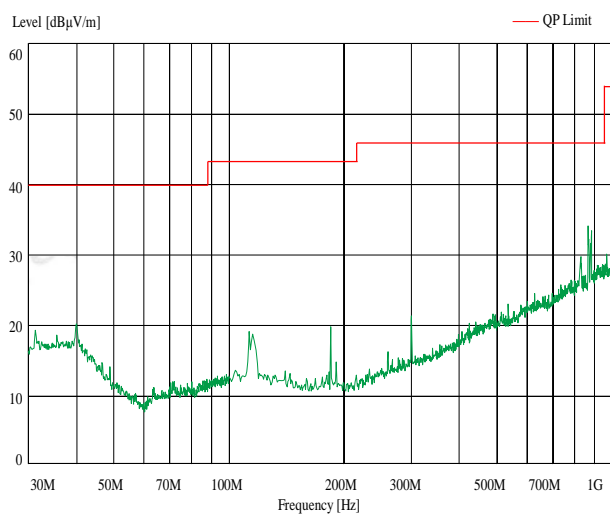
Antenna Vertical
