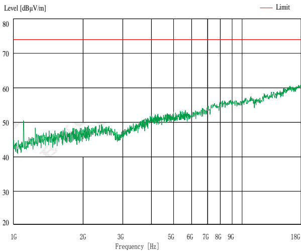
Antenna Horizontal
