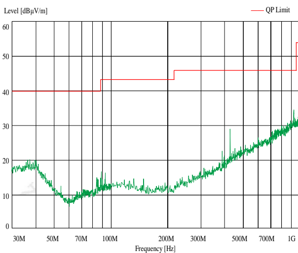
Antenna Horizontal
