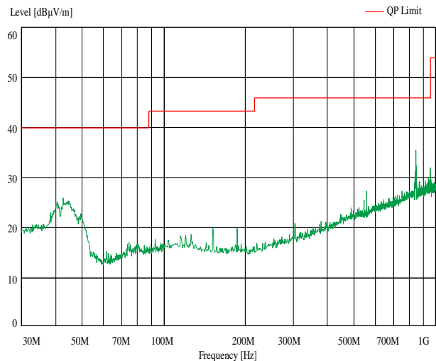
Antenna Vertical
