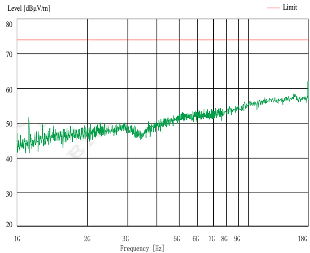
Antenna Vertical
