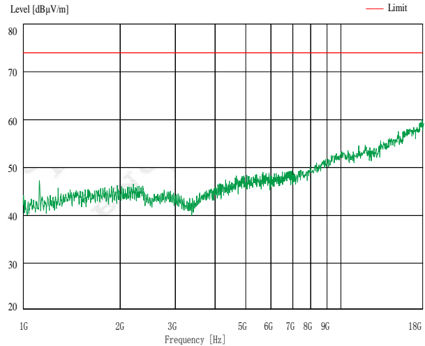
Antenna Vertical
