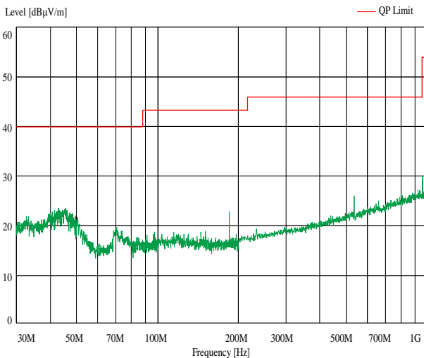
Antenna Horizontal
