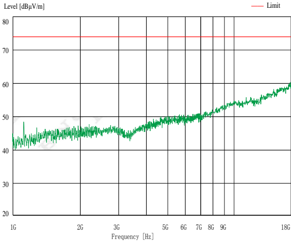
Antenna Horizontal
