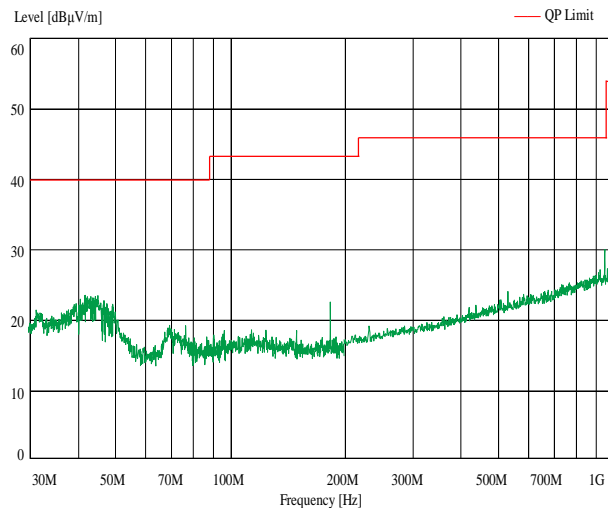
Antenna Vertical
