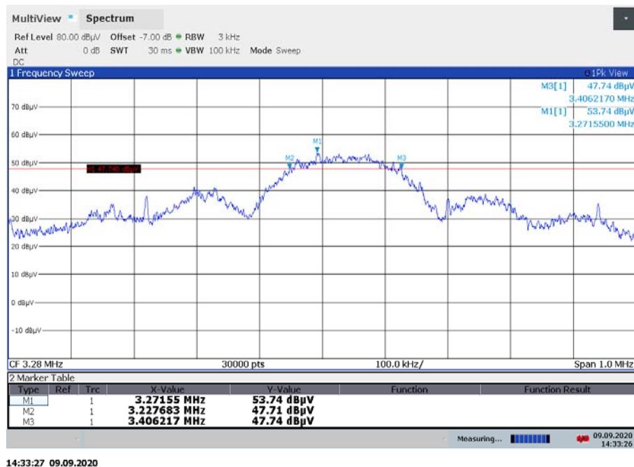
Plot 2: 6 dB bandwidth, 320 kbit/s
