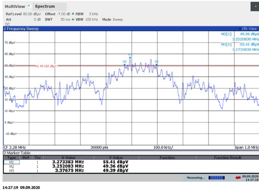
Plot 1: 6 dB bandwidth, 80 kbit/s
