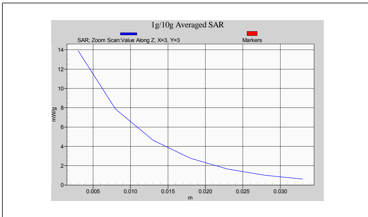
Body-Tissue-Simulating-Liquid 1900MHz
