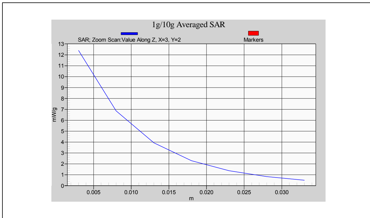
Head-Tissue-Simulating-Liquid 1900MHz
