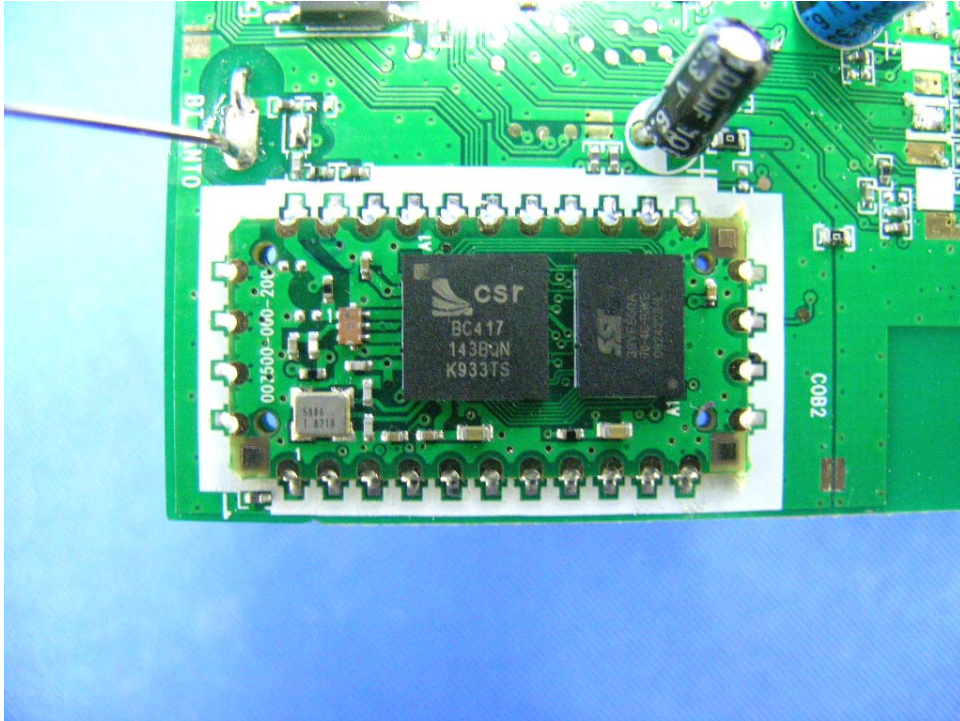
Base Unit Bluetooth RF Module front side
