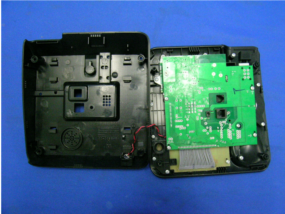
Base Unit assembly (View 1)
