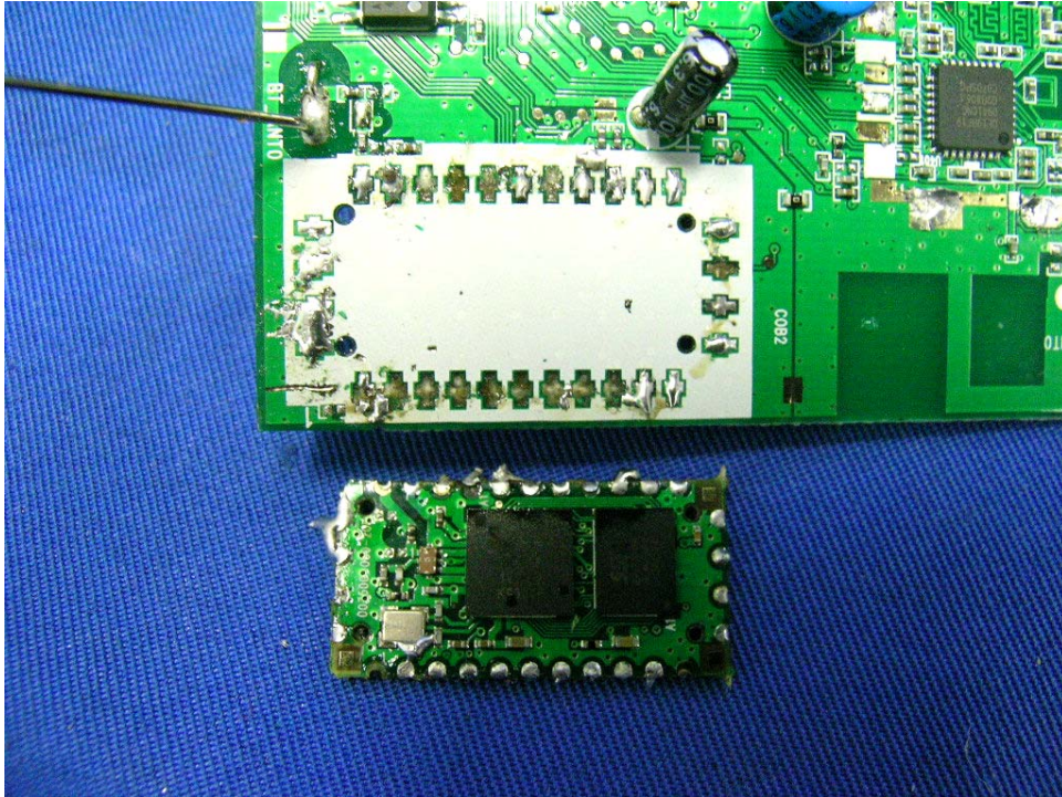
Base Unit Main PCB comp side (View 5)
