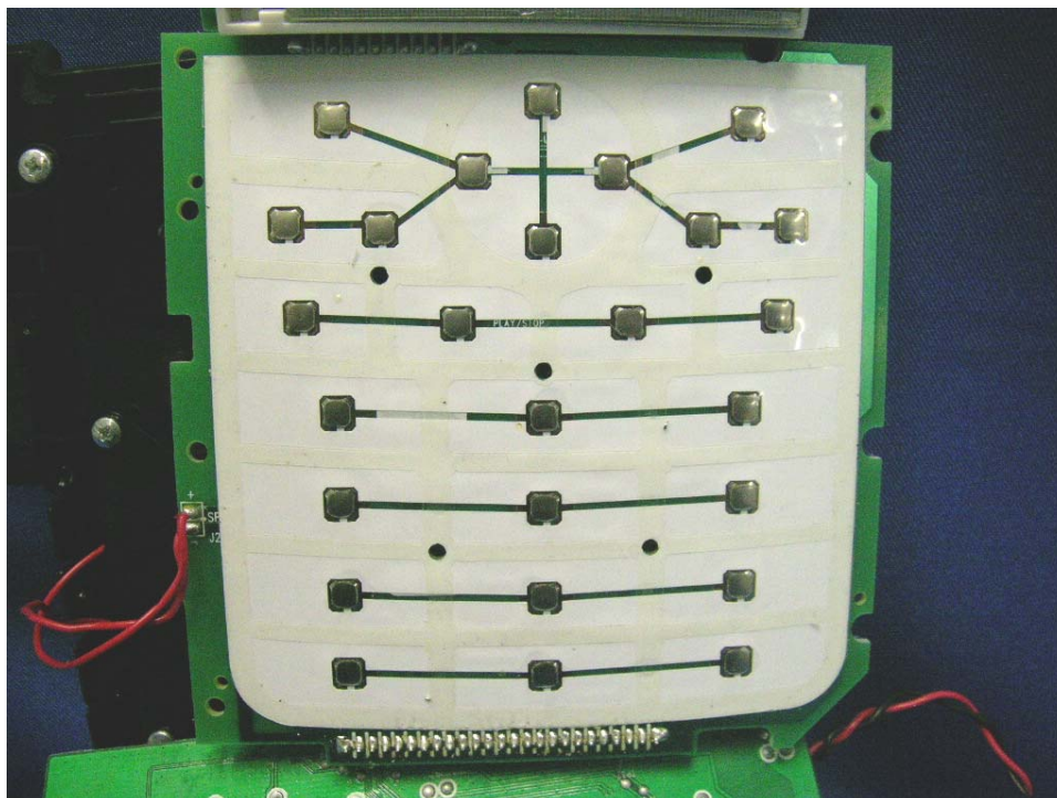
Keypad PCB front side
