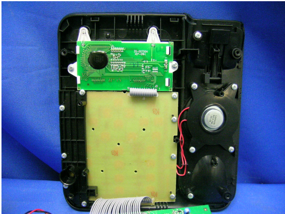
Base Unit assembly (View 2) (LCD & Keypad PCB rear side)
