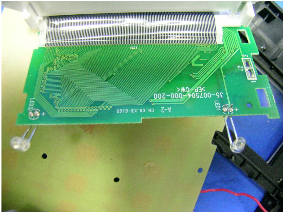
LCD PCB front side (View 1)
