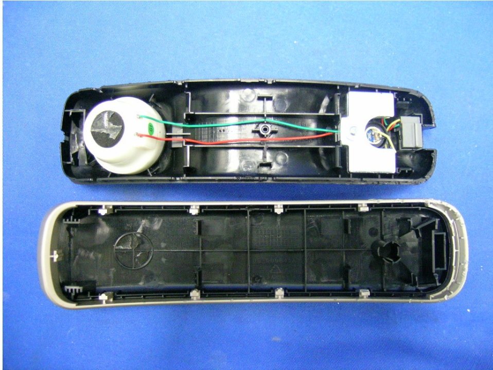
Corded handset internal view
