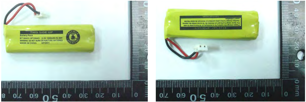
Figure 2. Battery (Ni-MH 2.4V , 500mAh)
