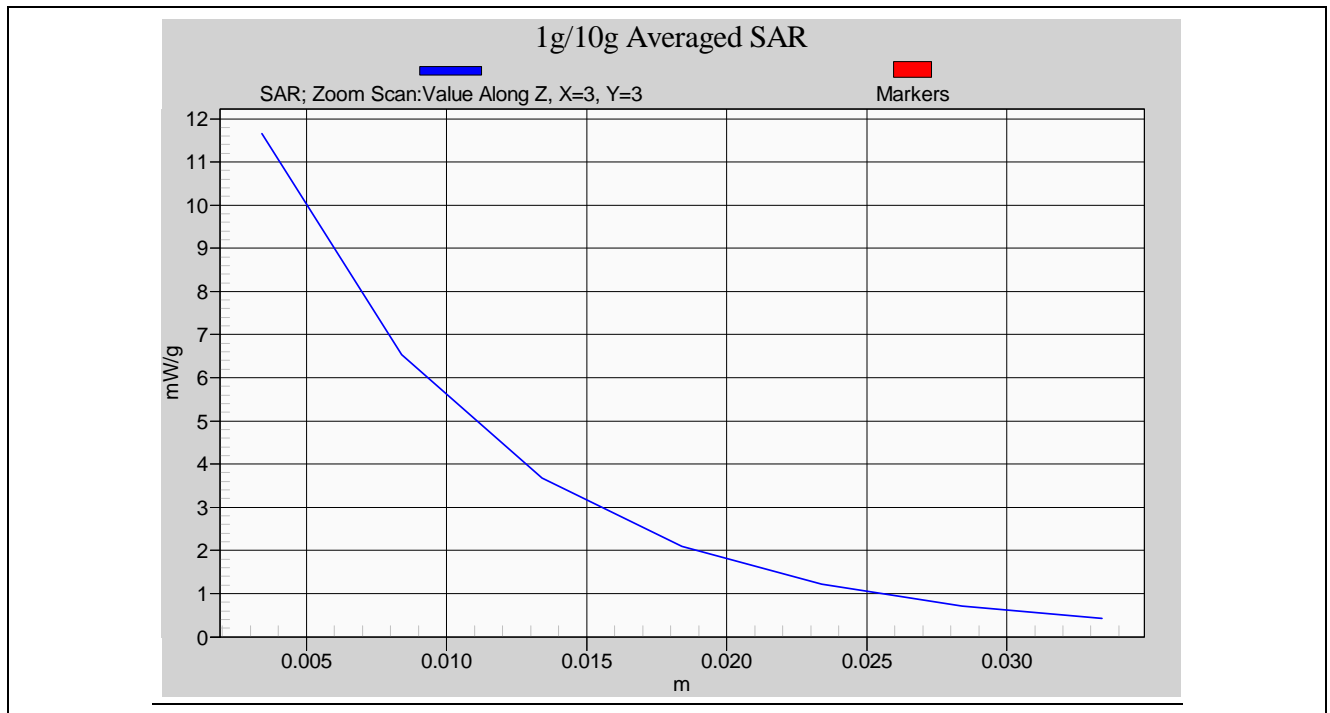
Head-Tissue-Simulating-Liquid 1900MHz
