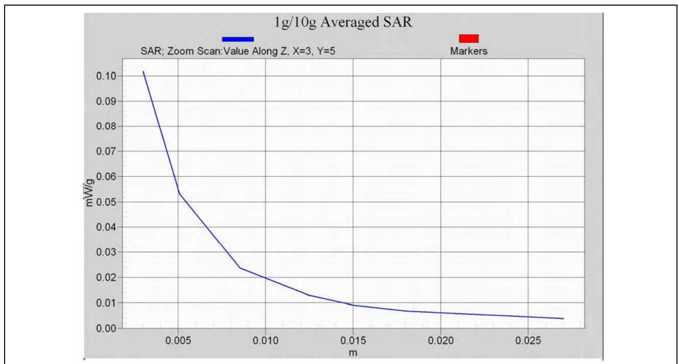
Body SAR Measurement _ Back to Phantom 2mm separation _CH4
