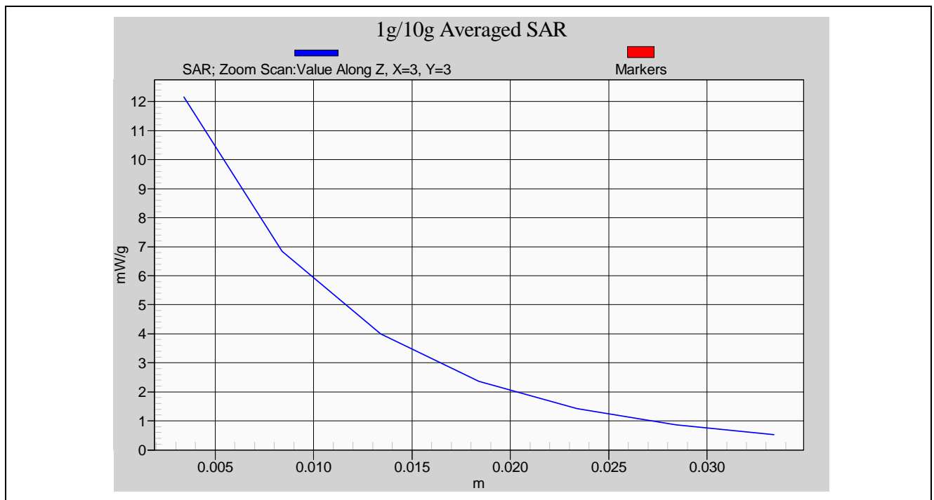
Body-Tissue-Simulating-Liquid 1900MHz
