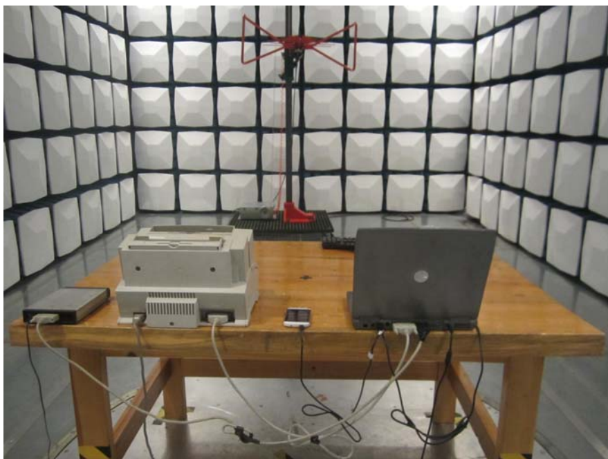
Radiated Emissions –Rear View (Below 1GHz) (USB Downloading)
