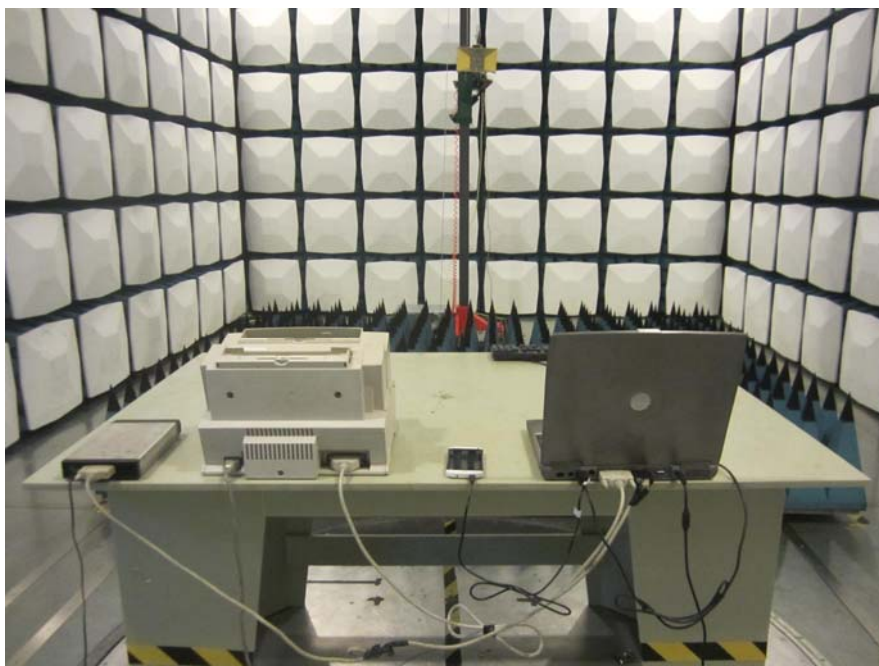
Radiated Emissions –Rear View (Above 1GHz) (USB Downloading)
