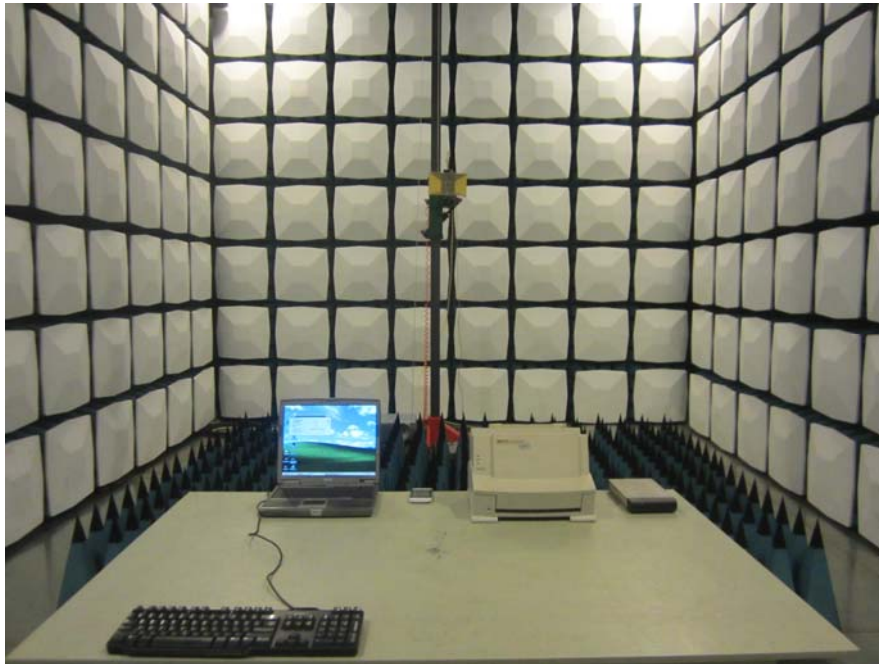
Radiated Emissions –Front View (Above 1GHz) (USB Downloading)
