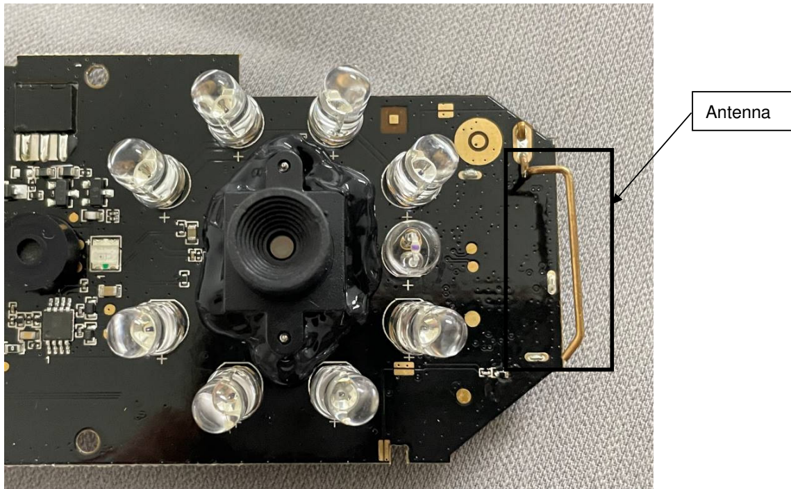
Photo of antenna refer to Appendix – Internal photo.
