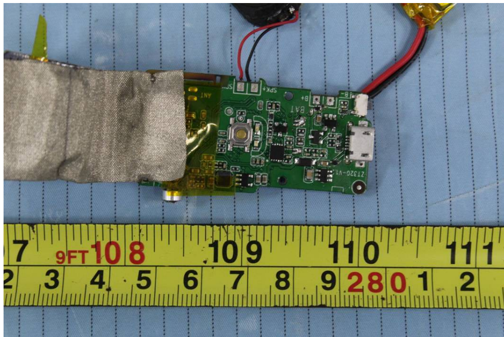
EUT – Main Board Top 1 View
