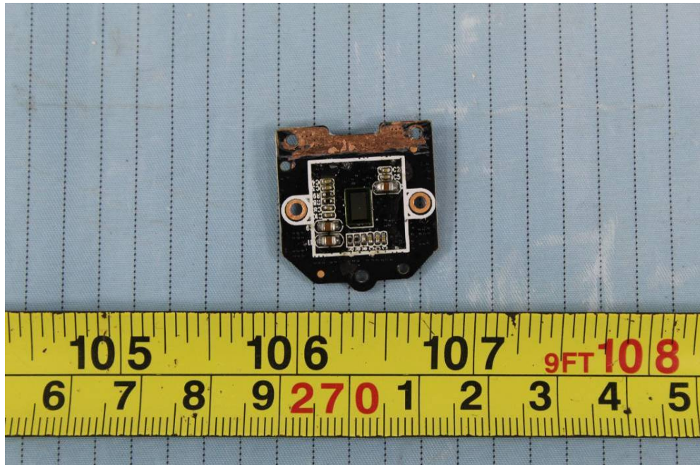
EUT – Sensor Board Top View
