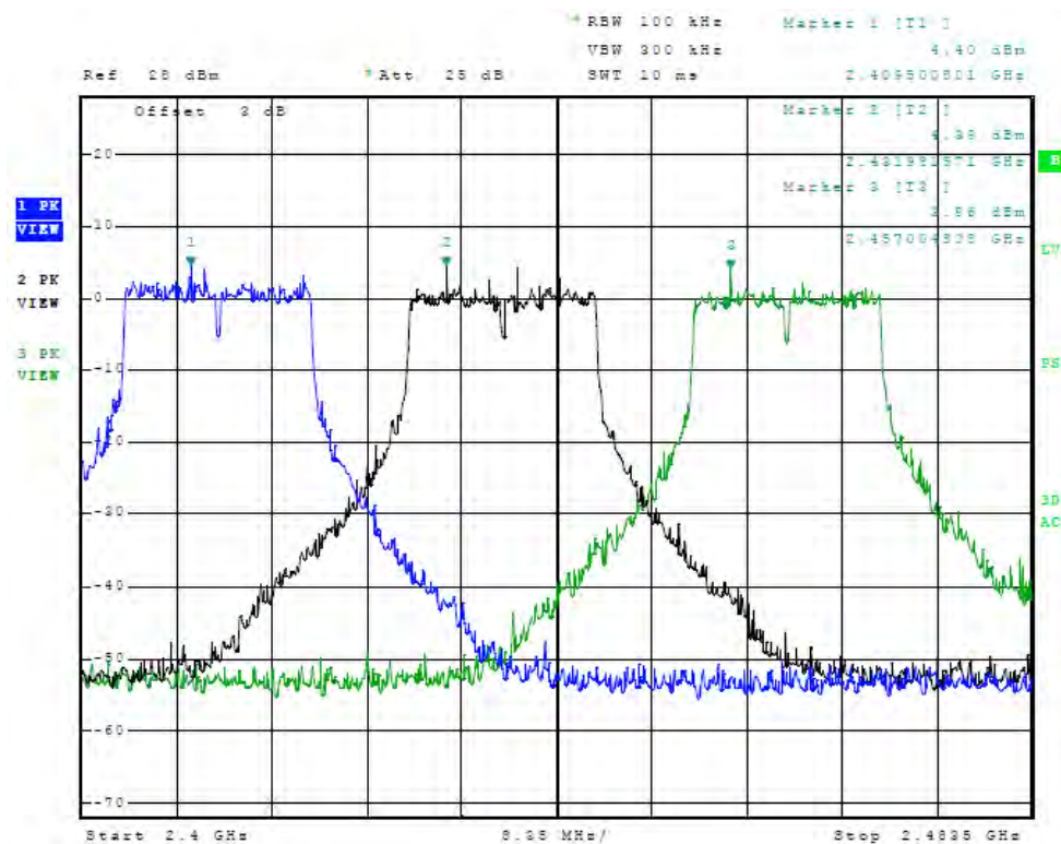
Figure 72 Plot of Antenna Port Conducted (2GHz, chain2, Operational Band, 20MHz Mode)
