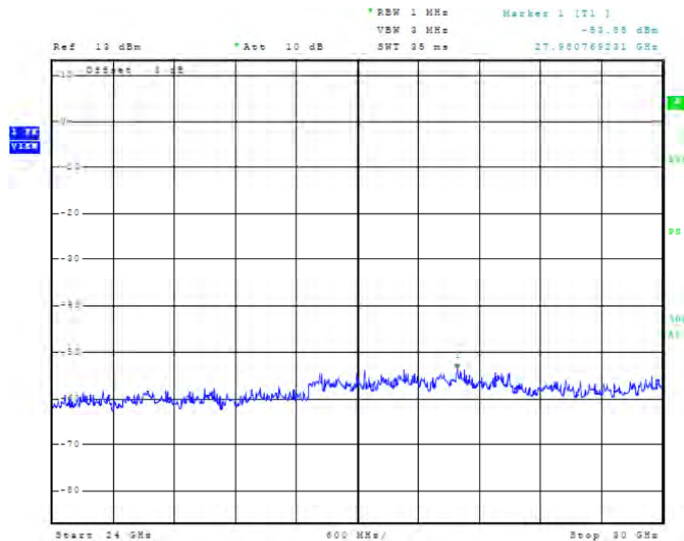
Figure 67 Plot of Antenna Port Conducted Emissions (5 GHz, chain 1, operation)
