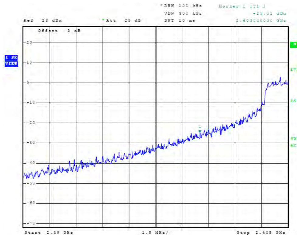
Figure 97 Plot of Low Band Edge Compliance at Antenna Port (chain2, 2.4MHz Operation)
