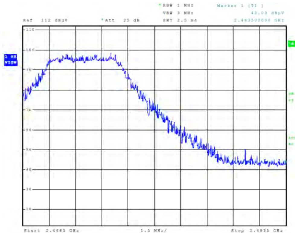
Figure 130 Plot of Radiated Emissions at High Band Edge
