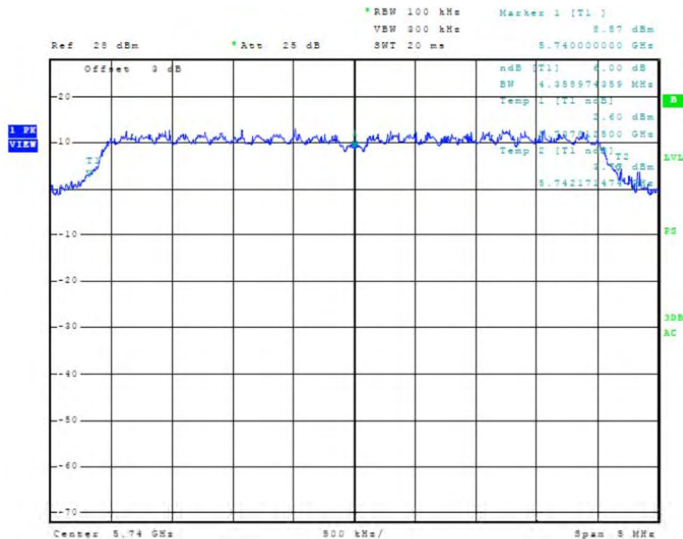
Figure 43 Plot of Antenna Port Conducted 6dB Band width (chain 1, 5740 MHz, 5 MHz Mode)
