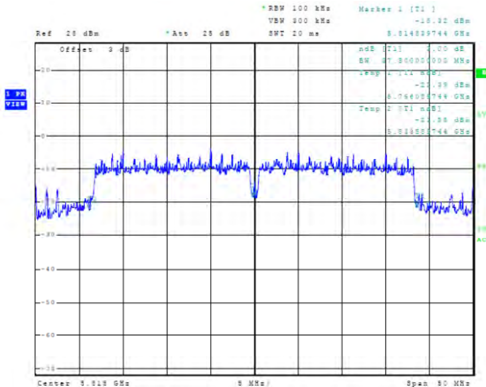
Figure 110 Plot of Antenna Port Conducted 6dB Band width (chain2, 5815 MHz, 40 MHz Mode)
