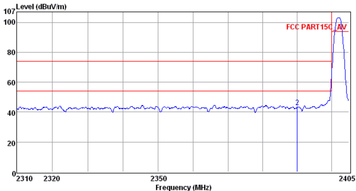
Test plot of Restricted Bands-Bluetooth LE Low channel(Horizontal)
