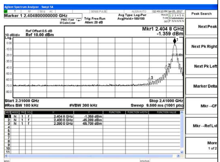
Zigbee-Low channel
