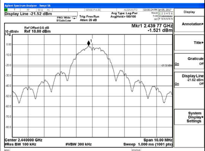
Zigbee-Middle channel
