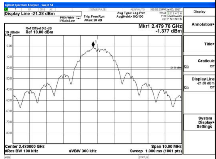
Zigbee-High channel
