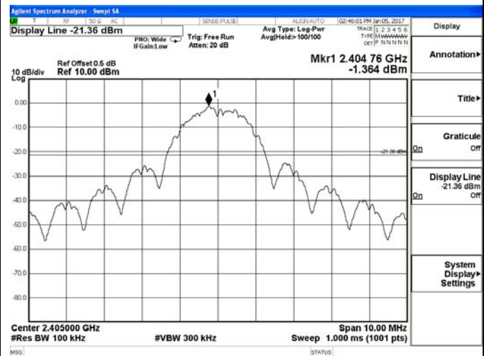
Zigbee-Low channel
