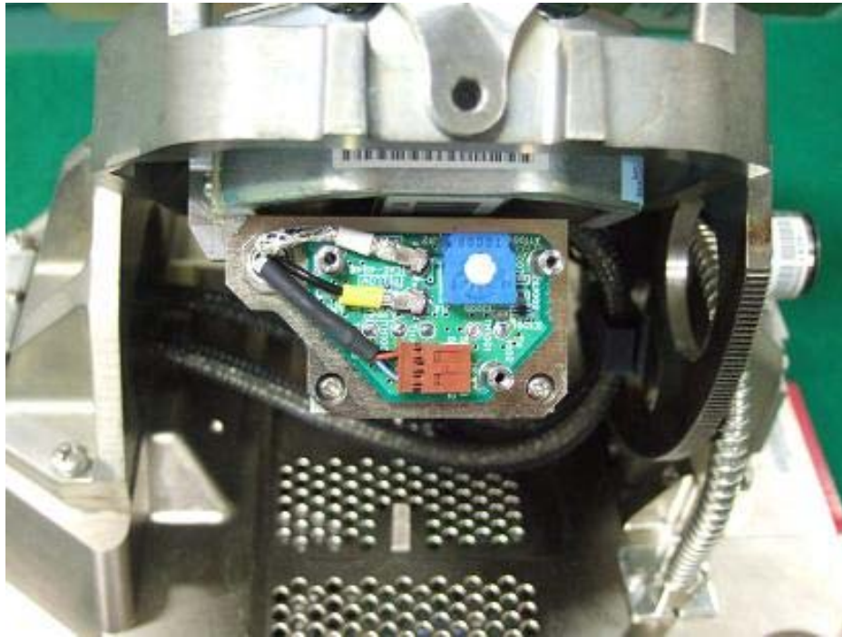
IF AMP Top view (Cover removed)
