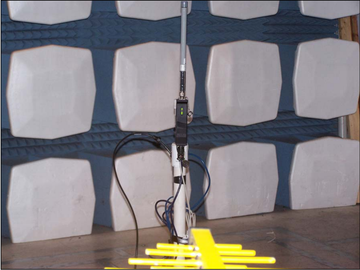
Photograph 2. Radiated Emissions, 15B, AC/DC Power Supply
