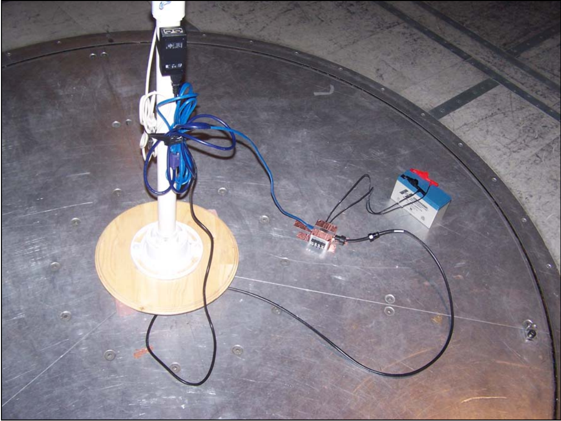
Photograph 3. Radiated Emissions, 15B, DC/DC Power Supply
