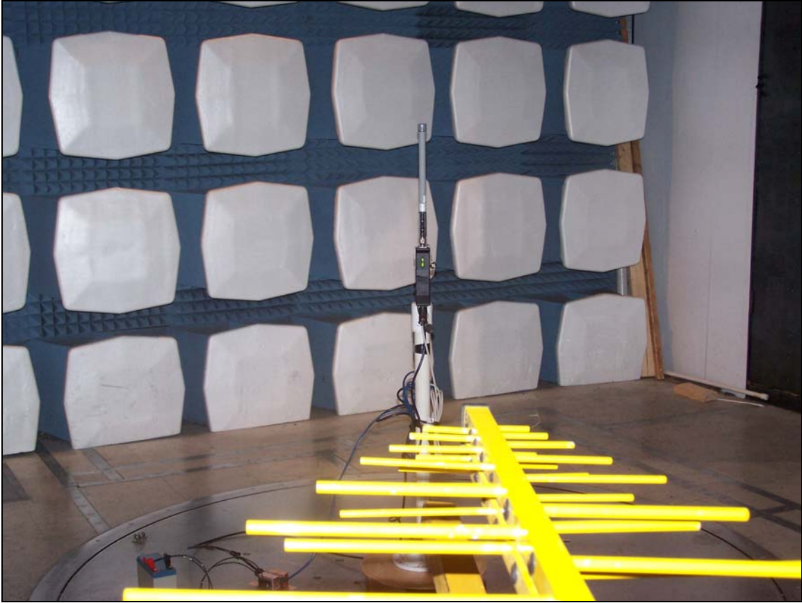
Photograph 4. Radiated Spurious Emissions Below 1 GHz
