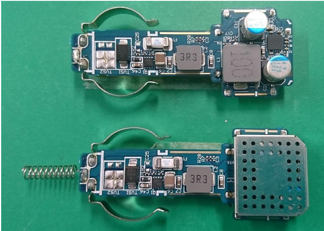
DC/DC Board with / without shield case
