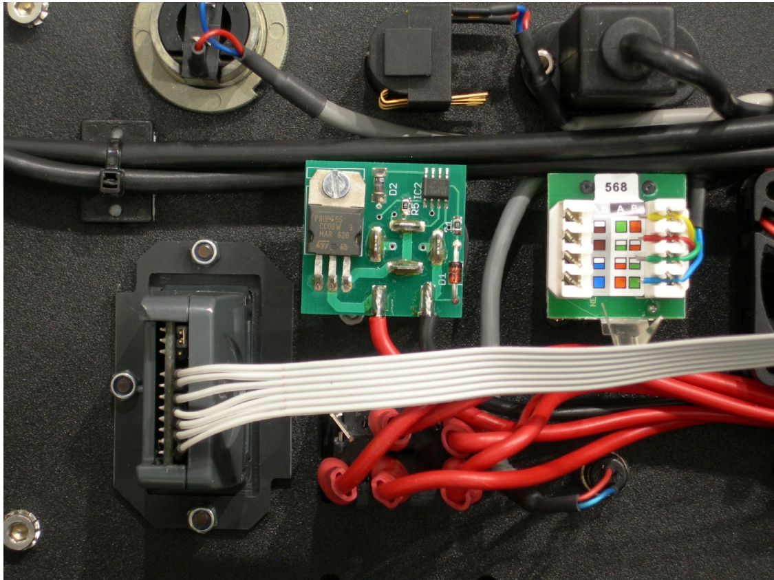
Figure 3 Over voltage protection PCB mounting
