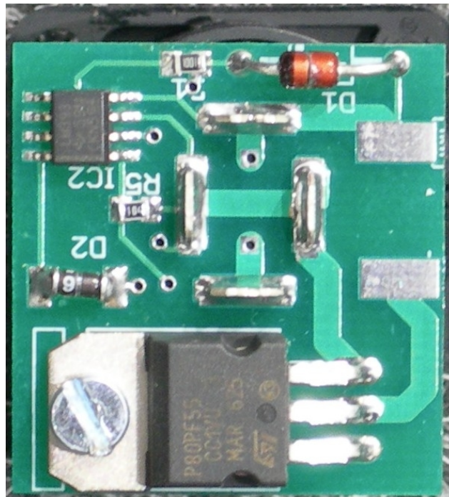
Figure 1 OV Protect 1.0 Bottom view
