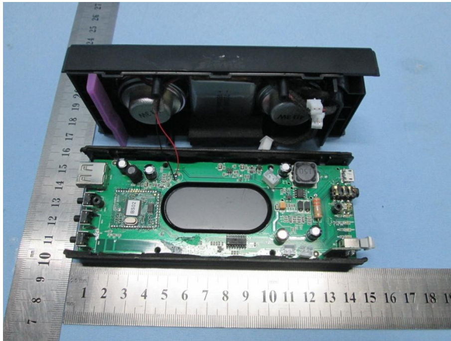
Figure 1 EUT Internal Photo
