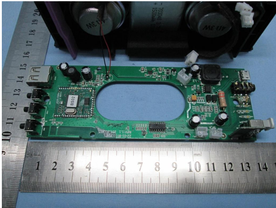
Figure 7 EUT Internal Photo (for model BT1140CUS)
