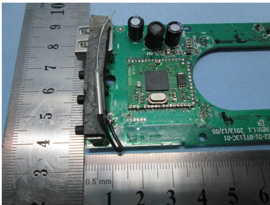
Figure 10 EUT Internal Photo (for model BT1130CUS)
