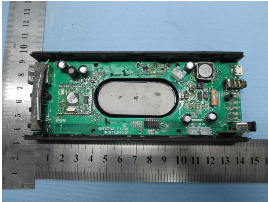
Figure 9 EUT Internal Photo (for model BT1130CUS)
