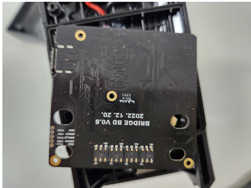
Connect Board - Rear Bottom
