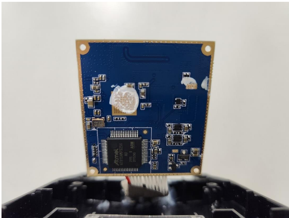
Main board - Rear Bottom
