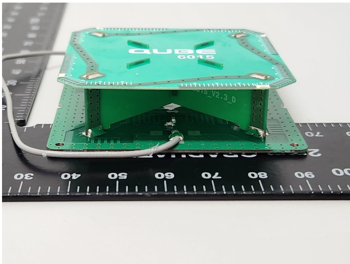
PCB Antenna
