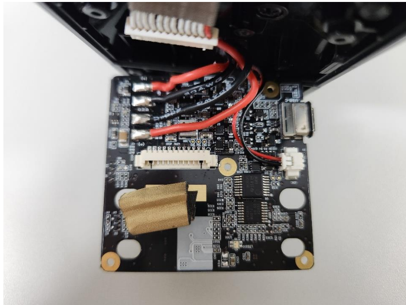
Connect Board -Front Top
