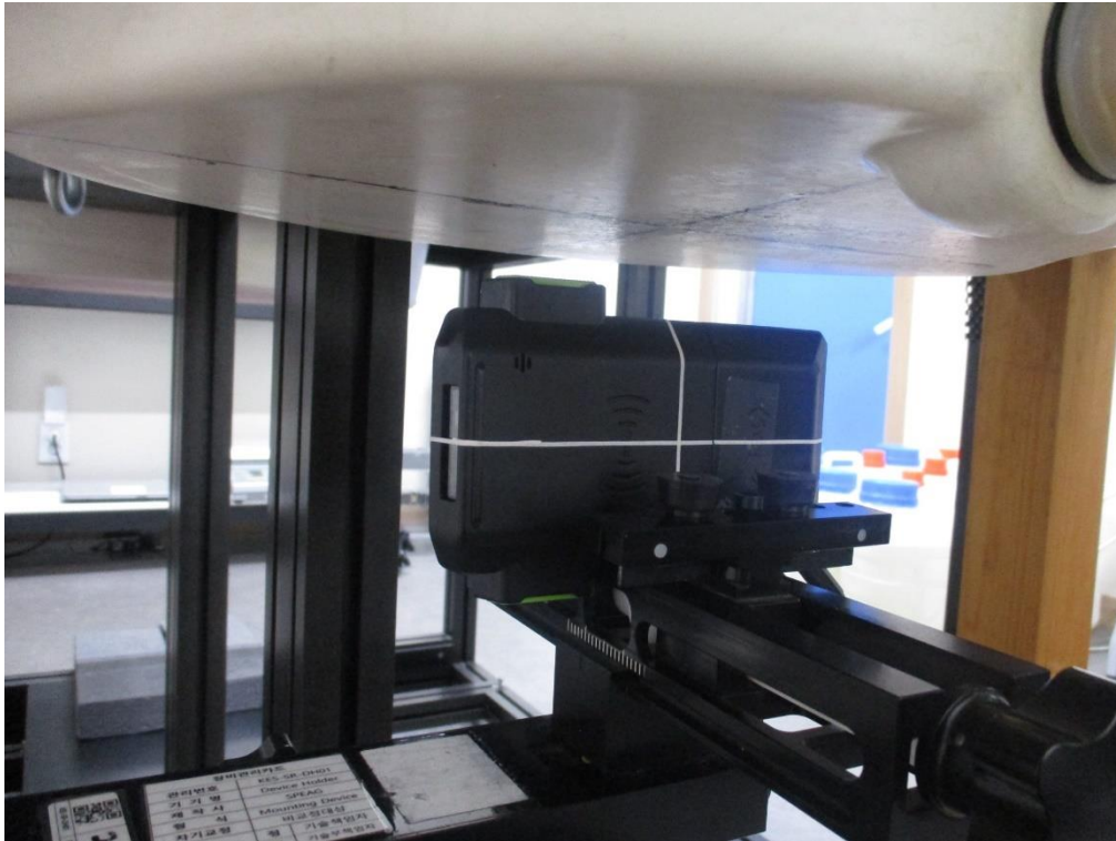
Right Side from Flat Phantom (Separation Distance: 2.5 cm) – Body SAR
