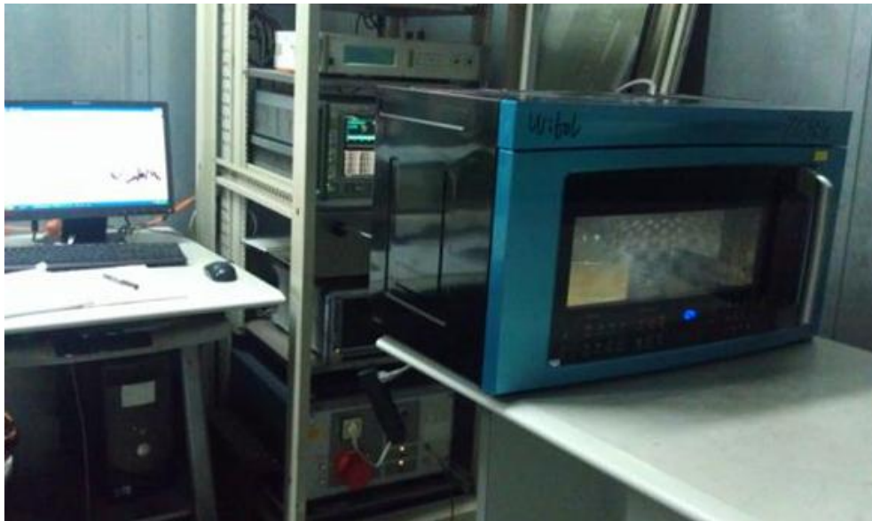
Conducted Emission Test Set-up
