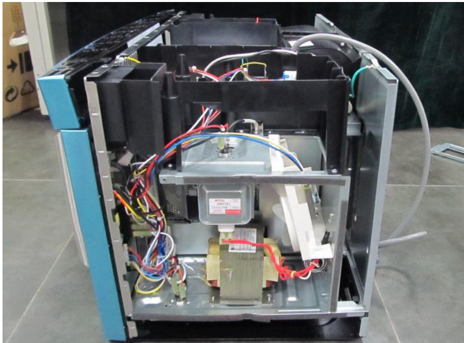
EUT Uncovered View #2
