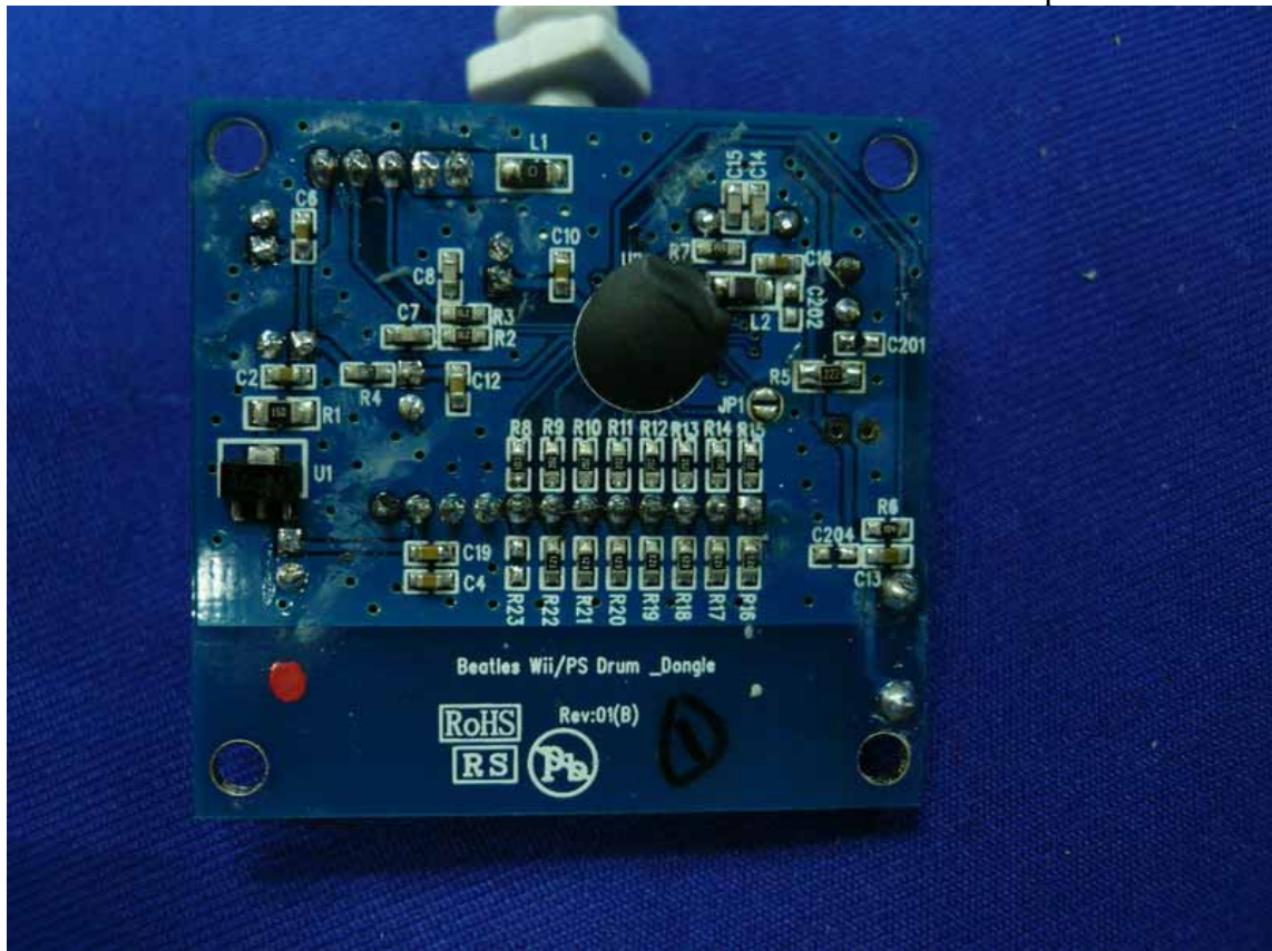
Figure 5 Component side of the EUT
