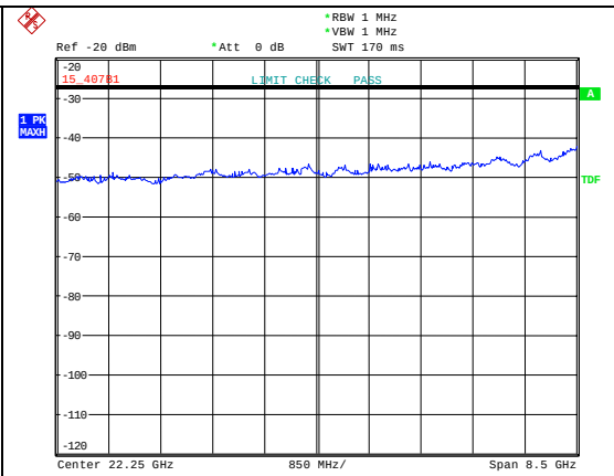
CH 36 18 - 26 GHz vertical polarization
