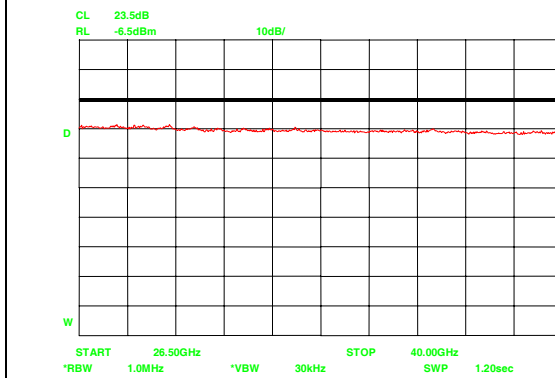
CH 36 26 - 40 GHz horizontal polarization
