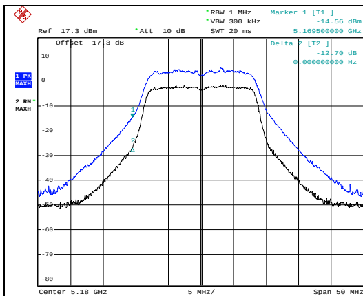
Channel 36: max. peak excursion is 12.70 dB
