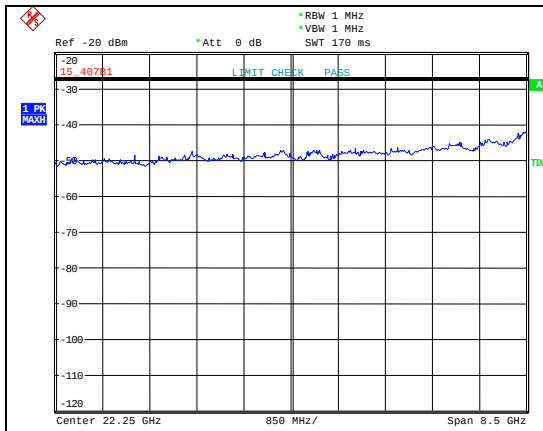
CH 36 18 - 26 GHz horizontal polarization
