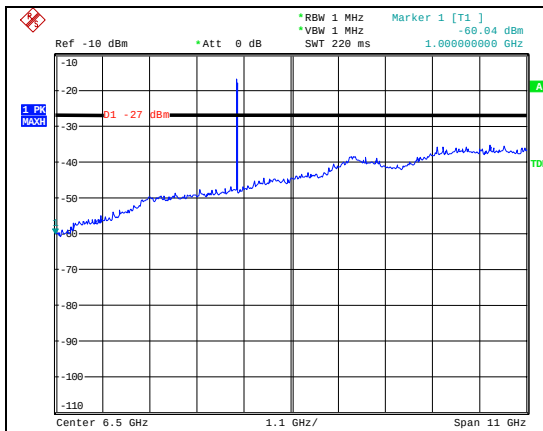
CH 48 1 - 12 GHz horizontal polarization
