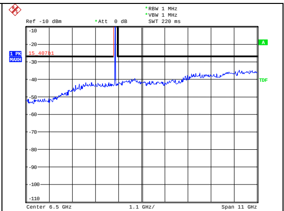
CH 48 1 - 12 GHz vertical polarization
