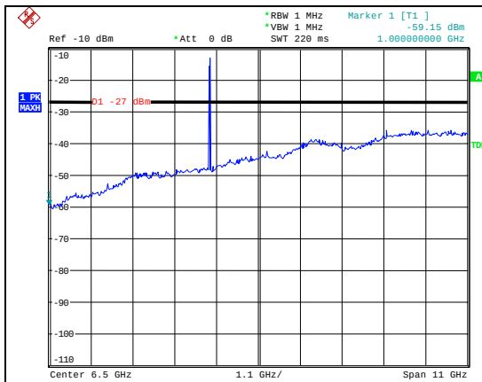
CH 44 1 - 12 GHz horizontal polarization
