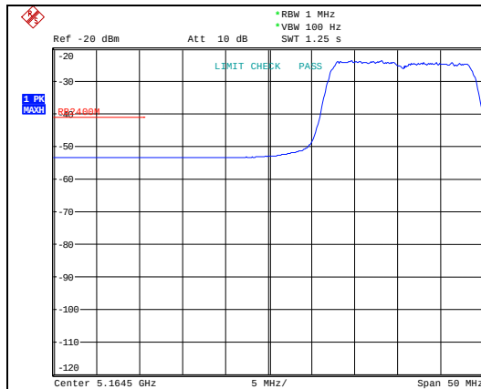
Lower band Channel 36 Polarization horizontal
