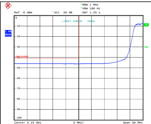
Lower band Channel 36 Polarization vertical
