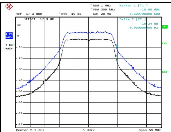
Channel 40: max. peak excursion is 10.24 dB
