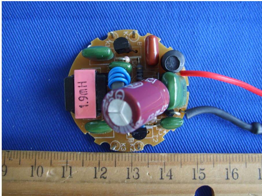
EUT –Components View (MS13W)
