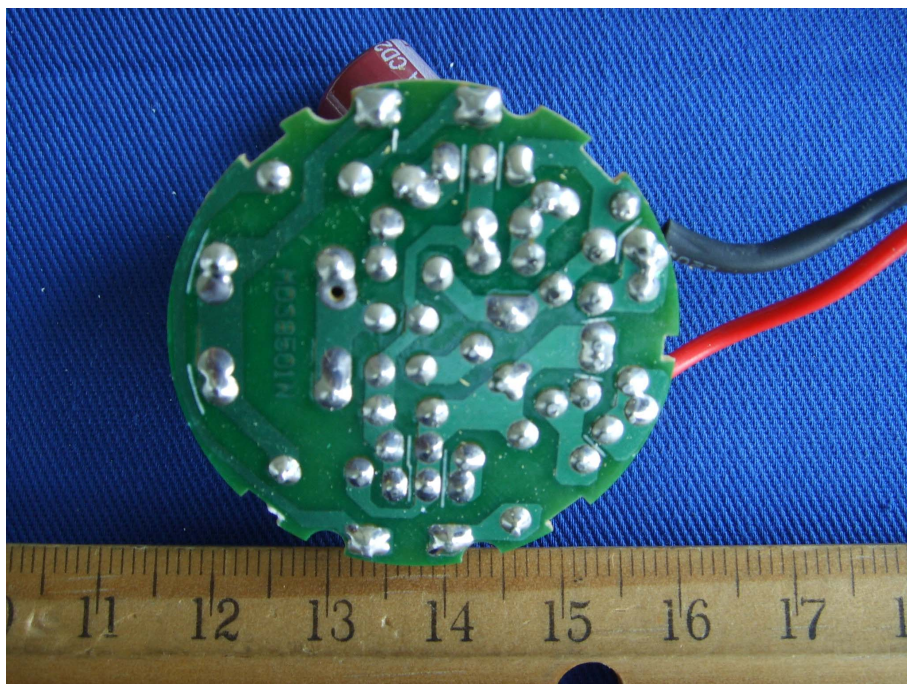
EUT–Solder View (MS13W)
