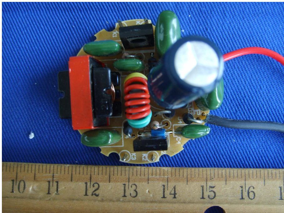
EUT –Components View (MS15W)
