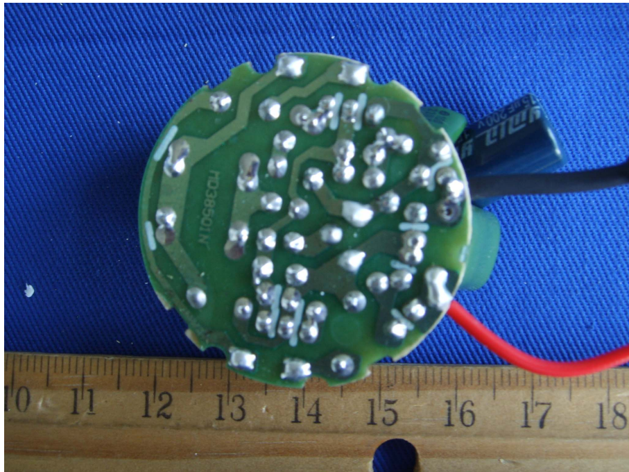
EUT–Solder View (MS15W)
