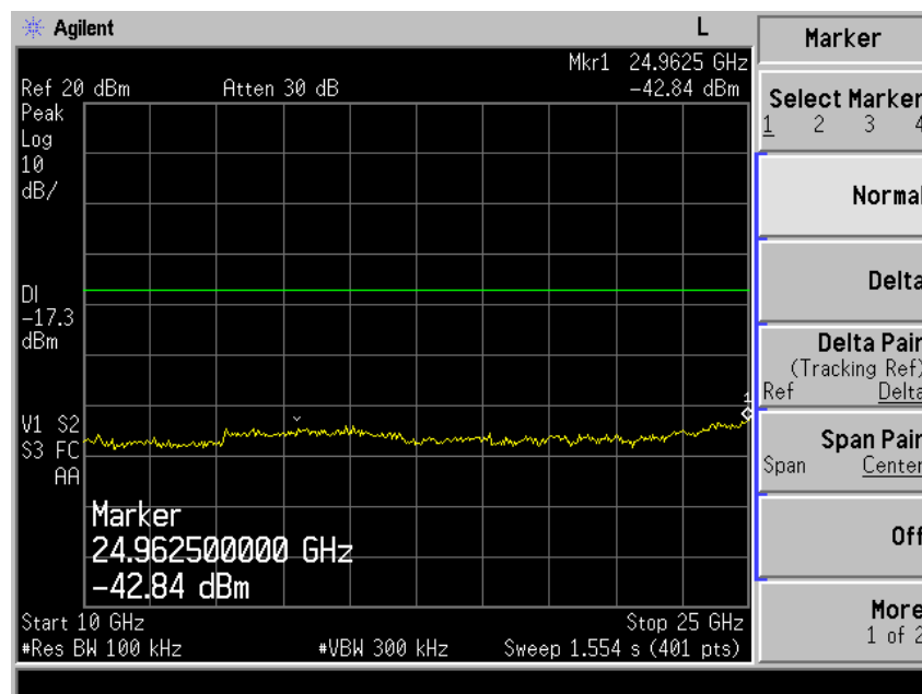
Plot 17 – Channel 39
