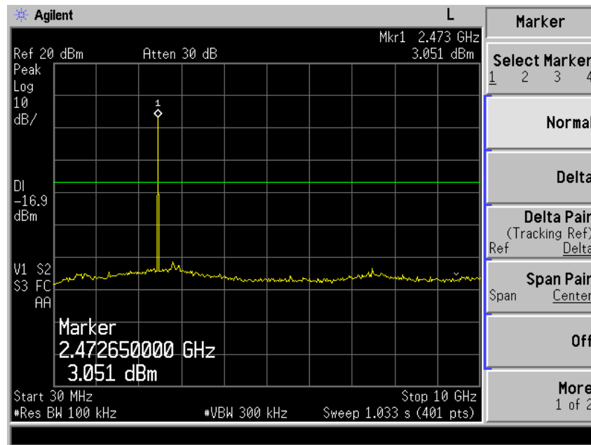
Plot 18 – Channel 78
