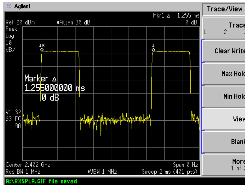
Plot 11 – Channel 0
