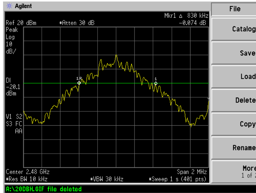
Plot 6 – Channel 78
