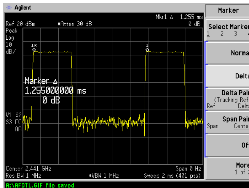
Plot 12 – Channel 39
