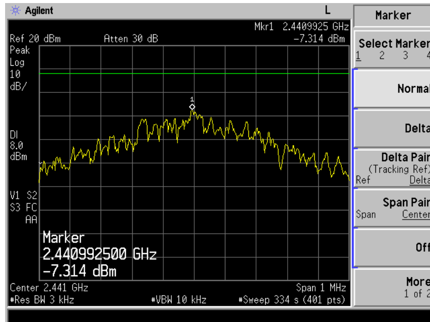
Plot 29 – Channel 39
