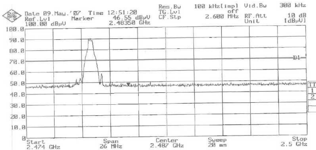
Plot 23 – Upper Band Edge at 2.4835GHz
