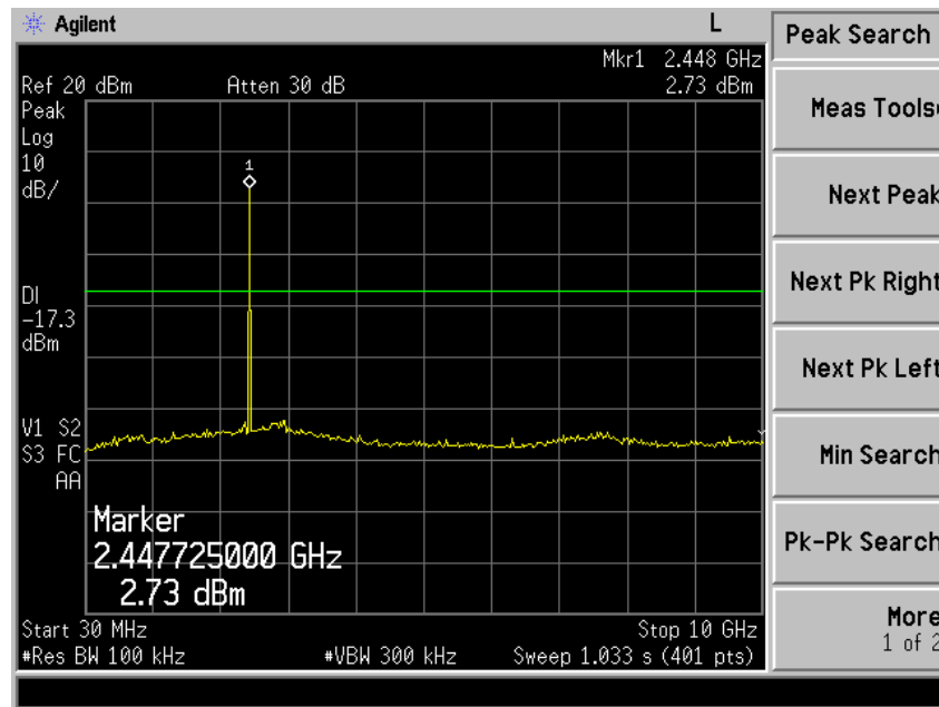
Plot 16 – Channel 39
