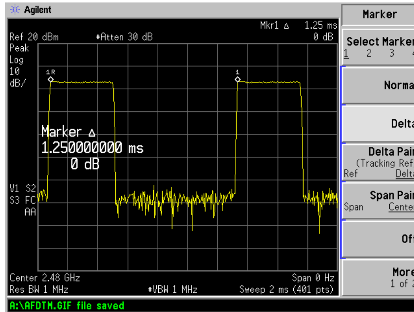
Plot 13 – Channel 78
