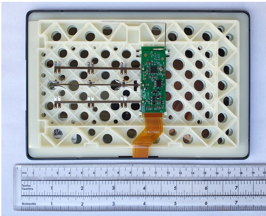
DD74-3A (Chroma Aeon 74) – Rear View, Rear Cover, Battery Cover and Coin cells removed.
