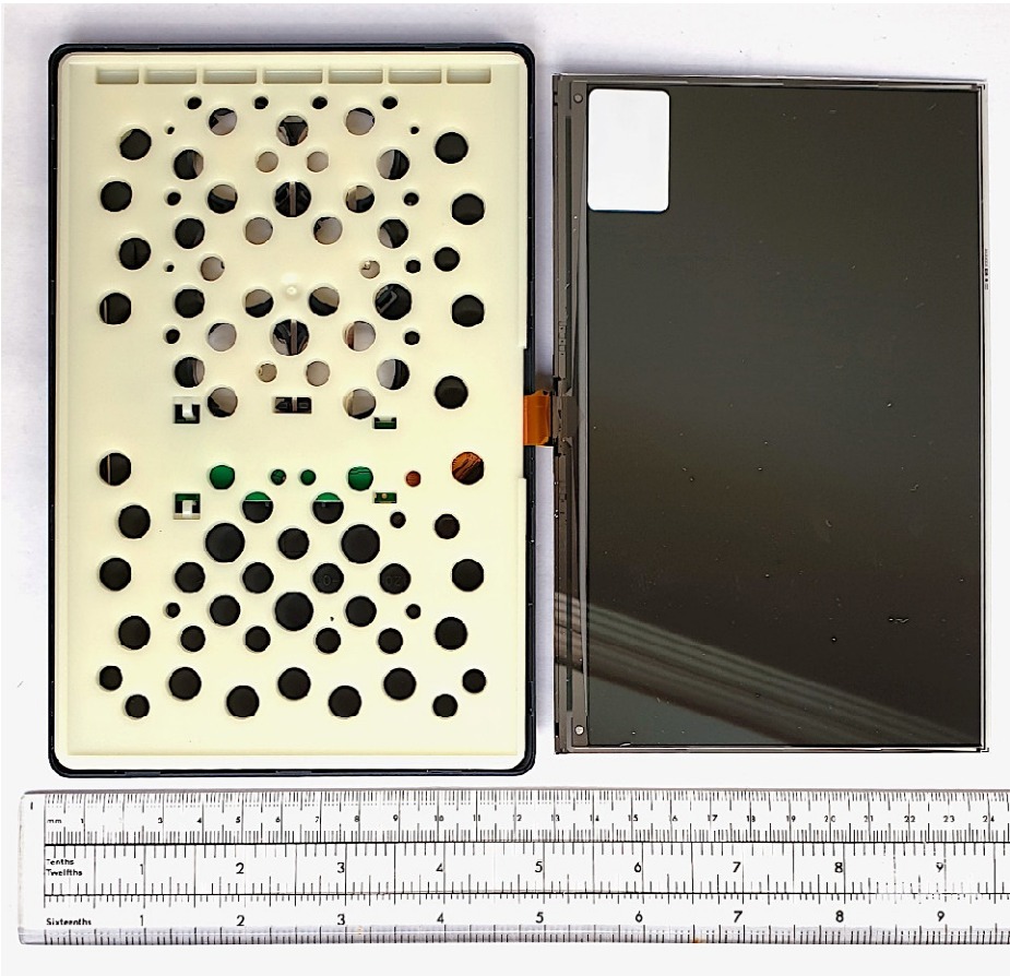
DD74-3A (Chroma Aeon 74) – Front View, with Front Cover removed and display “flipped” to reveal PCB.
