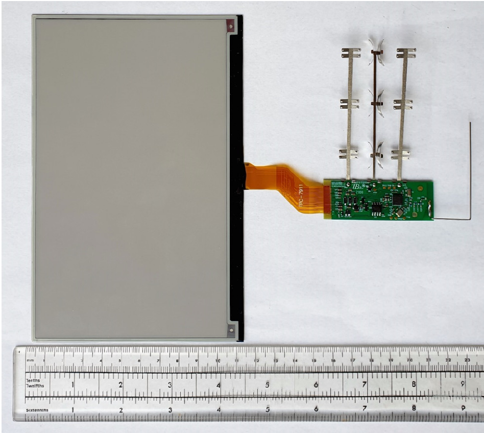
DD74-3A (Chroma Aeon 74) – PCB and Display Glass Front View.
