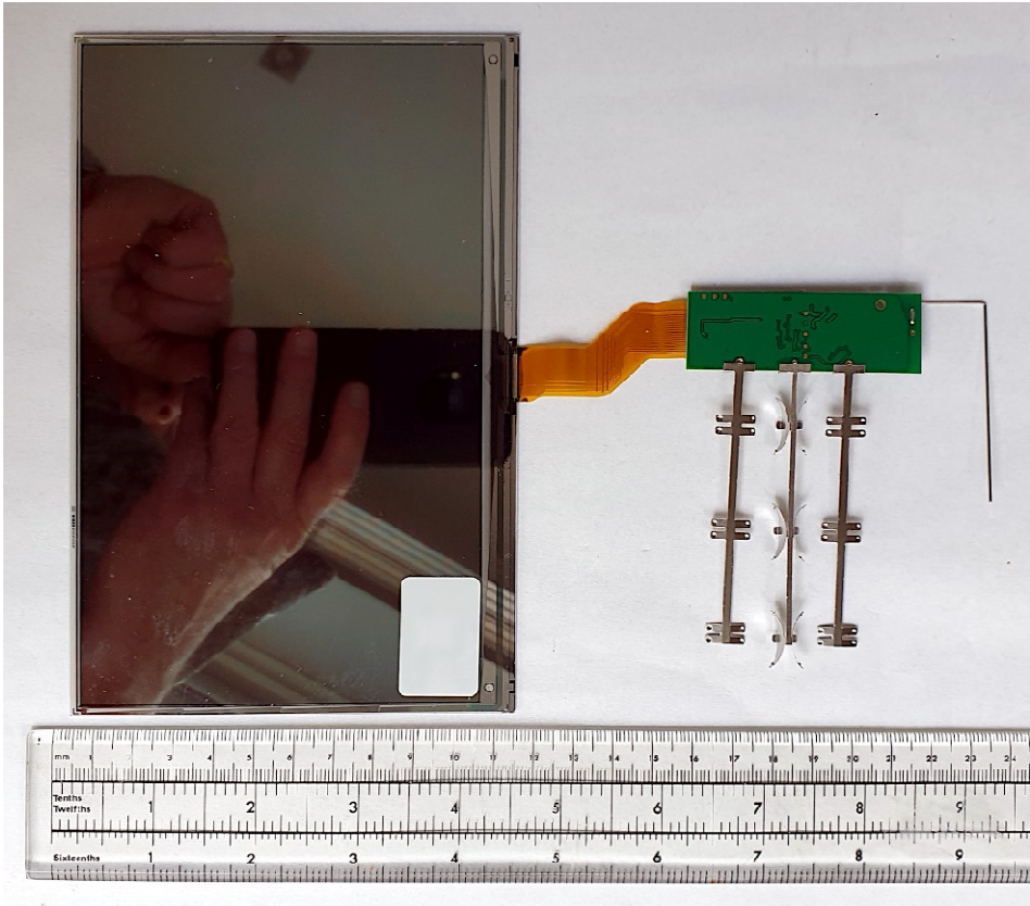
DD74-3A (Chroma Aeon 74) – PCB and Display Glass Rear View.
