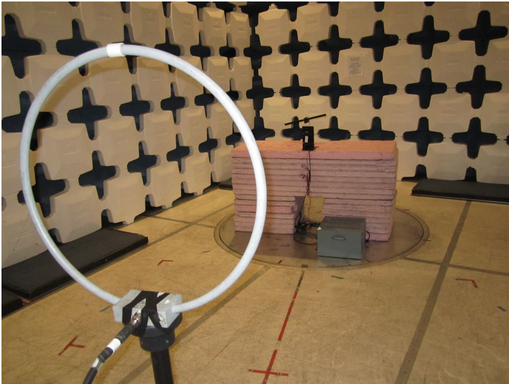
125kHz RFID Fundamental, Radiated Emissions 9kHz-1MHz
