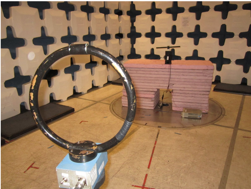
13.56MHz RFID Fundamental, Radiated Emissions 1-30MHz
