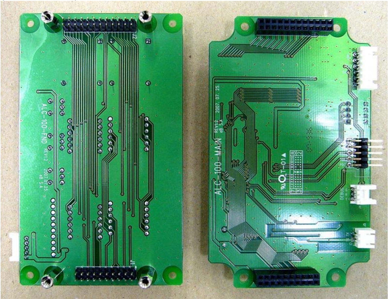
(ALC-100 Bottom)
