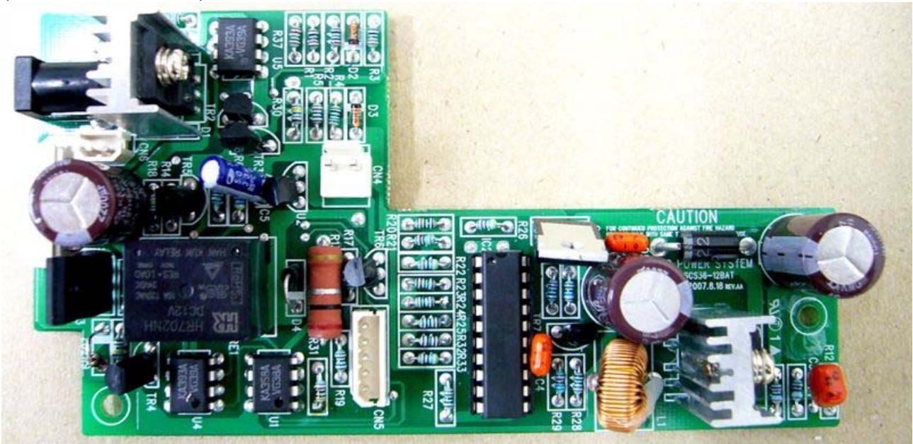
(SCS36-12BAT TOP)
