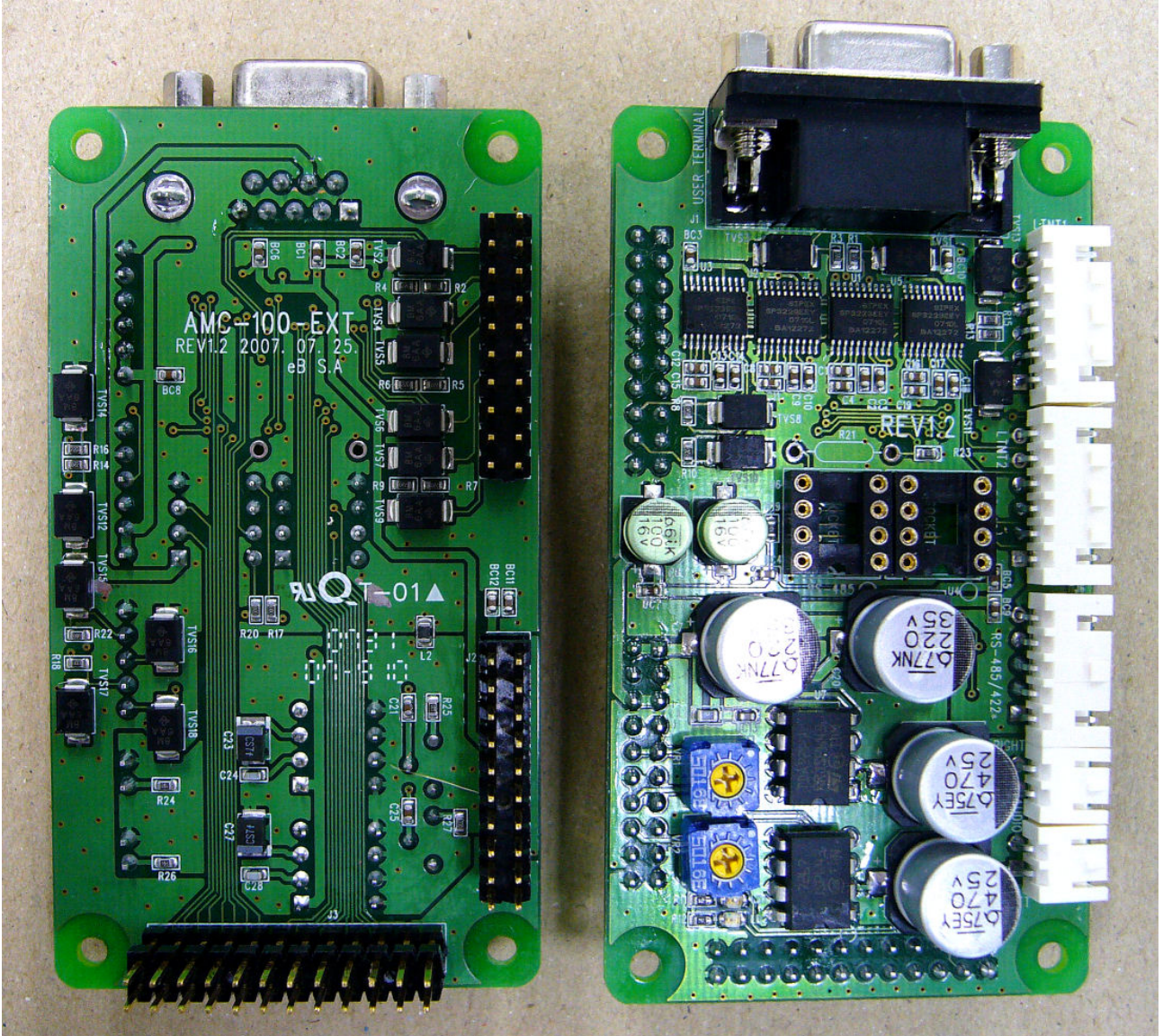
(AMC-100 Ext)
