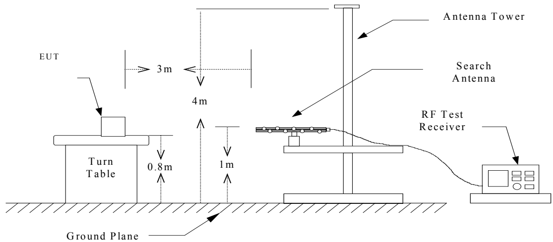
Figure 1: Frequencies measured 30MHz ~ 1GHz configuration
