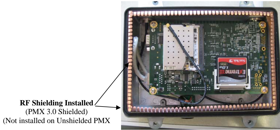
Figure #5: PMX 3.0 Internal Configuration (Top View of circuit board)
