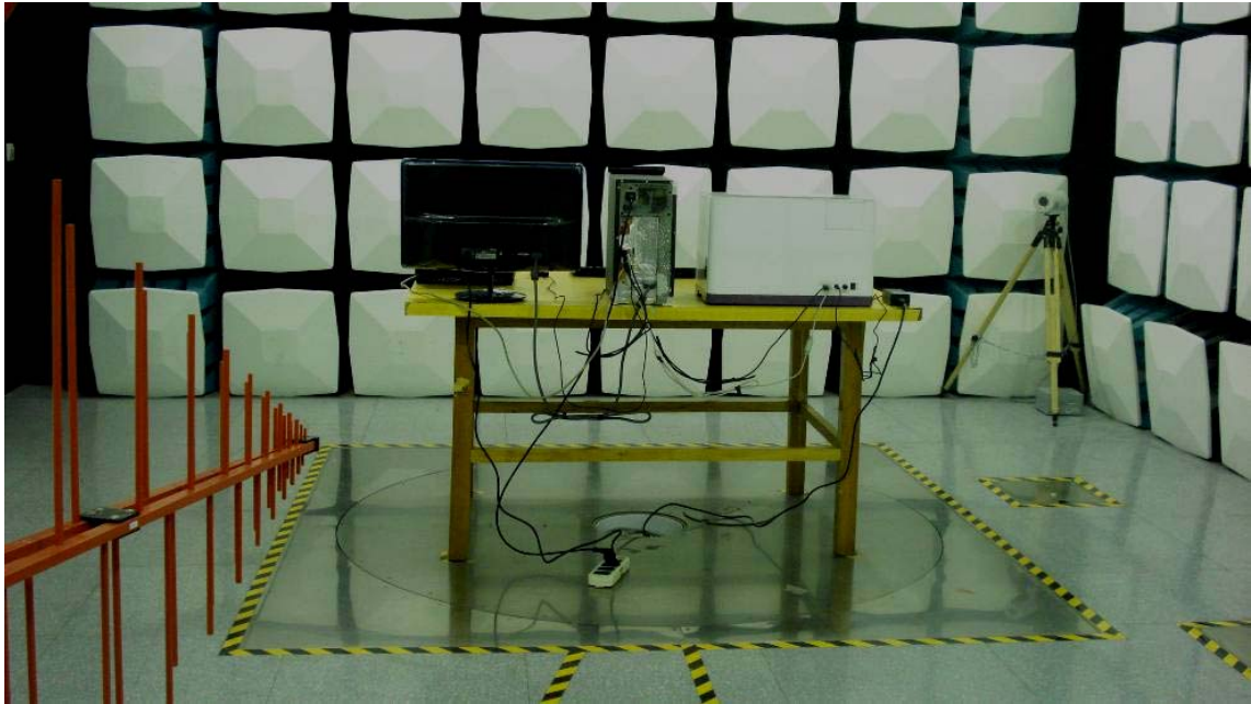
Radiated Emission Test Setup - Rear View
