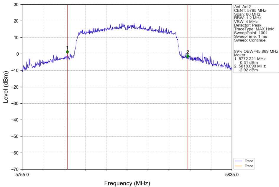
802.11ax(HEW40)_HCH_5795MHz_SU_ / _Ant2_NTNV
