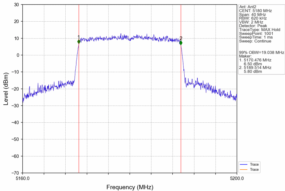
802.11ax(HEW20)_LCH_5180MHz_SU_ / _Ant2_NTNV
