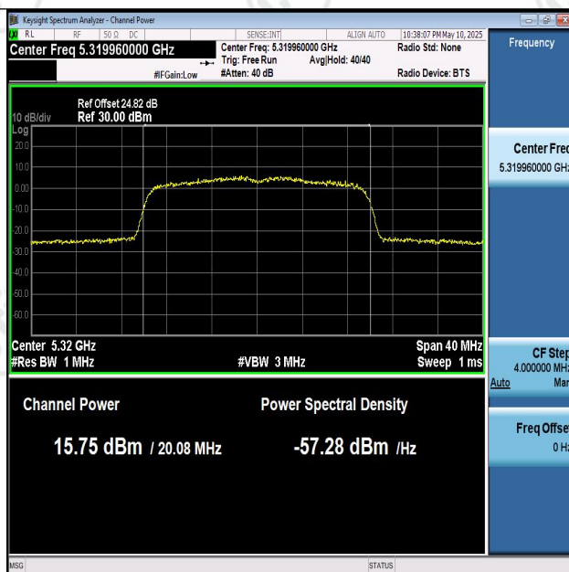
11AX20MIMO-Ant2-5320-PASS
