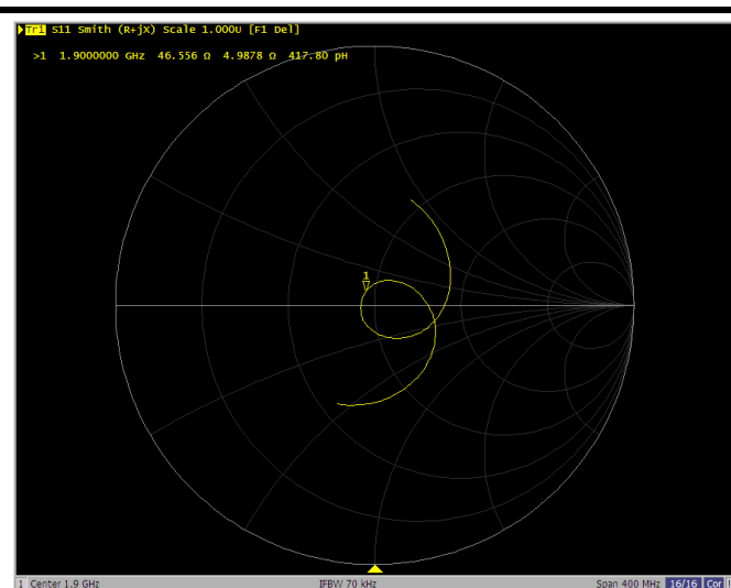
1900 MHz, Body TSL
