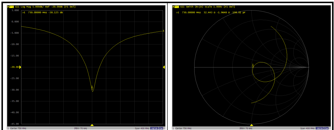
750 MHz, Head TSL
