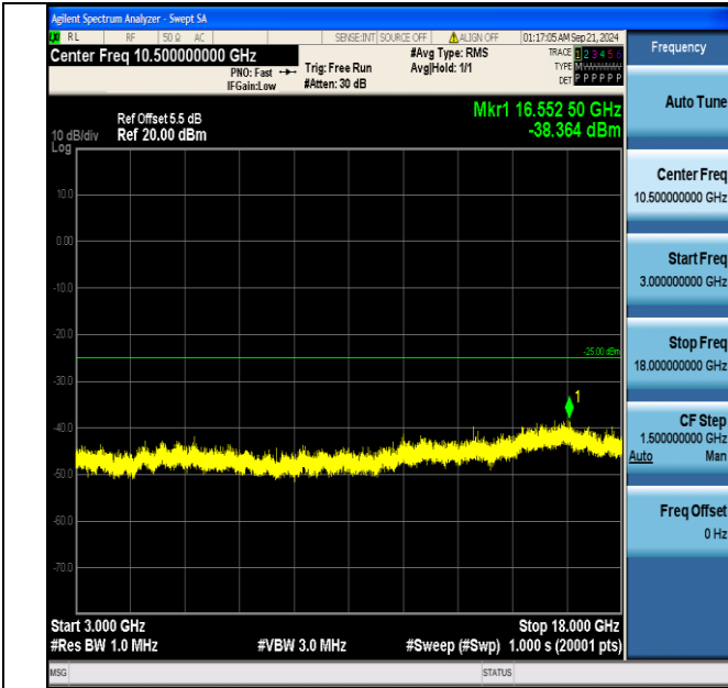
Band7_20MHz_QPSK_21350_1RB#99_3000~18000_3000~18000
