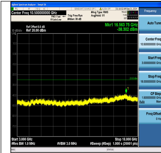
Band7_20MHz_QPSK_21350_1RB#0_3000~18000_3000~18000
