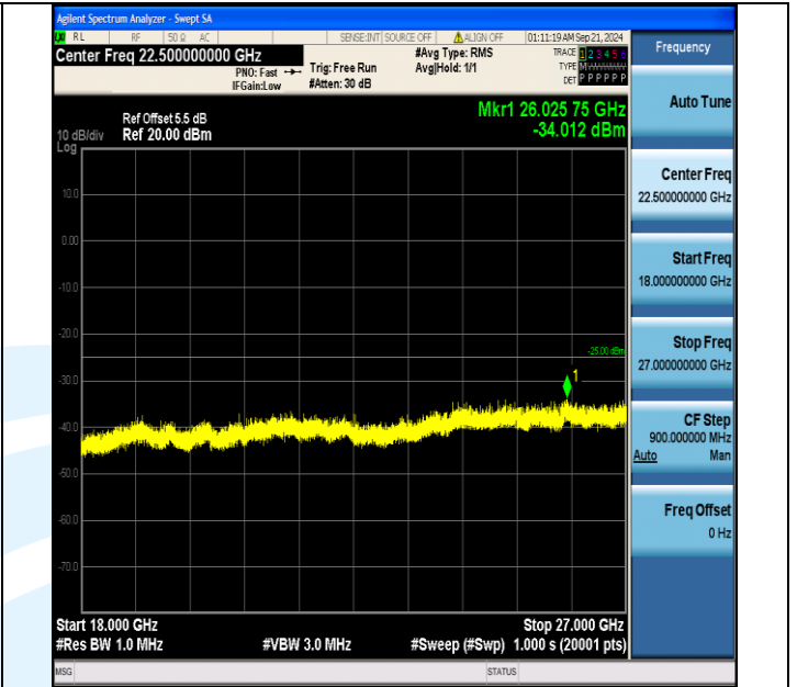
Band7_20MHz_16QAM_20850_1RB#99_18000~27000_18000~27000
