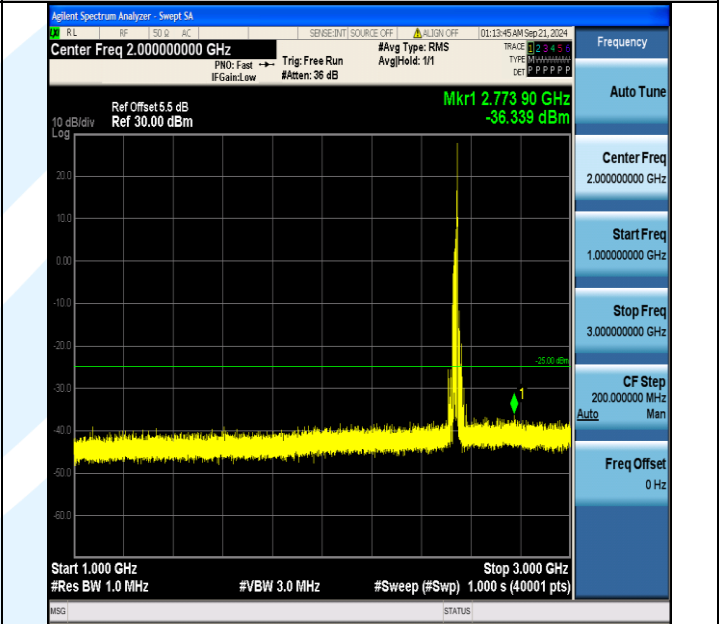
Band7_20MHz_QPSK_21100_1RB#99_1000~3000_1000~3000
