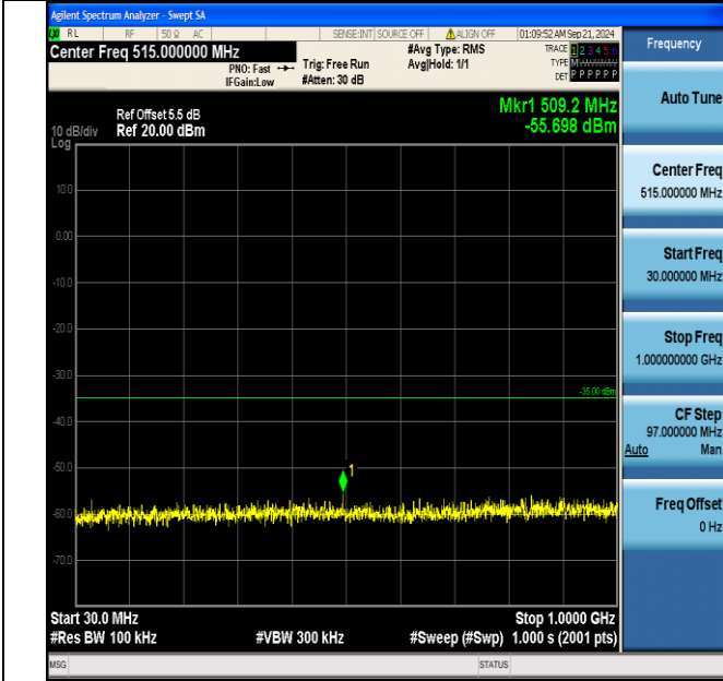
Band7_20MHz_16QAM_20850_1RB#0_30~1000_30~1000
