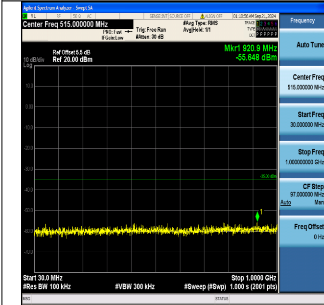
Band7_20MHz_16QAM_20850_1RB#99_30~1000_30~1000
