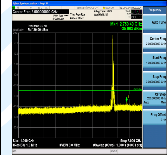
Band7_20MHz_QPSK_21100_1RB#0_1000~3000_1000~3000
