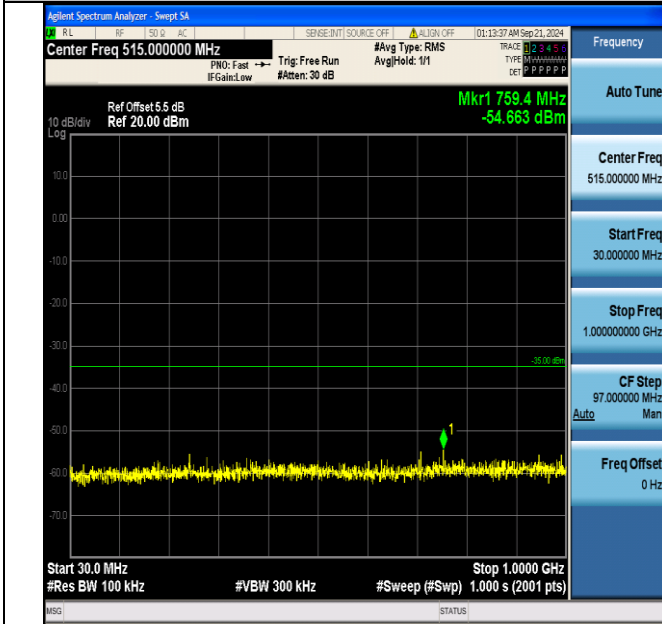
Band7_20MHz_QPSK_21100_1RB#99_30~1000_30~1000
