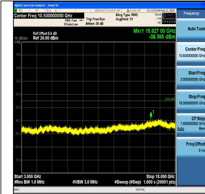
Band7_20MHz_QPSK_21100_1RB#99_3000~18000_3000~18000
