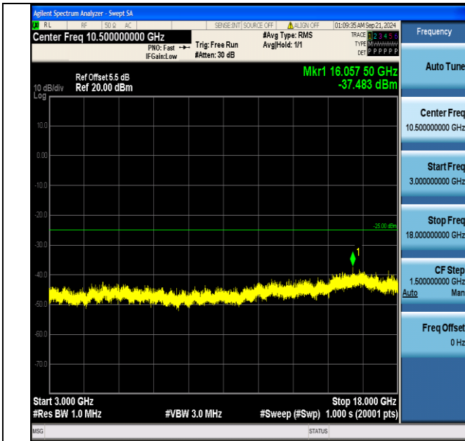
Band7_20MHz_QPSK_20850_1RB#0_3000~18000_3000~18000
