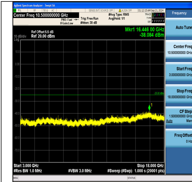
Band7_20MHz_16QAM_20850_100RB#0_3000~18000_3000~18000
