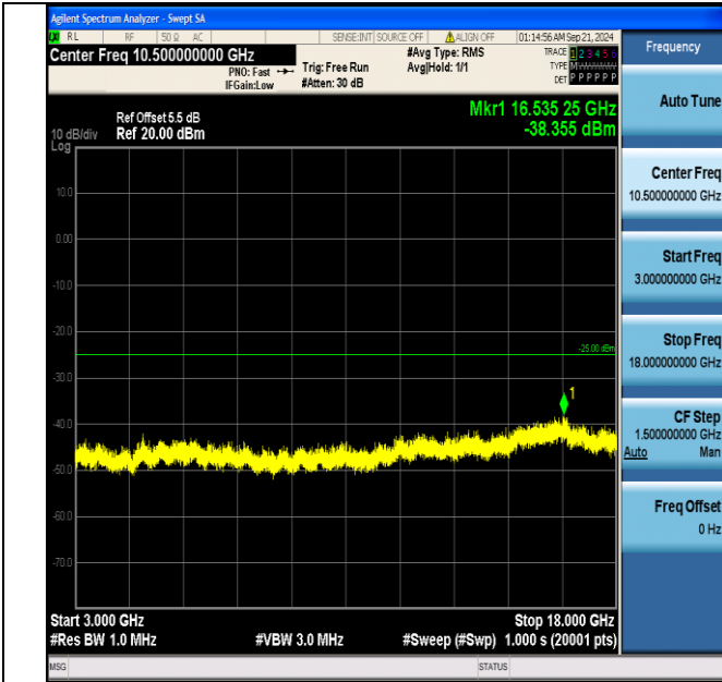
Band7_20MHz_QPSK_21100_100RB#0_3000~18000_3000~18000
