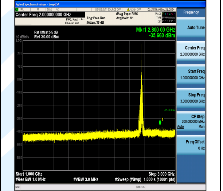
Band7_20MHz_QPSK_21350_1RB#0_1000~3000_1000~3000
