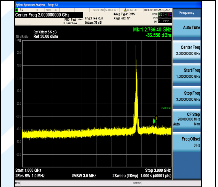
Band7_20MHz_16QAM_21100_1RB#0_1000~3000_1000~3000
