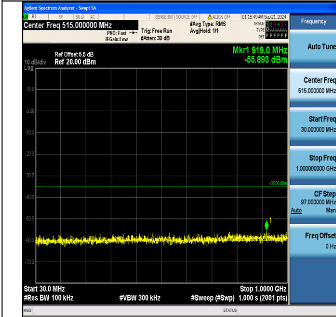
Band7_20MHz_QPSK_21350_1RB#99_30~1000_30~1000
