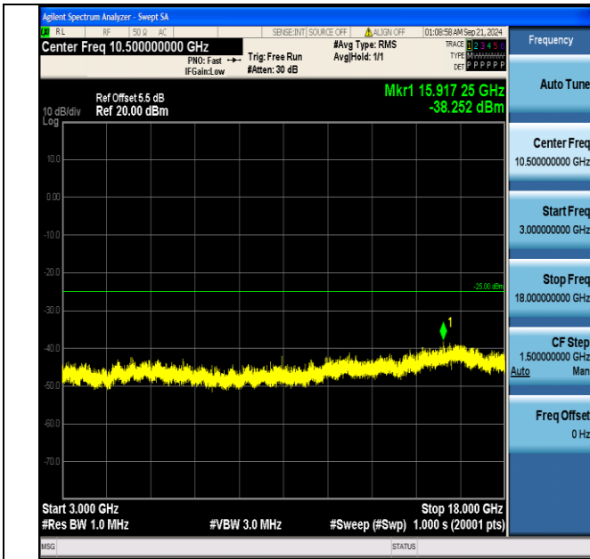
Band7_15MHz_16QAM_21375_75RB#0_3000~18000_3000~18000
