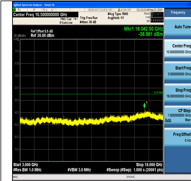
Band7_20MHz_16QAM_21100_1RB#0_3000~18000_3000~18000
