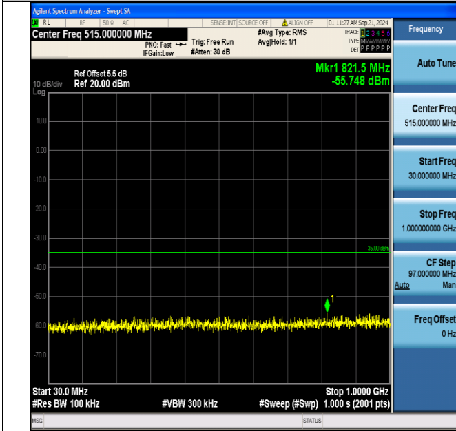
Band7_20MHz_QPSK_20850_100RB#0_30~1000_30~1000
