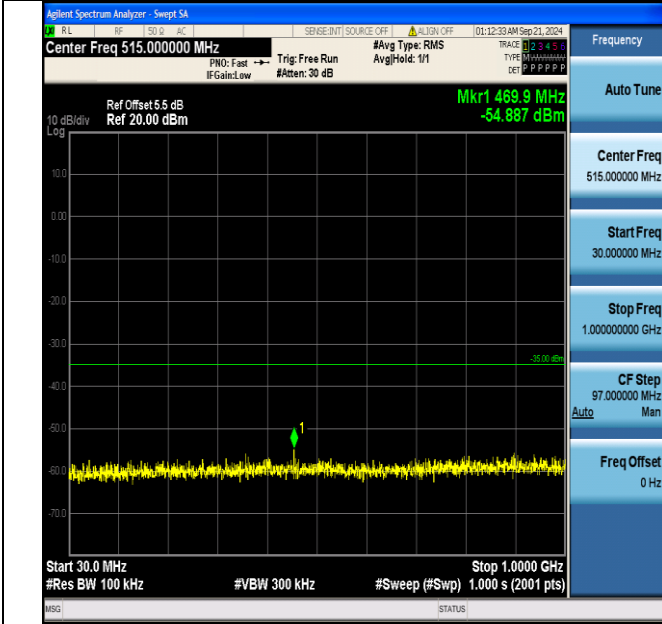
Band7_20MHz_QPSK_21100_1RB#0_30~1000_30~1000
