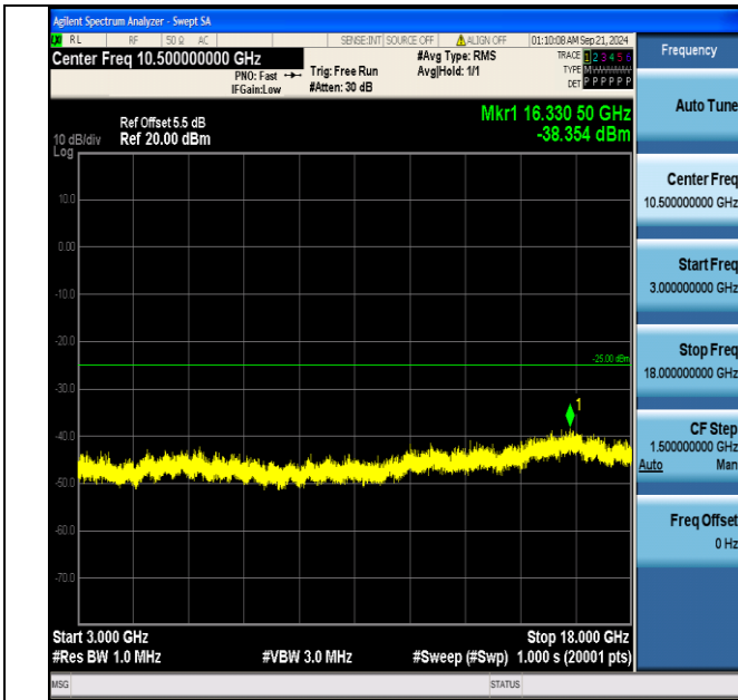
Band7_20MHz_16QAM_20850_1RB#0_3000~18000_3000~18000
