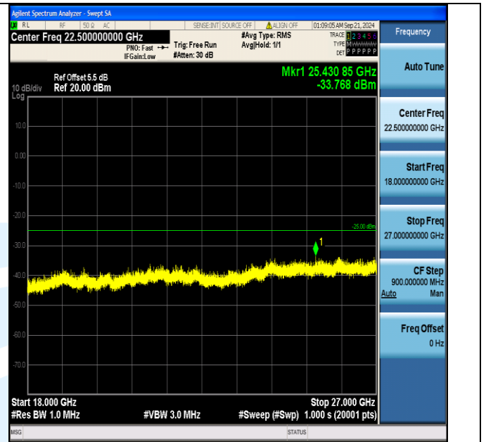
Band7_15MHz_16QAM_21375_75RB#0_18000~27000_18000~27000
