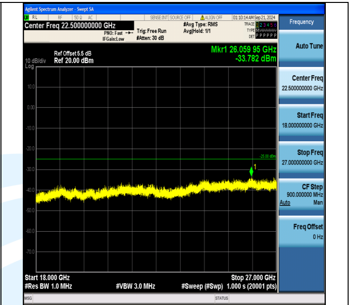
Band7_20MHz_16QAM_20850_1RB#0_18000~27000_18000~27000
