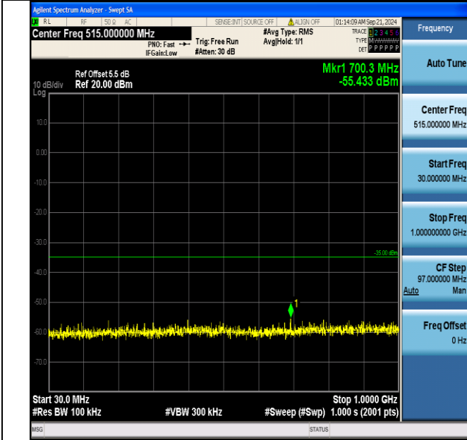
Band7_20MHz_16QAM_21100_1RB#99_30~1000_30~1000
