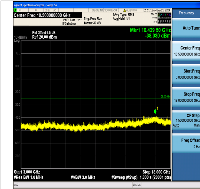
Band7_20MHz_16QAM_20850_1RB#99_3000~18000_3000~18000
