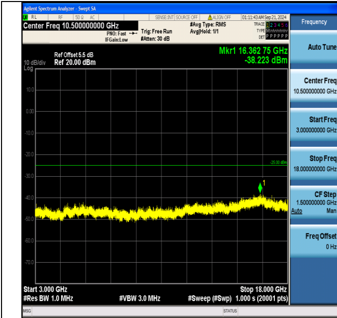
Band7_20MHz_QPSK_20850_100RB#0_3000~18000_3000~18000
