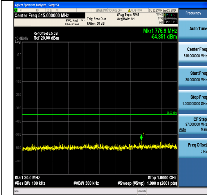
Band7_20MHz_QPSK_20850_1RB#99_30~1000_30~1000
