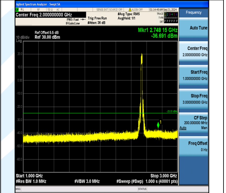
Band7_20MHz_QPSK_21100_100RB#0_1000~3000_1000~3000
