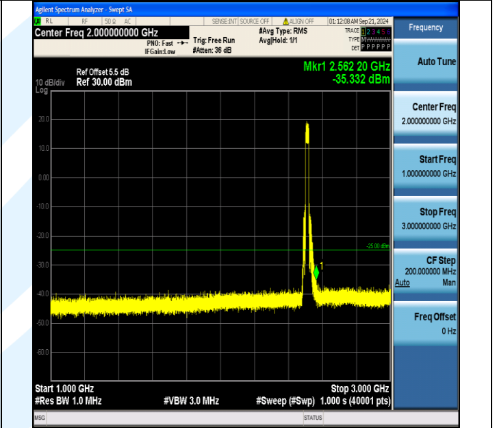
Band7_20MHz_16QAM_20850_100RB#0_1000~3000_1000~3000
