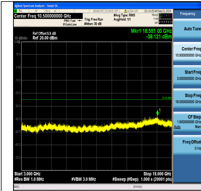
Band7_20MHz_16QAM_21100_1RB#99_3000~18000_3000~18000
