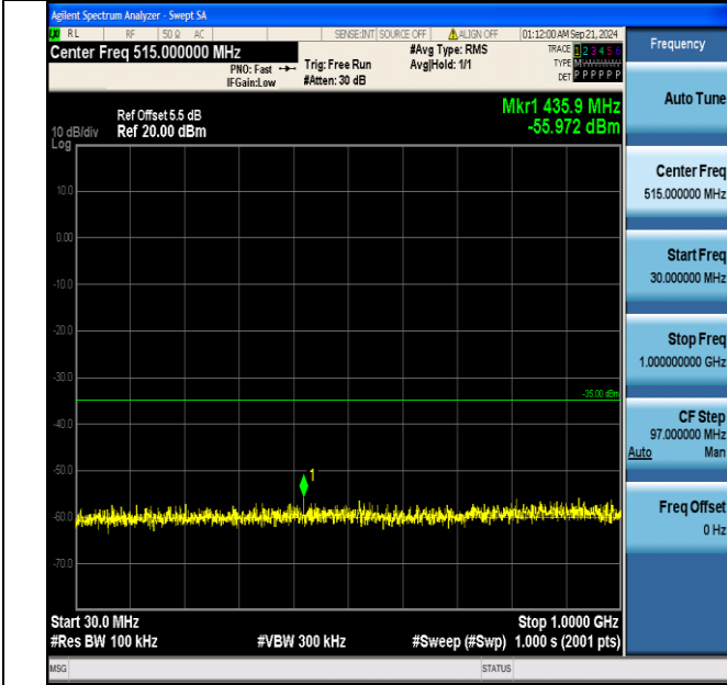
Band7_20MHz_16QAM_20850_100RB#0_30~1000_30~1000
