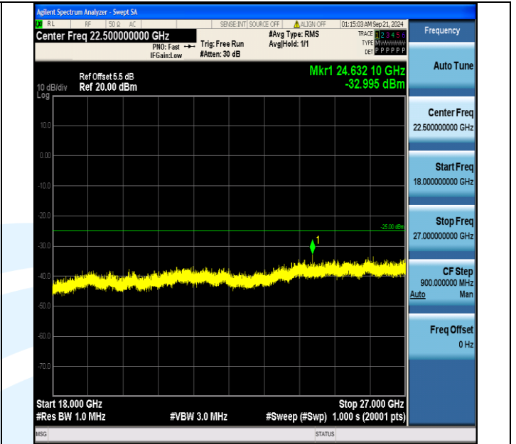
Band7_20MHz_QPSK_21100_100RB#0_18000~27000_18000~27000
