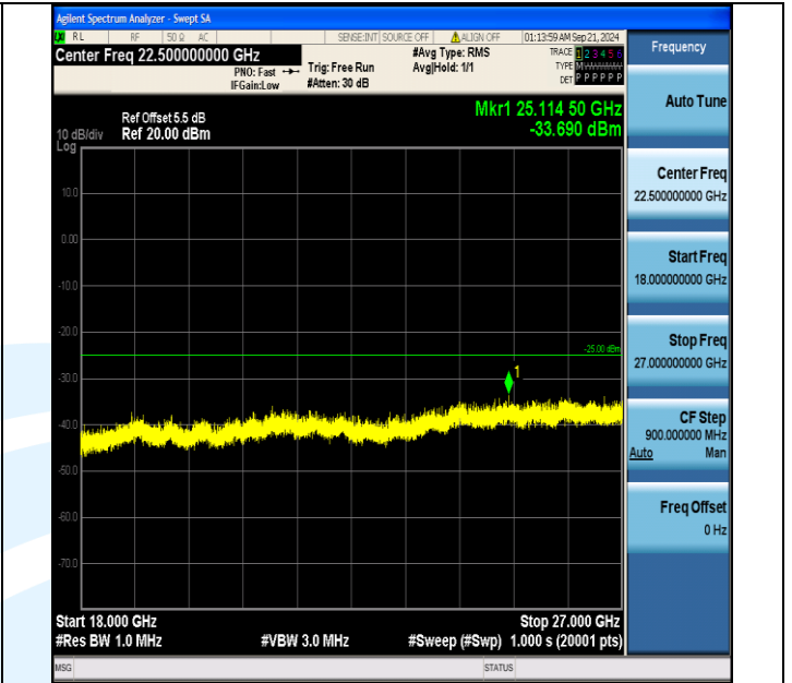
Band7_20MHz_QPSK_21100_1RB#99_18000~27000_18000~27000
