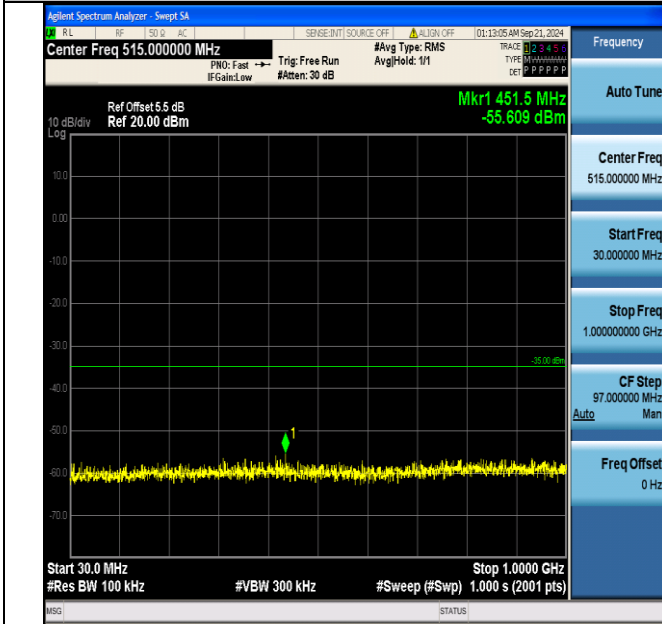
Band7_20MHz_16QAM_21100_1RB#0_30~1000_30~1000
