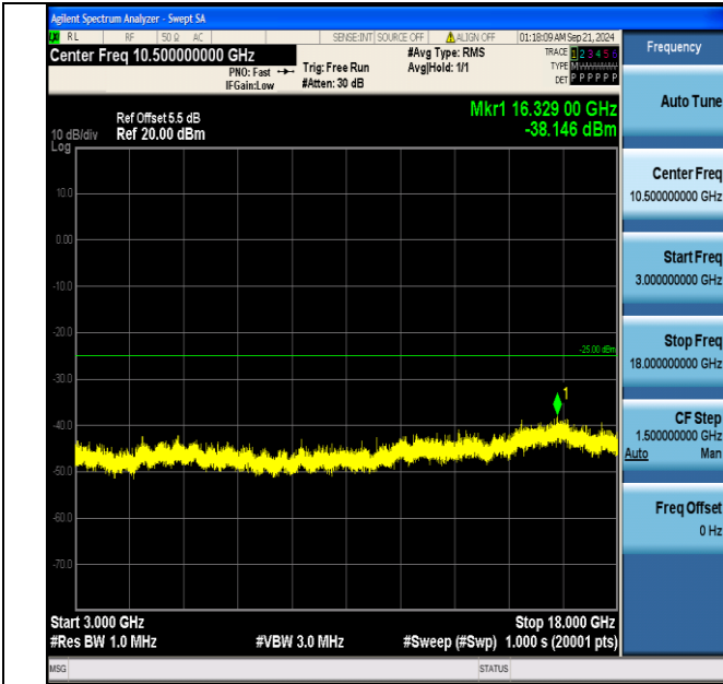
Band7_20MHz_QPSK_21350_100RB#0_3000~18000_3000~18000
