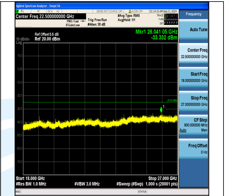
Band7_20MHz_16QAM_21100_1RB#99_18000~27000_18000~27000
