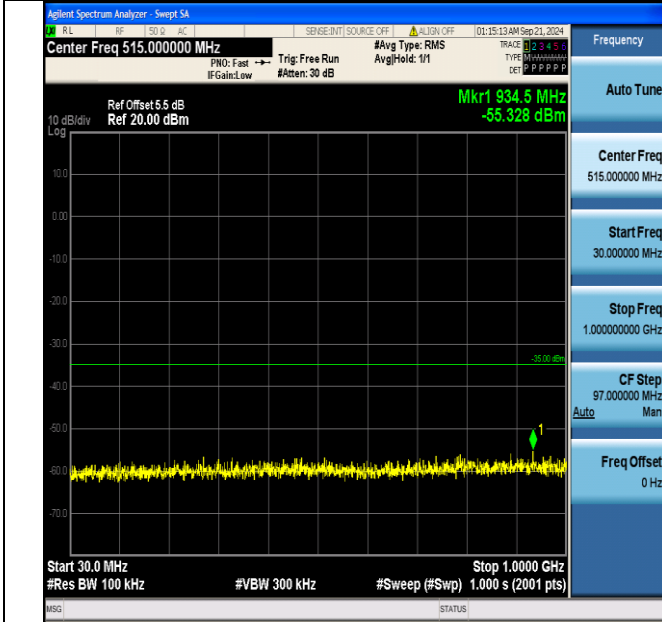
Band7_20MHz_16QAM_21100_100RB#0_30~1000_30~1000
