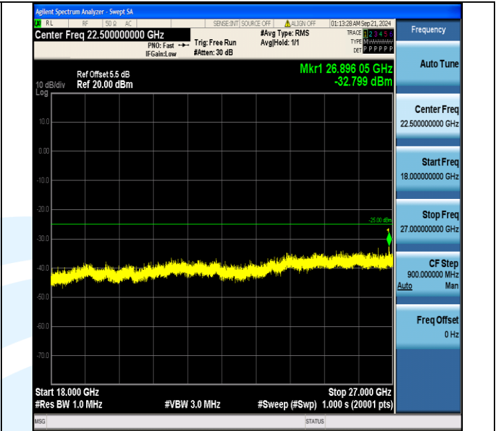
Band7_20MHz_16QAM_21100_1RB#0_18000~27000_18000~27000
