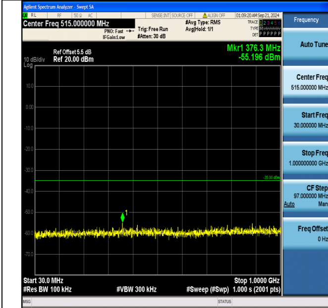
Band7_20MHz_QPSK_20850_1RB#0_30~1000_30~1000
