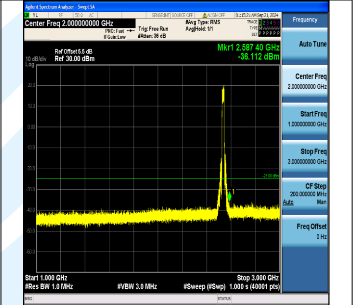
Band7_20MHz_16QAM_21100_100RB#0_1000~3000_1000~3000
