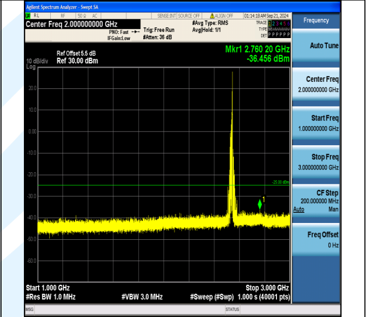
Band7_20MHz_16QAM_21100_1RB#99_1000~3000_1000~3000
