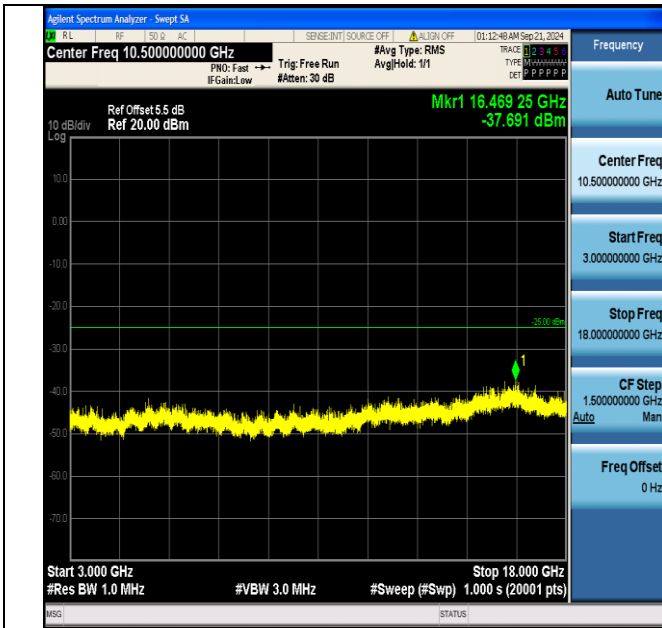
Band7_20MHz_QPSK_21100_1RB#0_3000~18000_3000~18000
