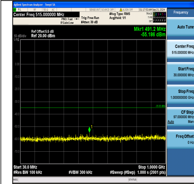
Band7_20MHz_QPSK_21350_100RB#0_30~1000_30~1000
